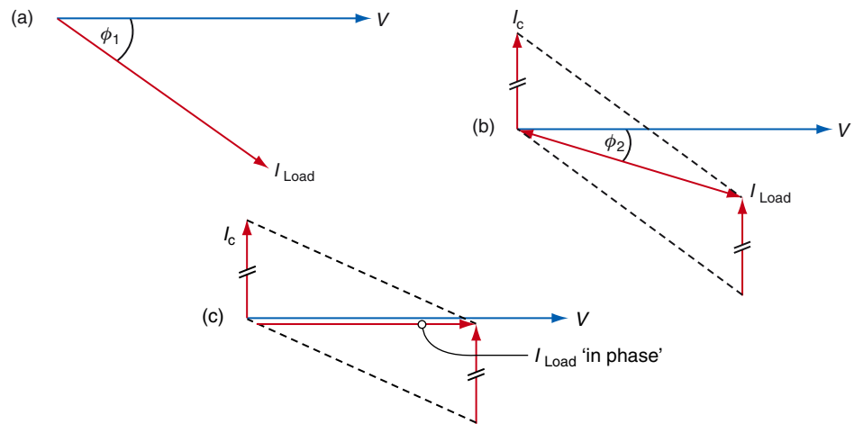
Figure 2.41 Power factor improvement using capacitors.
