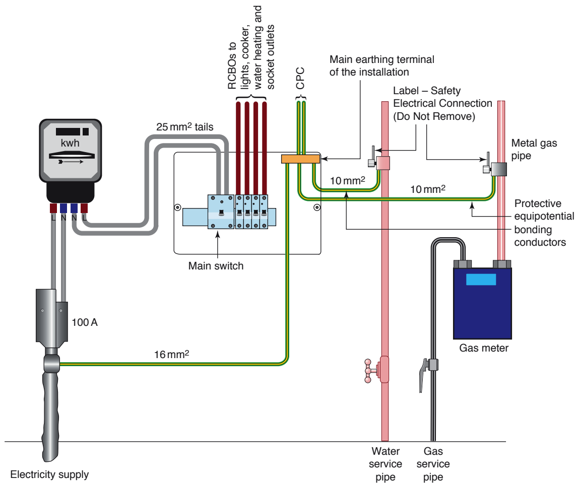
Figure 4.31 Cable sheath earth supplies (TN-S system): showing earthing and main protective bonding arrangements.
