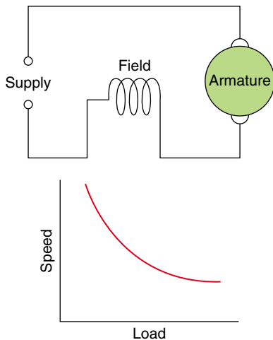
Figure 2.47 Series motor connections and characteristics.
