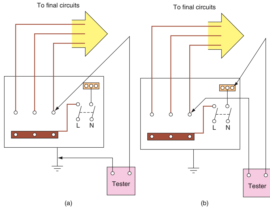
Figure 4.36 Insulation resistance test.
