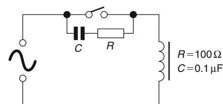
Figure 3.70 A simple noise suppressor.
