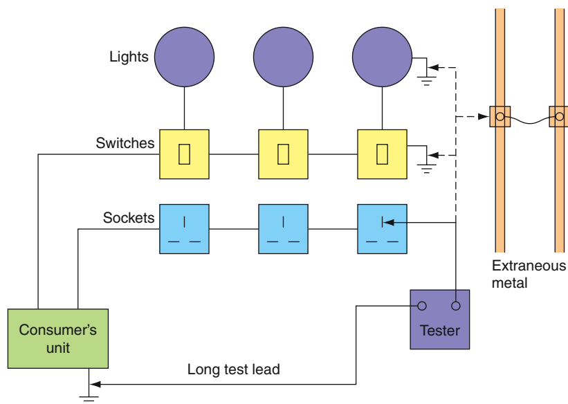
Figure 4.32 Testing continuity of protective conductors.
