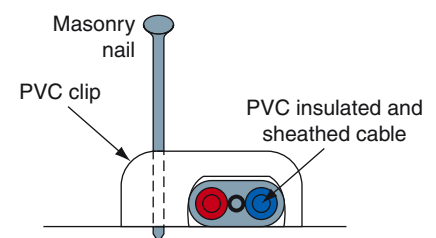
Figure 3.64 PVC insulated and sheathed cable clip.
