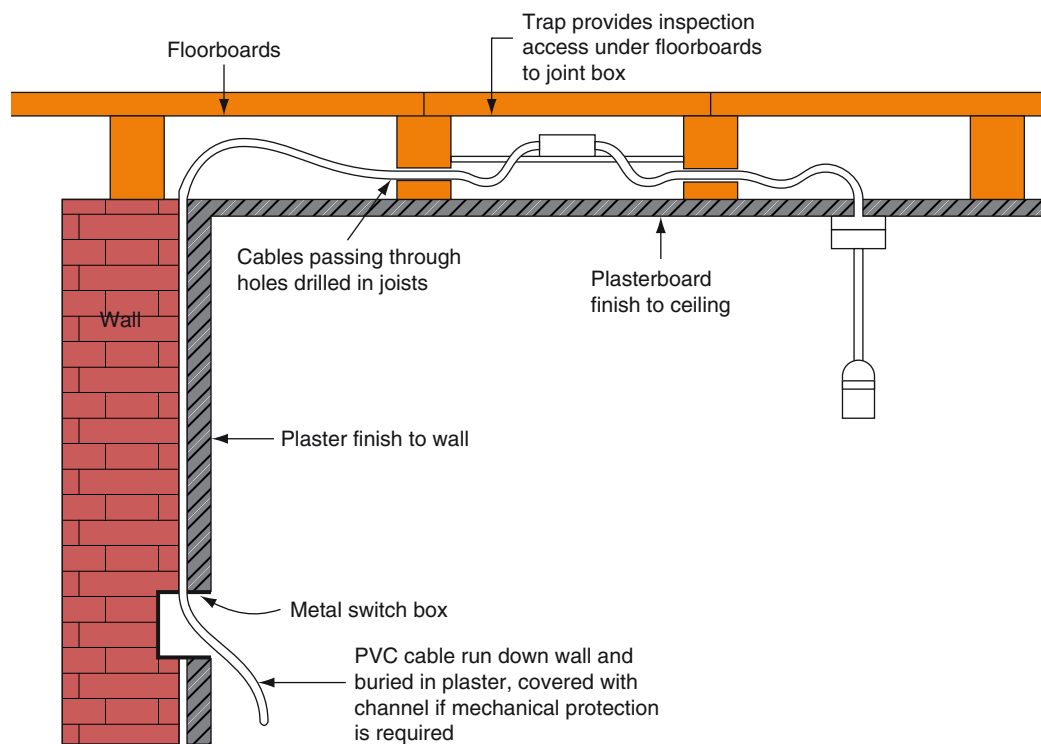
Figure 3.44 A concealed PVC sheathed wiring system.
