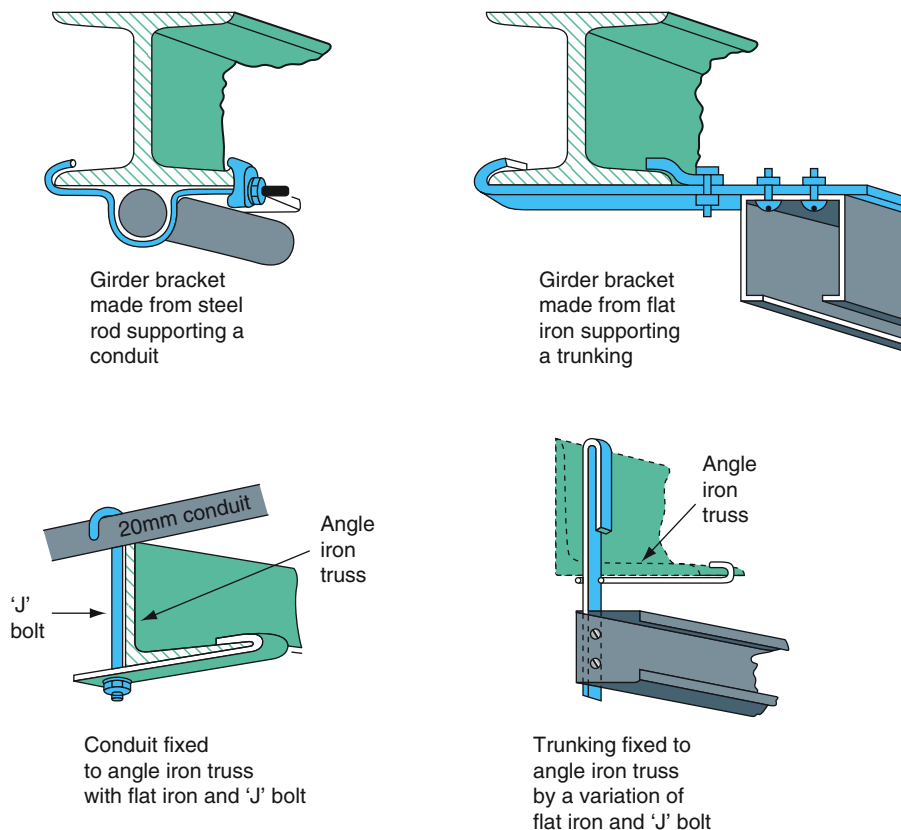
Figure 3.63 Bracket supports for conduits and trunking.
