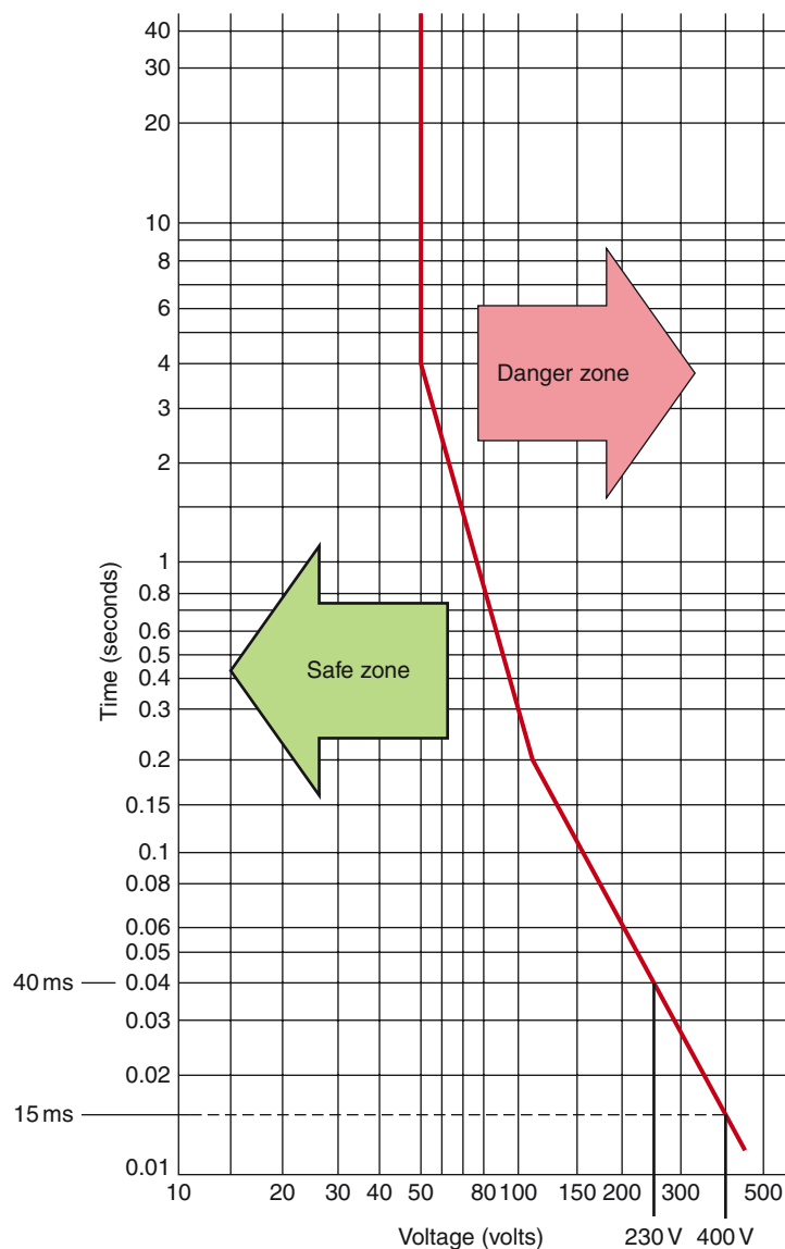
Figure 3.8 Touch voltage curve.
