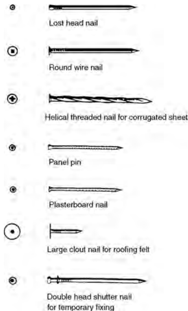
17.2 Standard nails.
