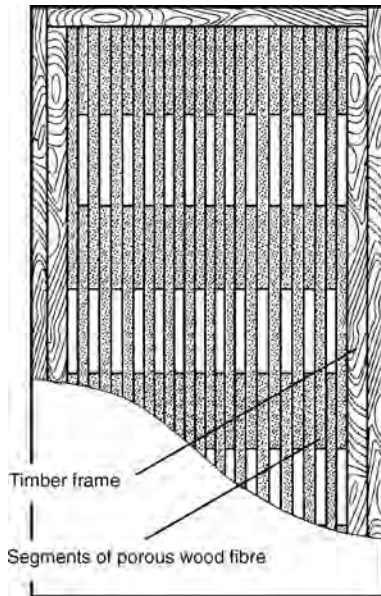
16.6 A flush door.
