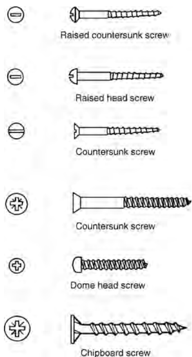
17.3 Standard wood screws.
