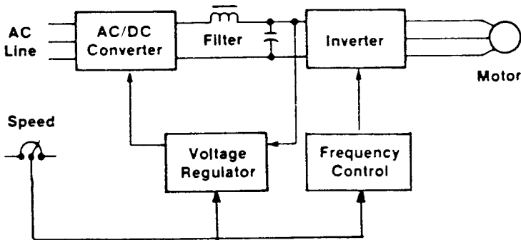
Figure 2.16. Mechanical Speed Control (Courtesy Dynamatic)
