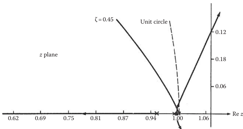
FIGURE 18.22 Enlargement of the 1 + j0 area of the root-locus plot of Figure 18.21 ( T = 0.01 s). (From Houpis, C.H. and Lamont, G.B., Digital Control Systems, Theory, Hardware, Software , 2nd edn., McGraw-Hill, New York, 1992. With permission.)
