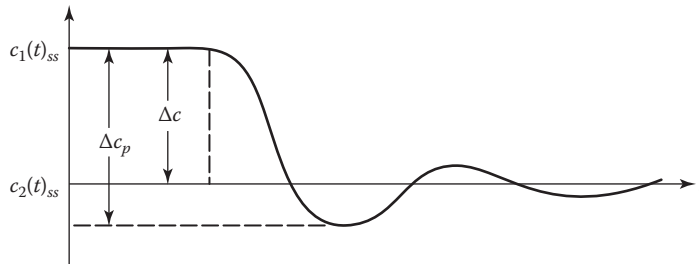
FIGURE 6.10 Underdamped transient.
