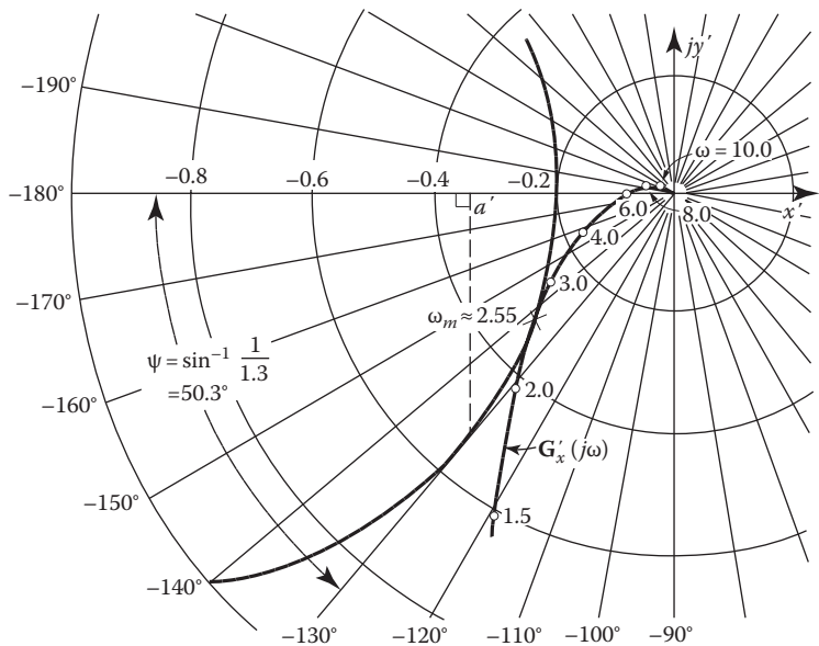
FIGURE 12.18 Gain adjustment using the procedure outlined in Section 12.7 for G'_x(j\omega) = 1/j\omega(1 + j0.25\omega)(1 + j0.1\omega) .
