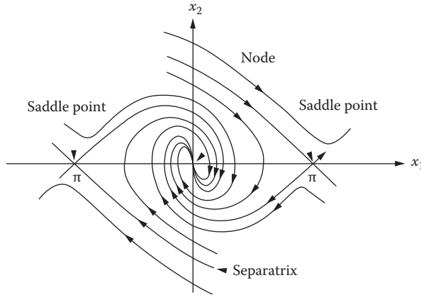
FIGURE 17.12 Phase portrait for Equation 17.34.
