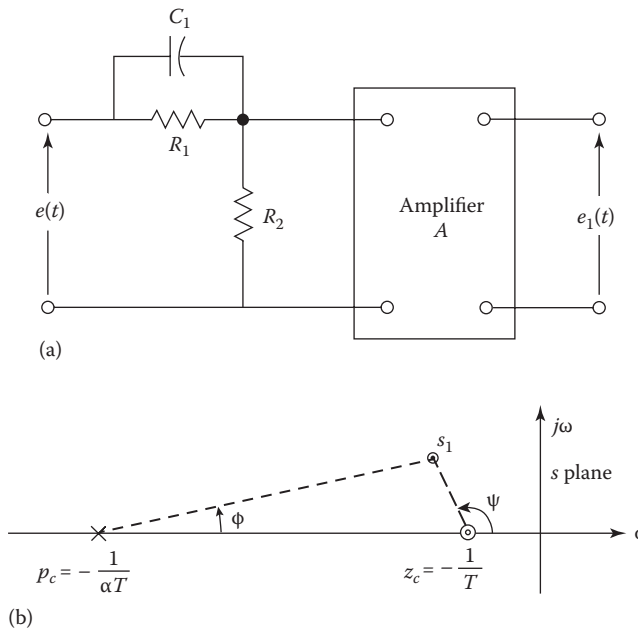
FIGURE 13.16 (a) Derivative or lead compensator. (b) Location of pole and zero of a lead compensator.
