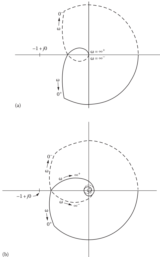
FIGURE 11.33 Complete polar plots of (a) Equation 11.66 and (b) Equation 11.67.
