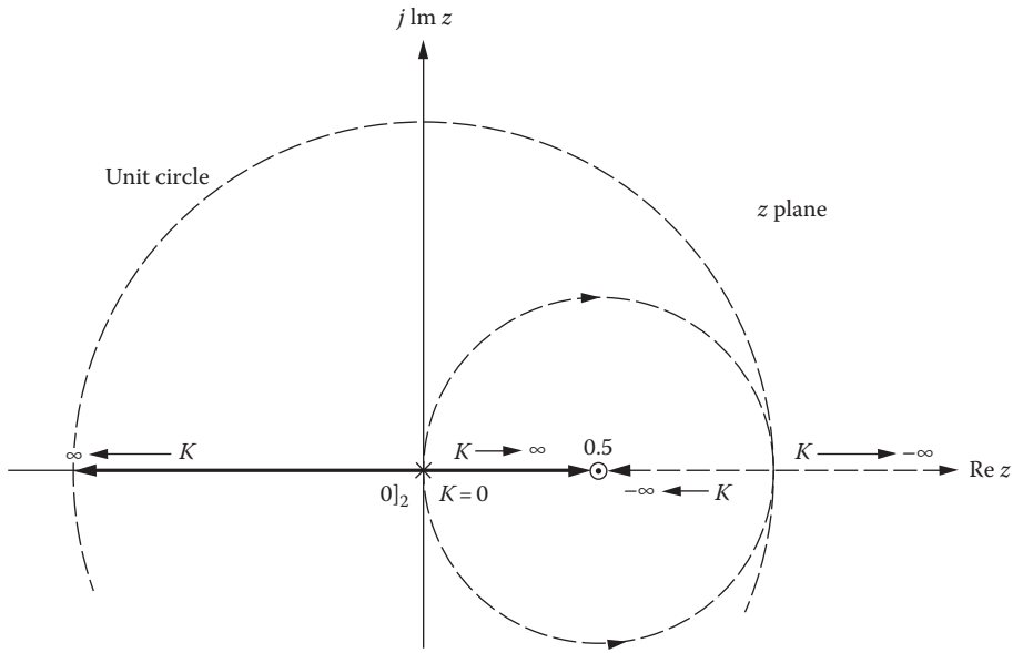
FIGURE 18.19 Root-locus plot of Example 18.8. (From Houpis, C.H. and Lamont, G.B., Digital Control Systems, Theory, Hardware, Software , 2nd edn., McGraw-Hill, New York, 1992. With permission.)
