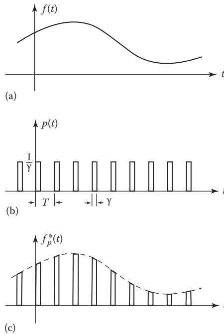
FIGURE 18.3 (a) Continuous function f(t) ; (b) sampling train p(t) ; (c) sampled function f_p^*(t) .
