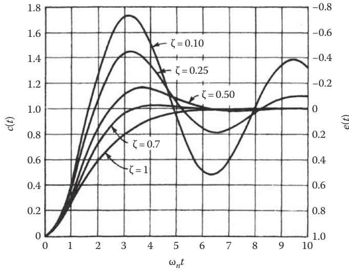
FIGURE 6.6 Simple second-order transients.
