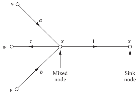
FIGURE 8.22 Mixed and sink nodes for a variable.
