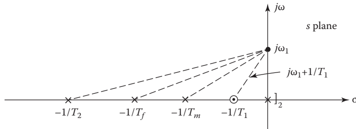
FIGURE 11.18 Pole-zero diagram for G_0(s) = \frac{K'_2 T_1}{T_f T_m T_2} \frac{s + 1/T_1}{s^2 (s + 1/T_f)(s + 1/T_m)(s + 1/T_2)} .
