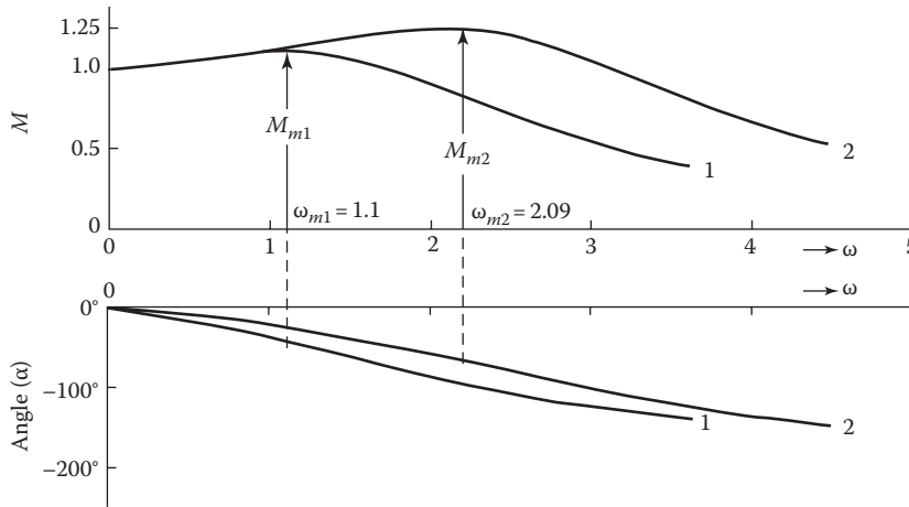
FIGURE 12.24 Control ratio versus frequency obtained from the Lm-angle diagram of Figure 12.23.
