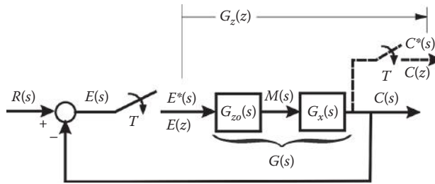
FIGURE 18.14 The uncompensated S-D control system.
