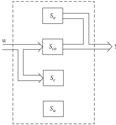
FIGURE 16.1 The four possible subdivisions of a system.
