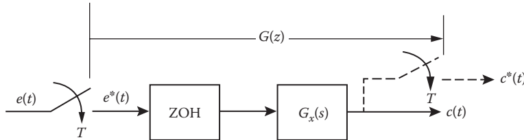
FIGURE 19.2 An open-loop sampled-data system.
