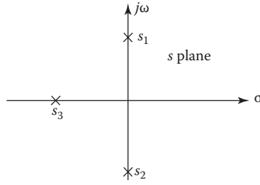
FIGURE 7.4 Poles of F(s) containing imaginary conjugate poles in the s plane.
