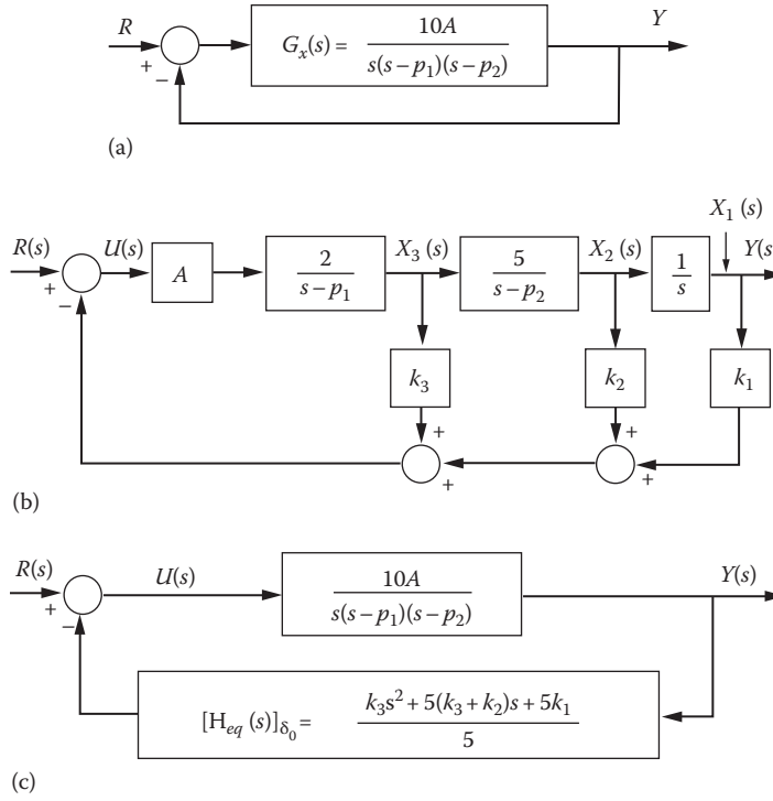
FIGURE 17.5 Control: (a) unity feedback; (b) state feedback; (c) state feedback, H -equivalent. The nominal values are p_1 = -1 , p_2 = -5 and A = 10 .
