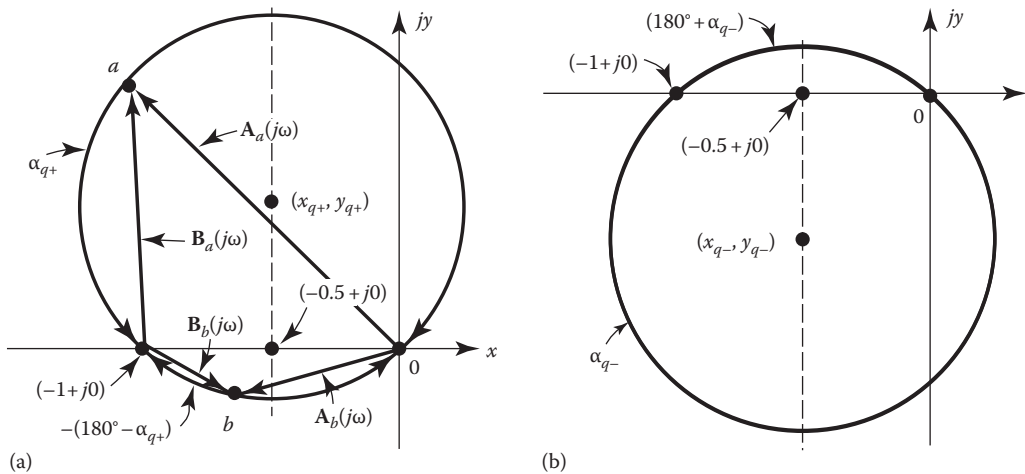
FIGURE 12.11 Arcs of constant \alpha . (a) Arcs for \alpha = -310^\circ and -130^\circ . (b) Constant \alpha contours.
