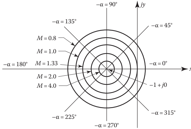
FIGURE 12.16 Typical M and \alpha contours on the inverse polar plane for unity feedback.
