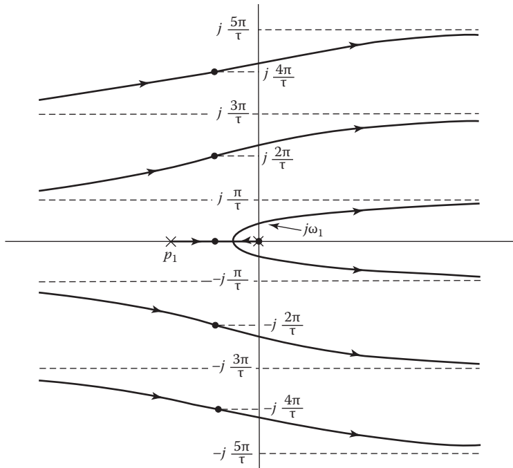
FIGURE 10.28 Root locus for G(s)H(s) = \frac{Ke^{-\tau s}}{s(s - p_1)} .
