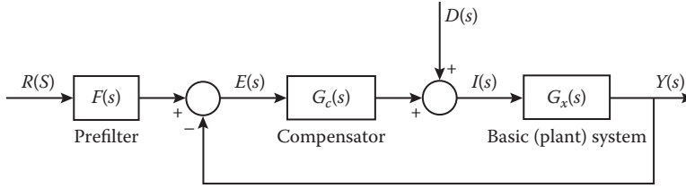
FIGURE 15.1 A MISO control system.
