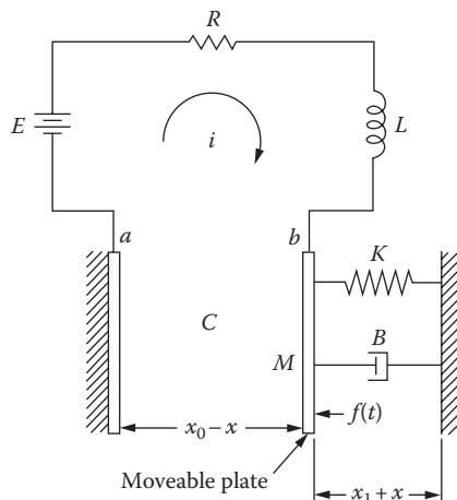
FIGURE 5.29 Electromechanical system with capacitive coupling.
