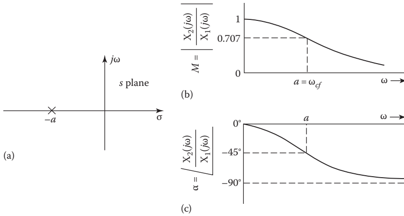
FIGURE 7.9 (a) Pole location of Equation 7.78; (b) M versus \omega ; (c) \alpha versus \omega .
