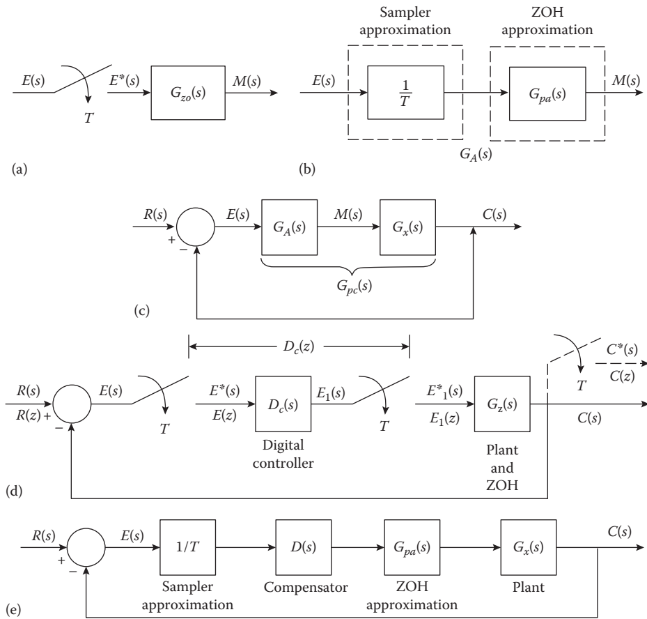
FIGURE 19.14 The PCT equivalent of Figure 19.1. (a) This corresponds to the forward loop of Figure 19.1 excluding the plant G_x(s) . (b) A representation of a sampler and a ZOH. (c) A PCT representation of Figure 19.1. (d) A MISO digital control system representation of Figure 19.14c. (e) A simplified block diagram of Figure 19.14d.
