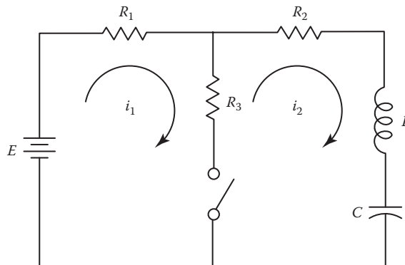
FIGURE 6.5 Electric circuit: E = 10 V, R_1 = 10 \Omega , R_2 = 15 \Omega , R_3 = 10 \Omega , L = 1 H, C = 0.01 F.
