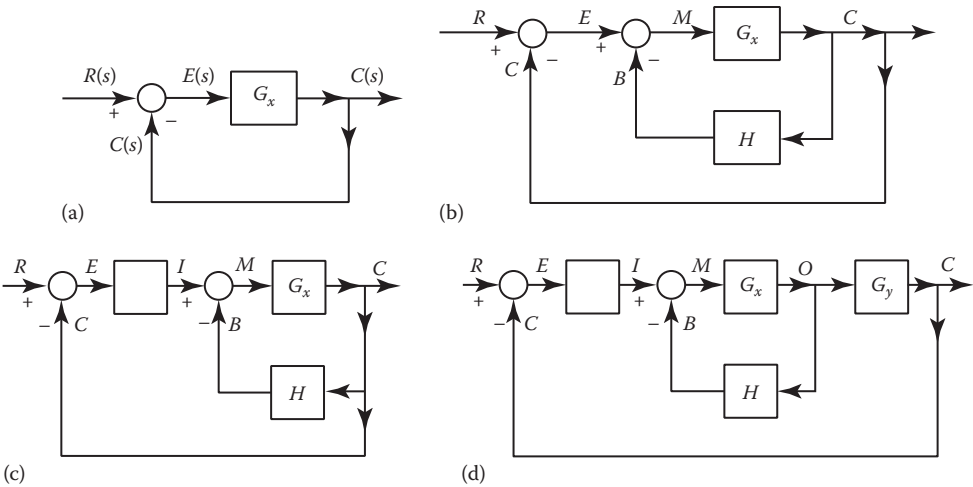
FIGURE 13.27 Various forms of feedback systems: (a) uncompensated system; (b) feedback-compensated system; (c) and (d) feedback-compensated systems with a cascade gain A or compensator G_c .
