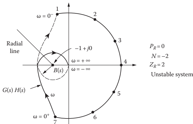
FIGURE 11.28 Polar plot of Figure 11.26b with increased gain.
