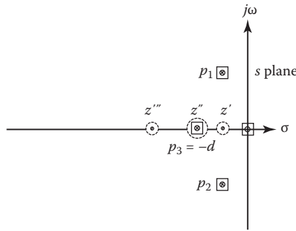
FIGURE 15.3 Pole–zero location of Y(s) for Equation 15.5, with a step input.
