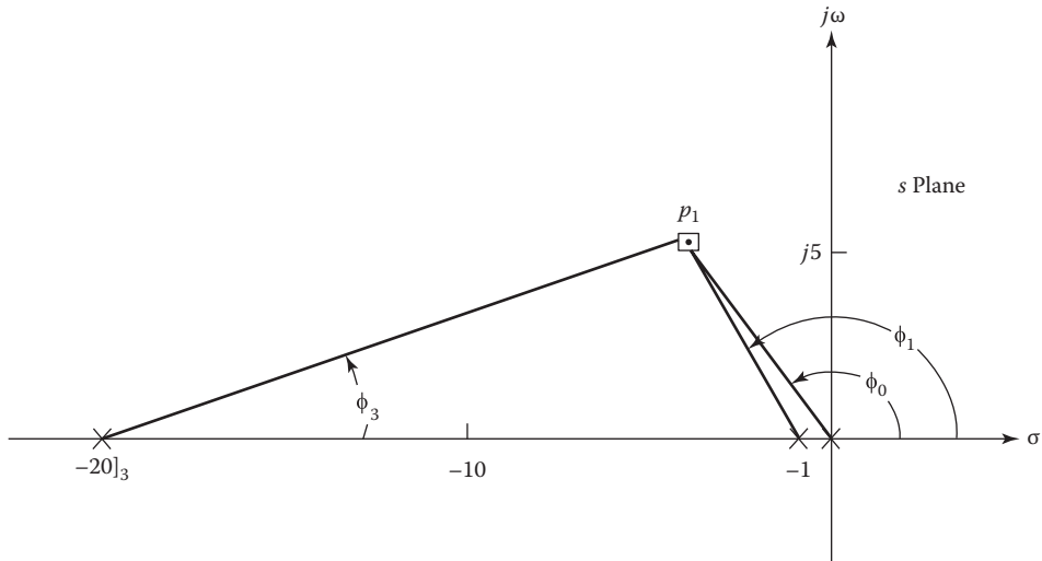
FIGURE 19.25 The plot of the poles of Equation 19.104.
