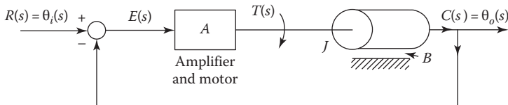
FIGURE 10.1 A position-control system.
