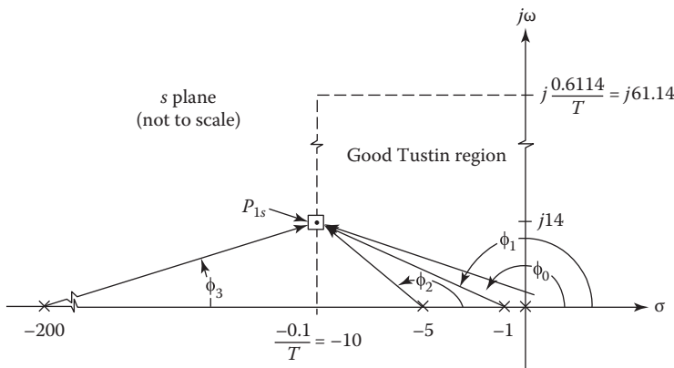
FIGURE 19.20 Plot of known poles of G(s) and P_{1_s} .
