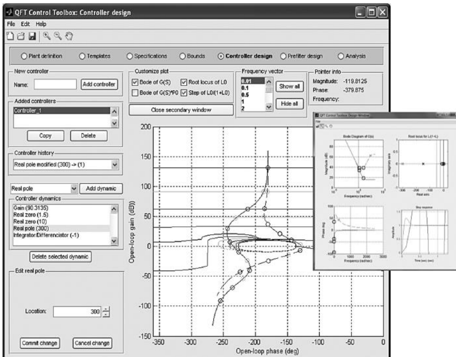
FIGURE 3.4 A novel CAD toolbox in MATLAB® for QFT controller design (the QFTCT). (From Garcia-Sanz, M. and Houppis, C.H., Wind Energy Systems: Control Engineering Design , Taylor & Francis Group, Boca Raton, FL, 2012.)
