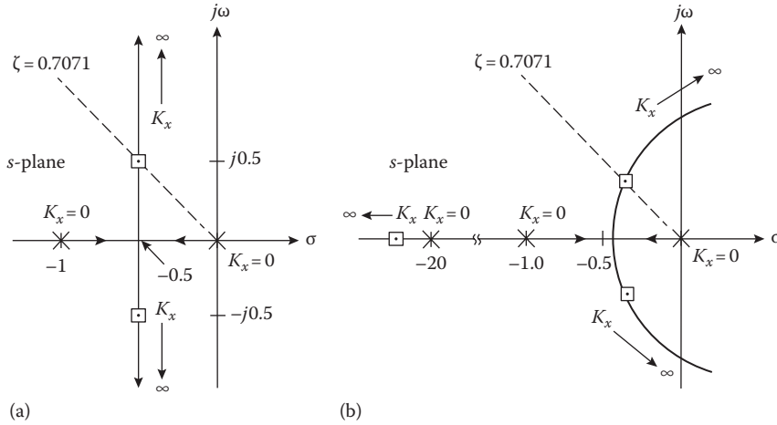
FIGURE 19.13 Root locus for (a) Case 19.1, Equation 19.27, and (b) Case 19.2, Equation 19.28.
