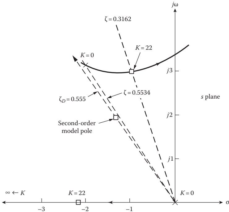
FIGURE 13.6 Root locus for Equation 13.19.
