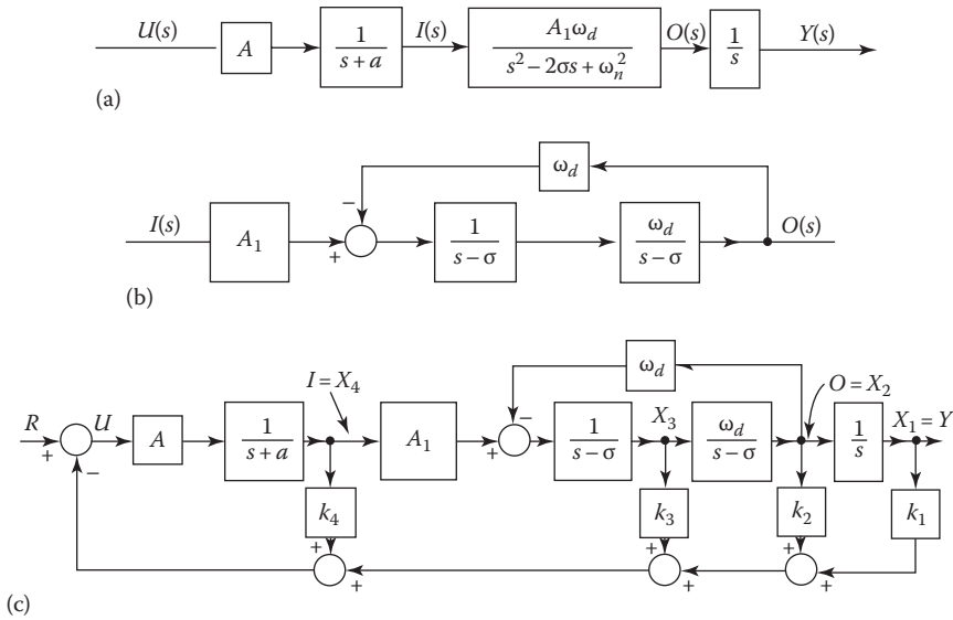
FIGURE 16.11 Representation of a plant containing complex poles. (a) A block diagram for a system containing four state variables having only two explicit state variables identified. (b) A simulation diagram. (c) A state-variable feedback compensation diagram.
