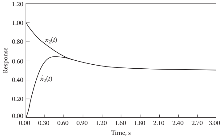
FIGURE 16.22 Plant and observer states, Equations 16.141 and 16.143.
