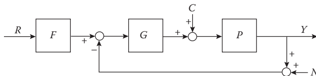
FIGURE 17.2 An example of system sensitivity analysis.
