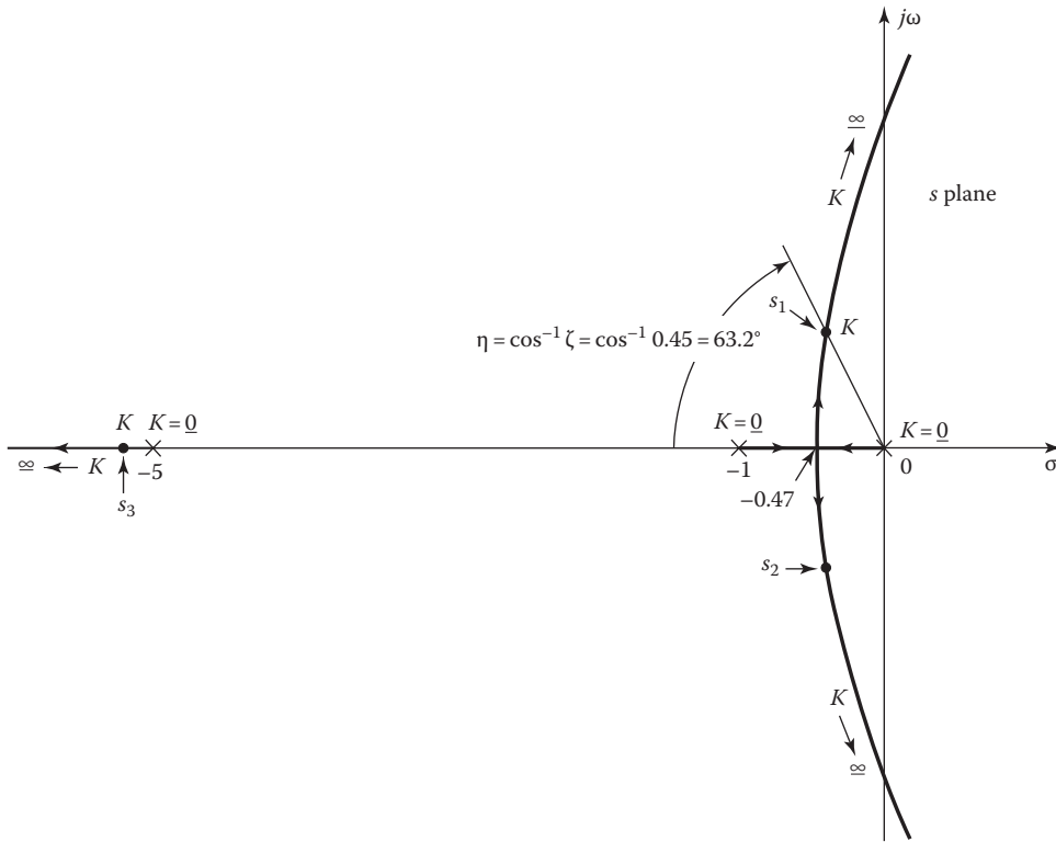
FIGURE 13.10 Root locus of G_x(s) = K/s(s+1)(s+5) .
