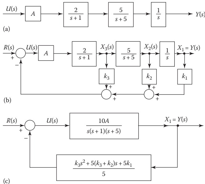
FIGURE 16.9 A state-variable-feedback system, all-pole plant: (a) plant, (b) state-variable feedback, and (c) H_{eq}(s) .
