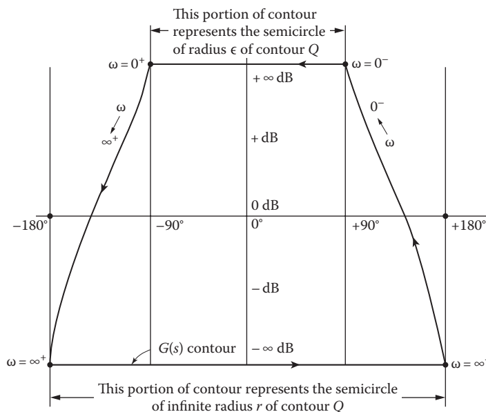
FIGURE 11.36 The L_m -angle contour for the m.p. system of Equation 11.71.
