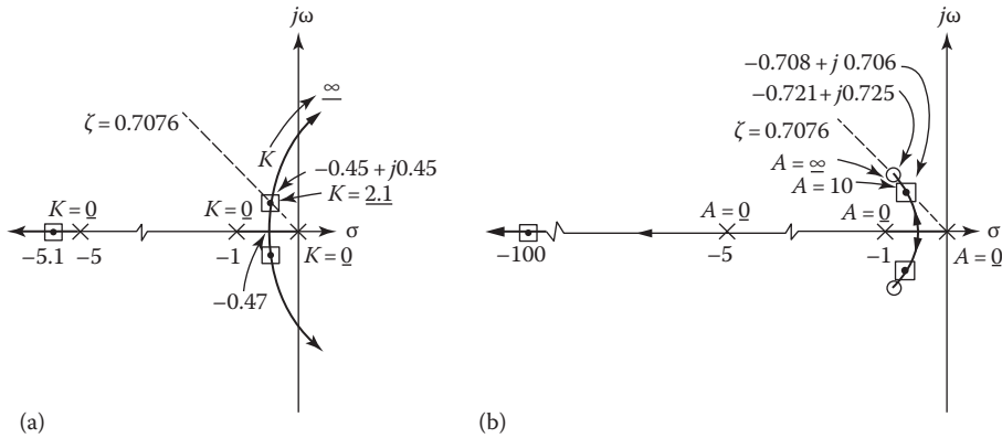
FIGURE 16.10 Root-locus diagrams for (a) basic unity-feedback and (b) state-variable control systems.
