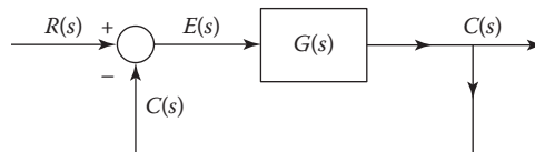
FIGURE 9.4 Unity-feedback control system.
