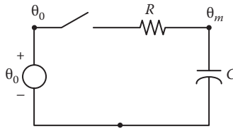
FIGURE 5.20 Simple network representation of a thermometer.
