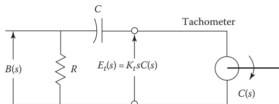
FIGURE 13.36 Tachometer and RC feedback network.
