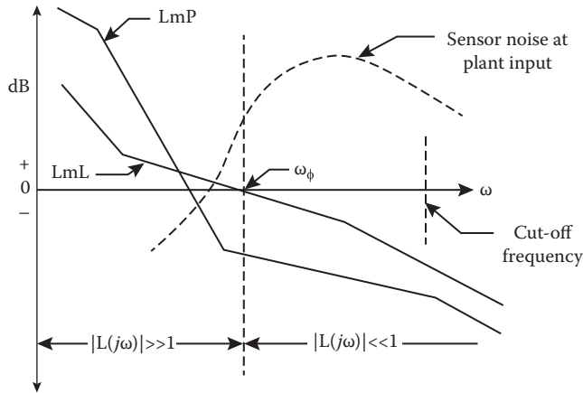
FIGURE 17.4 Bandwidth characteristics of Figure 17.2.
