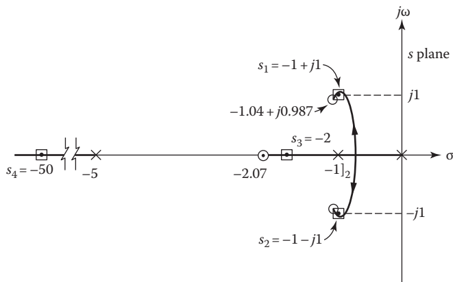
FIGURE 16.18 The root locus for Equation 16.126.
