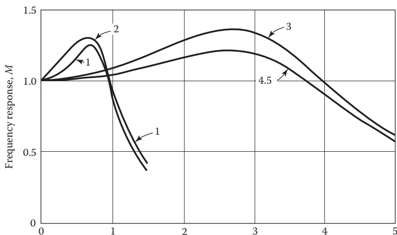
FIGURE 13.24 Frequency response for systems of Table 13.1: (1) original basic system; (2) lag compensated; (3) lead compensated, zero at -1.5 ; (4) lead compensated, zero at -1.0 ; and (5) lag–lead compensated.
