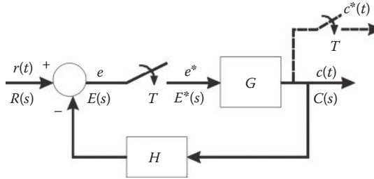
FIGURE 18.2 Block diagram of an S-D control system involving the sampling of the actuating signal.
