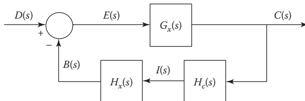
FIGURE 19.26 A control system with a disturbance input.
