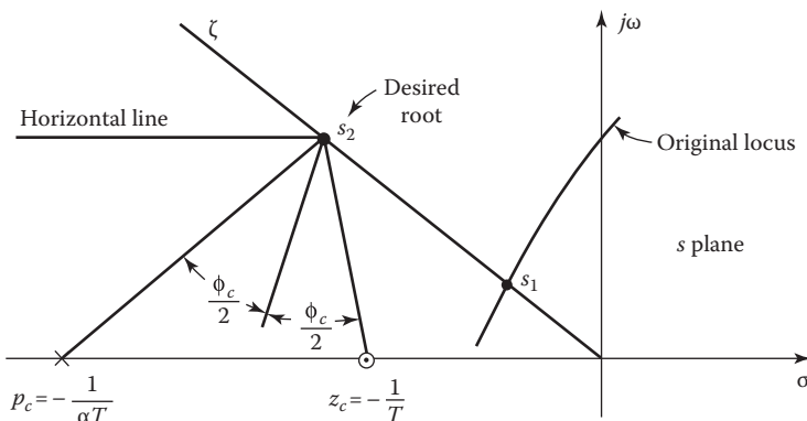
FIGURE 13.21 Graphical construction for locating the pole and zero of a simple lead compensator.
