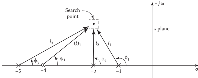
FIGURE 10.7 Construction of the root locus.
