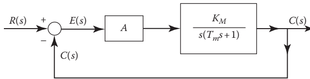
FIGURE 12.3 A position-control system.
