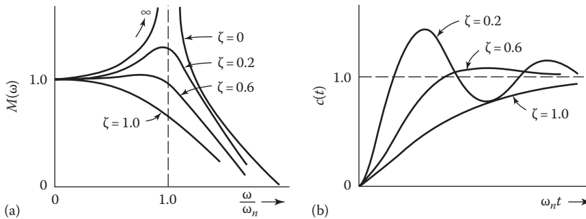
FIGURE 12.4 (a) Plots of M versus \omega/\omega_n for a simple second-order system. (b) Corresponding time plots for a step input.
