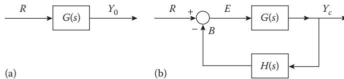
FIGURE 17.1 Control systems: (a) open loop; (b) closed loop.
