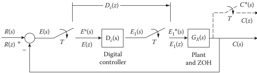
FIGURE 19.1 A compensated digital control system.
