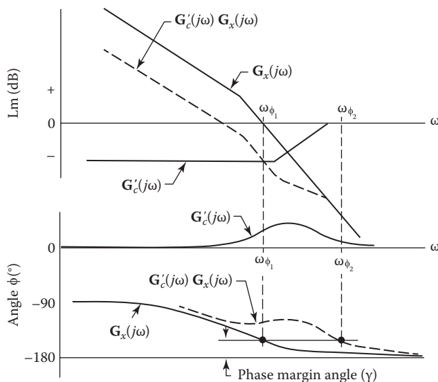
FIGURE 14.11 Original and lead-compensated Lm and phase-angle plots.
