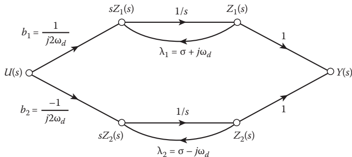
FIGURE 8.33 Simulation diagram for Equations 8.129 and 8.130.
