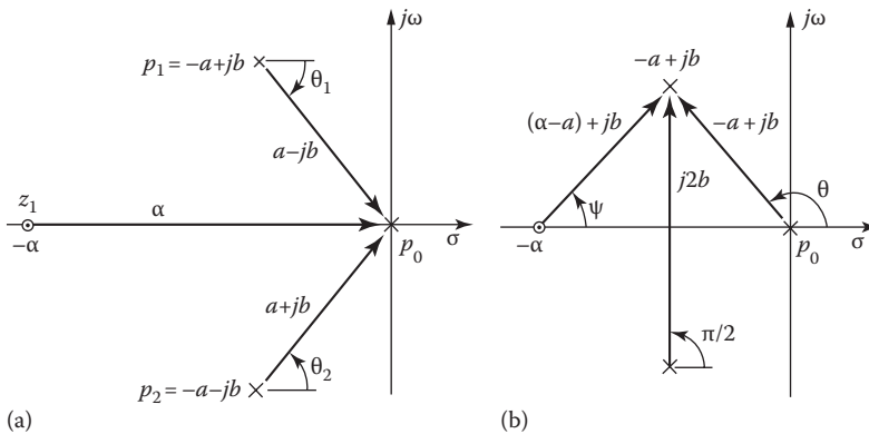
FIGURE 7.7 Directed line segments for evaluating (a) A_0 of Equation 7.70 and (b) A_1 of Equation 7.71.
