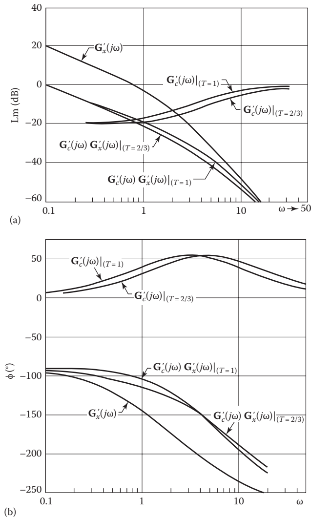
FIGURE 14.13 (a) L_m and (b) phase-angle diagrams of G'_x(j\omega) = \frac{1}{0.1(1+j\omega T)} G'_c(j\omega)G'_x(j\omega) = \frac{1}{j\omega(1+j\omega)(1+j0.2\omega)(1+j0.1\omega T)} .
