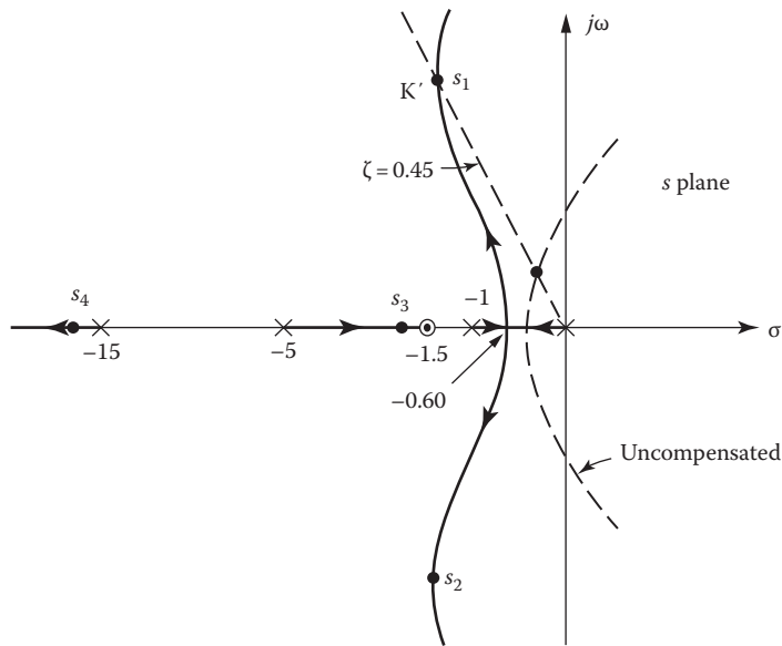
FIGURE 13.19 Root locus of G(s) = AK(s + 1.5)/(s(s + 1)(s + 5)(s + 15)) .
