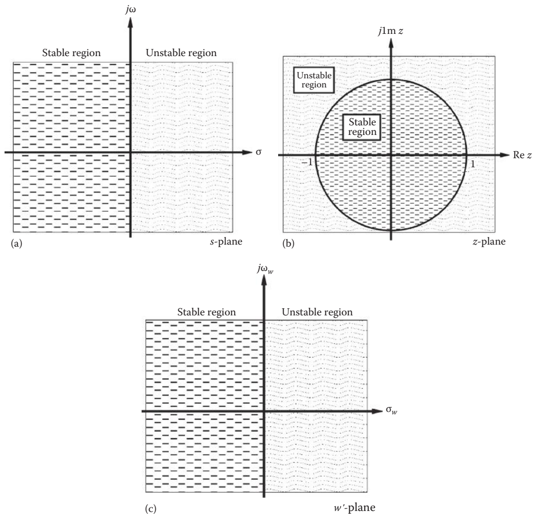
FIGURE 19.6 Mapping of (a) the s -plane into (b) the z -plane into (c) the w' -plane.
