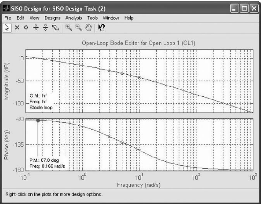
FIGURE C.8 Bode diagram SISOTOOL window.
