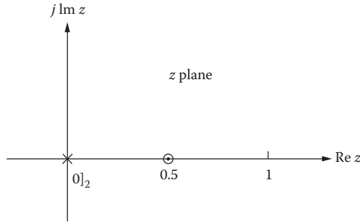
FIGURE 18.18 Poles and zero of Equation 18.101. (From Houpis, C.H. and Lamont, G.B., Digital Control Systems, Theory, Hardware, Software , 2nd edn., McGraw-Hill, New York, 1992. With permission.)
