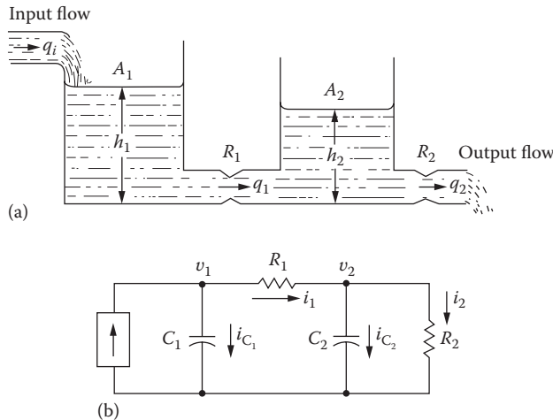
FIGURE 5.23 (a) A liquid level system and (b) its equivalent electrical analog diagram.
