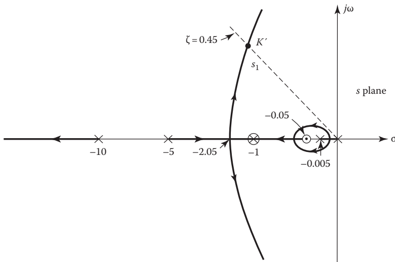
FIGURE 13.23 Root locus of G(s) = K'(s+0.05)/(s(s+0.005)(s+5)(s+10)) .
