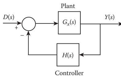
FIGURE 15.6 A simple disturbance-rejection control system.
