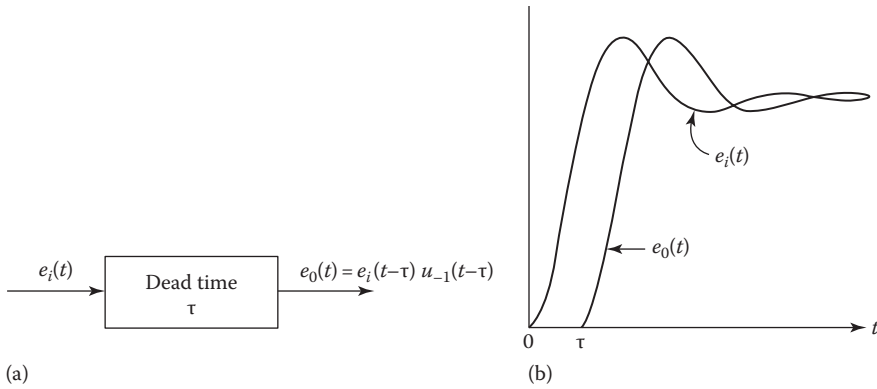
FIGURE 10.27 (a) Transport lag \tau ; (b) time characteristic.
