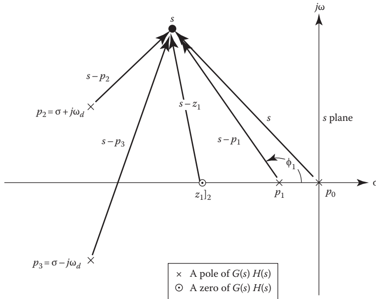
FIGURE 10.6 Pole-zero diagram for Equation 10.27.
