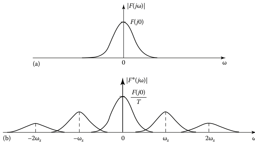
FIGURE 18.4 Frequency spectra for (a) a continuous function f(t) and (b) a pulse-sampled function f_p^*(t) .
