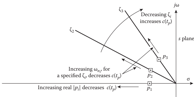
FIGURE 15.11 Effects on the peak overshoot to a disturbance input due to changes in the parameters \zeta_i and \omega_{n_i} of complex poles and the values of the real poles of the control ratio.
