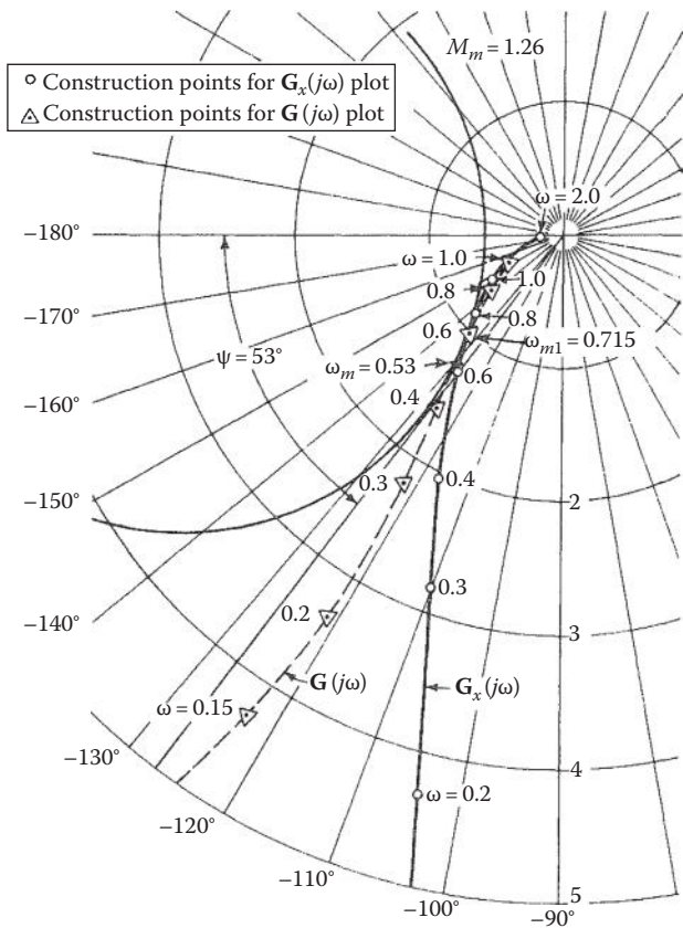
FIGURE 14.9 Polar plots of a Type 1 control system, with and without lag compensation.
