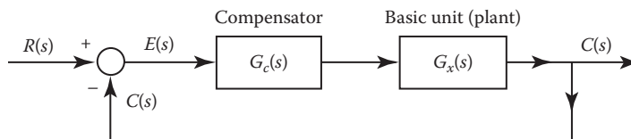
FIGURE 14.1 Cascade compensation.
