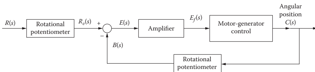
FIGURE 8.9 Position-control system.
