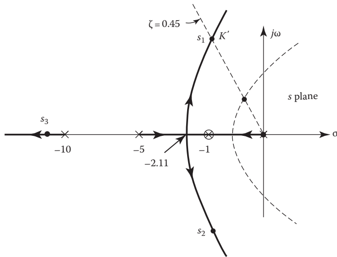
FIGURE 13.18 Root locus of G(s) = AK(s + 1)/(s(s + 1)(s + 5)(s + 10)) .
