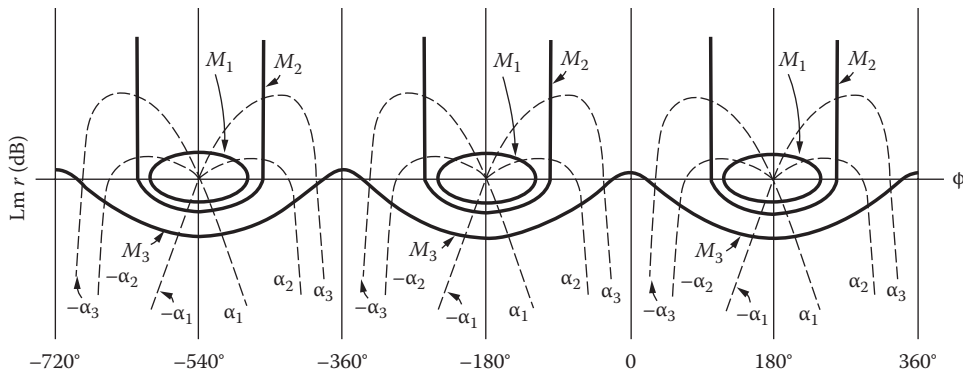
FIGURE 12.20 Constant M and \alpha curves on the Nichols chart.
