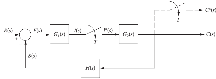
FIGURE 18.17 A nonunity-feedback S-D control system. (From Houpis, C.H. and Lamont, G.B., Digital Control Systems, Theory, Hardware, Software , 2nd edn., McGraw-Hill, New York, 1992. With permission.)
