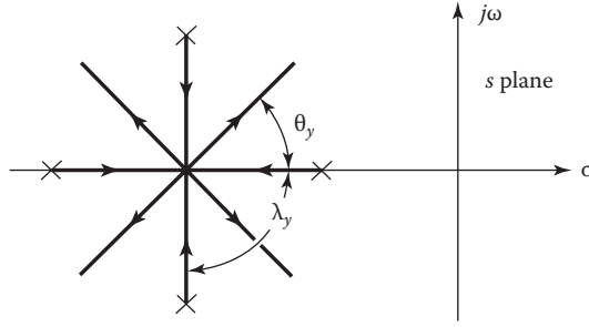
FIGURE 10.14 Root locus for G(s)H(s) = \frac{K}{(s+2)(s+4)(s^2+6s+10)} .
