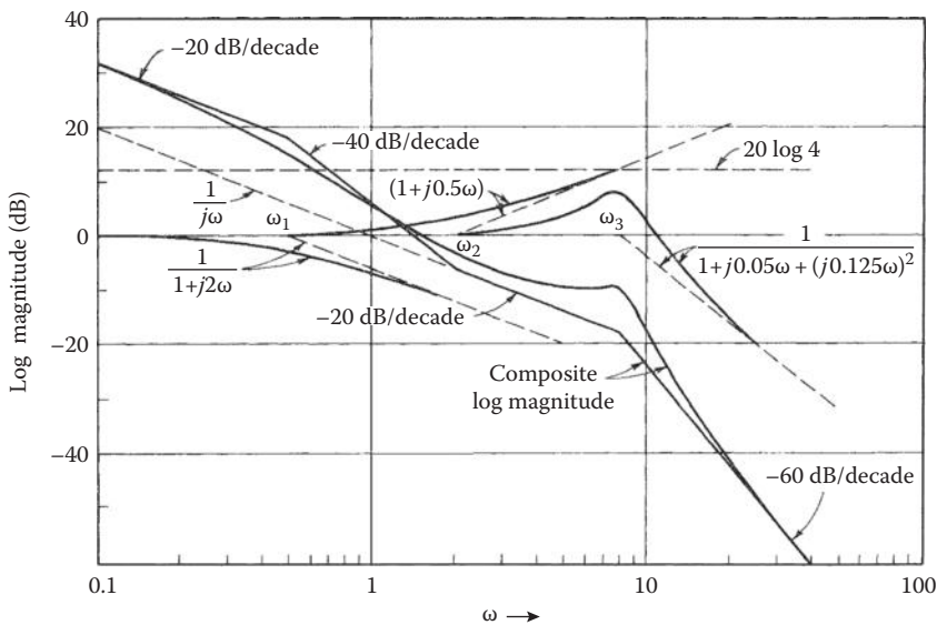
FIGURE 11.6 Lm curve for G(j\omega) = \frac{4(1 + j0.5\omega)}{j\omega(1 + j2\omega)[1 + j0.05\omega + (j0.125\omega)^2]} .
