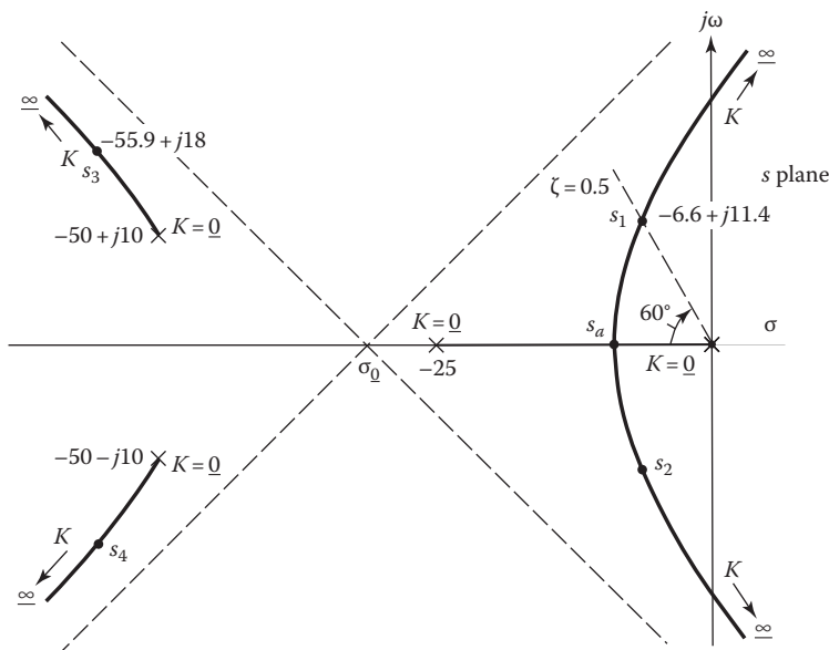
FIGURE 10.17 Determination of the departure angle.
