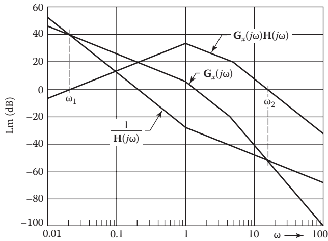
FIGURE 14.24 Lm plots of 1/\mathbf{H}(j\omega) , \mathbf{G}_x(j\omega) , and \mathbf{G}_x(j\omega)\mathbf{G}(j\omega) .
