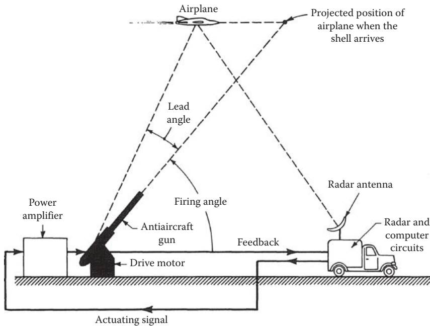
FIGURE 1.10 Anti-aircraft radar-tracking control systems.
