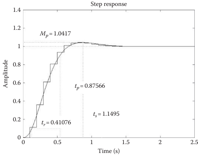
FIGURE 19.17 MATLAB® step response T = 0.1 s and FOM for Equations 19.57 and 19.60.
