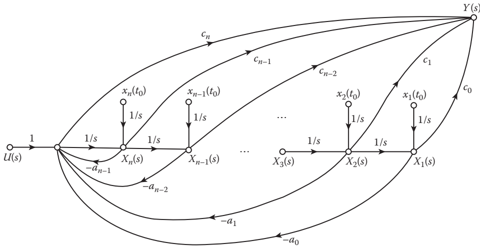
FIGURE 8.30 State diagram for Equation 8.62 using phase variables, for w = n .
