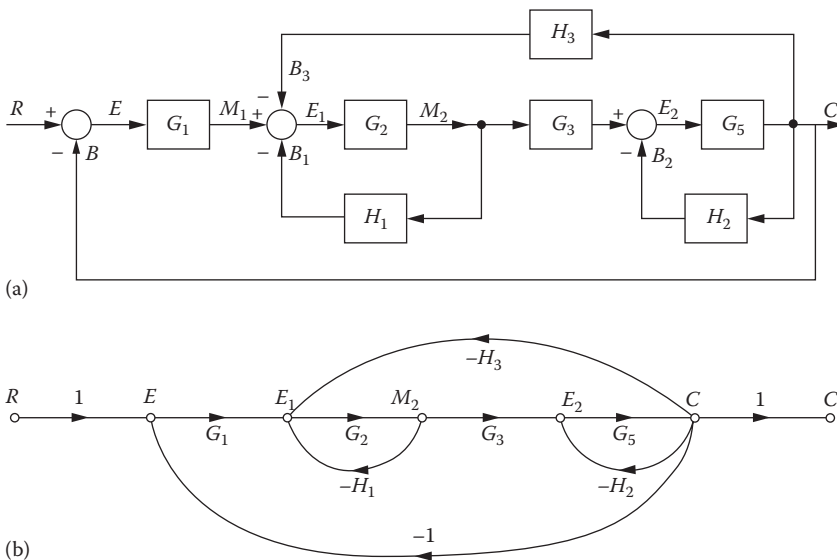
FIGURE 8.26 (a) A block diagram and (b) its SFG.
