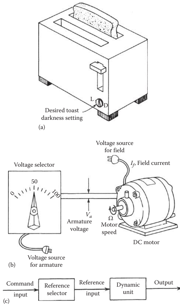
FIGURE 1.1 Open-loop control systems: (a) automatic toaster; (b) electric motor; (c) functional block diagram.
