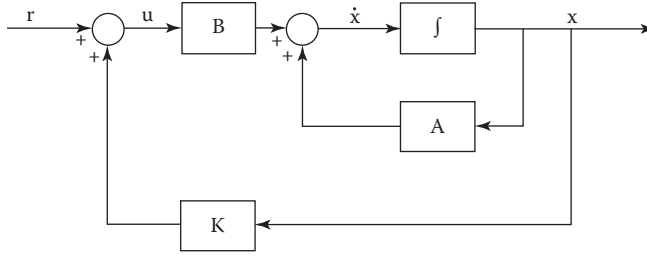
FIGURE 16.4 State-feedback-control system.
