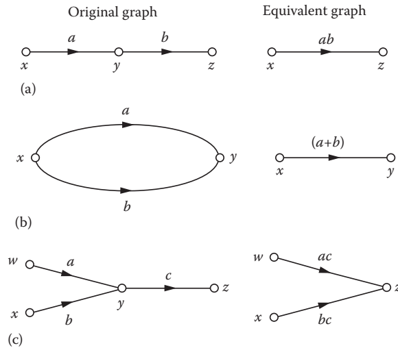
FIGURE 8.23 Flow-graph simplifications. Representation of (a) series paths, (b) parallel paths, and (c) node absorption.
