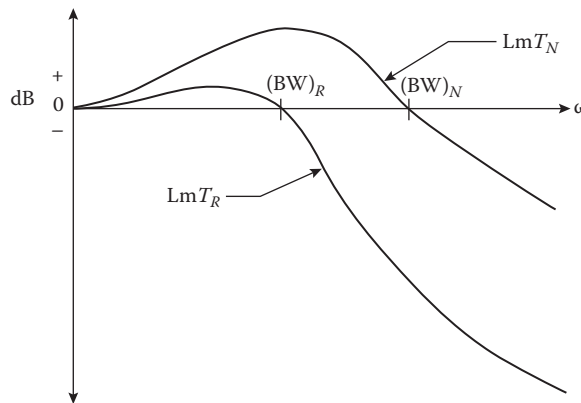
FIGURE 17.3 Frequency response characteristics for the system of Figure 17.2.
