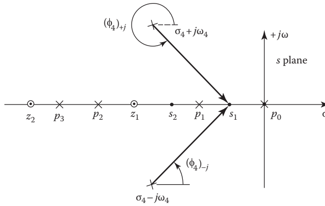
FIGURE 10.9 Determination of the real-axis locus.
