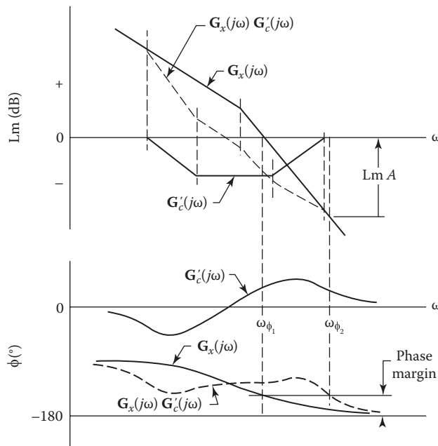
FIGURE 14.17 Original and lag-lead compensated Lm and phase-angle plots.
