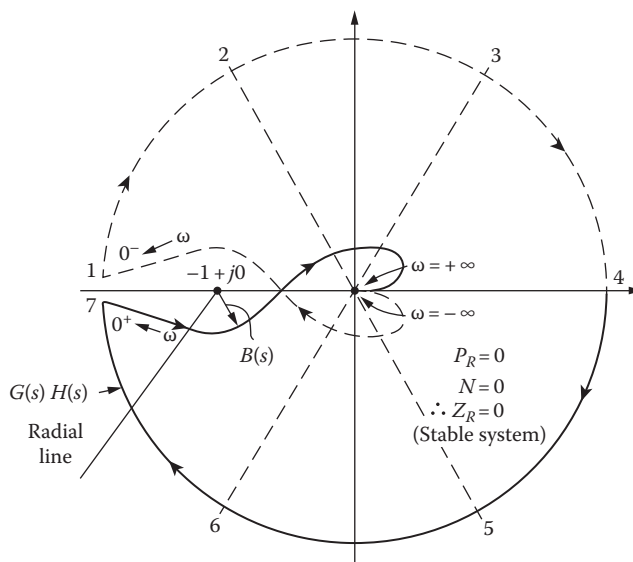
FIGURE 11.29 The complete polar plot of Equation 11.62.
