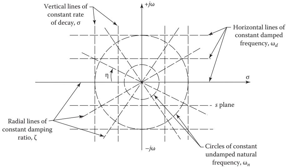
FIGURE 10.24 Constant-parameter curves on the s plane.
