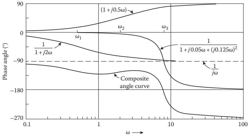
FIGURE 11.7 Phase-angle curve for G(j\omega) = \frac{4(1 + j0.5\omega)}{j\omega(1 + j2\omega)[1 + j0.05\omega + (j0.125\omega)^2]} .
