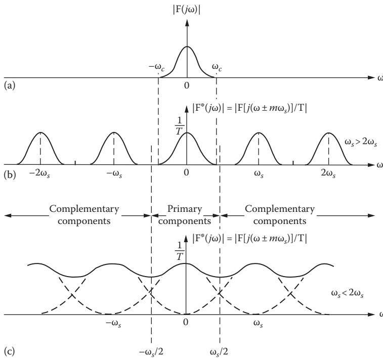
FIGURE 18.6 Frequency spectra for (a) a continuous function f(t) ; (b) an impulse-sampled function f^*(t) , when \omega_s > 2\omega_c ; (c) an impulse-sampled function f^*(t) , when \omega_s < 2\omega_s . (From Houpis, C.H. and Lamont, G.B., Digital Control Systems, Theory, Hardware, Software , 2nd edn., McGraw-Hill, New York, 1992.)
