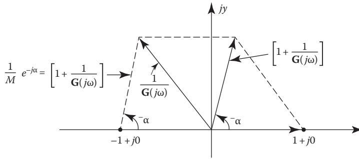
FIGURE 12.14 Representation of the quantities in Equation 12.37 with \mathbf{H}(j\omega) = 1 .
