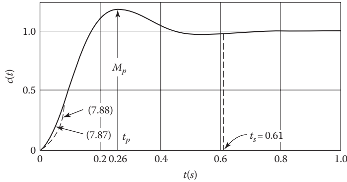
FIGURE 10.26 Plot c(t) versus t for Equations 10.87 and 10.88.
