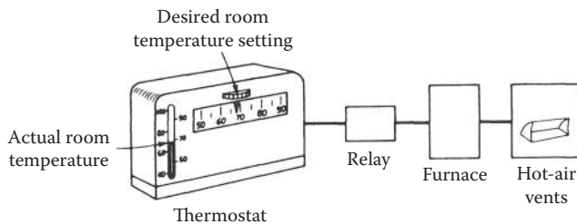
FIGURE 1.3 Home heating control system.
