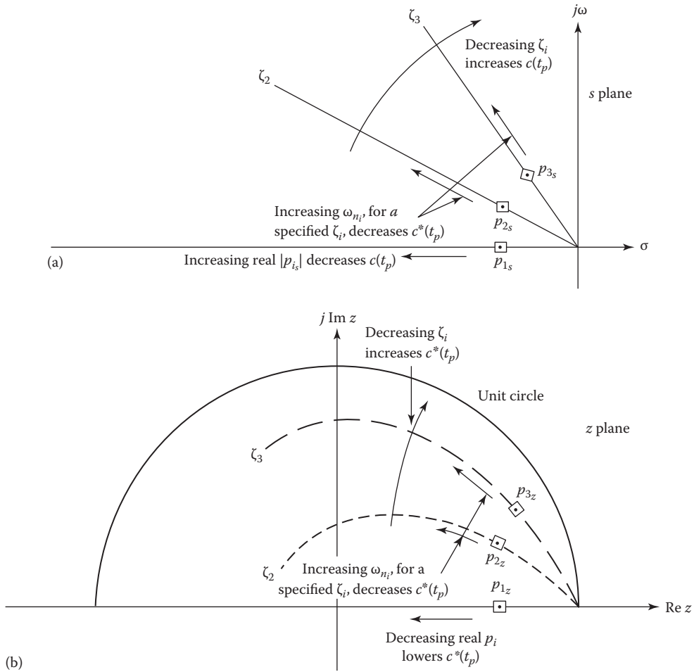
FIGURE 19.27 Desired directional changes in the parameters \zeta_i and \omega_{n_i} and the control ratio's real pole values for decreasing the peak overshoot to a disturbance input: (a) s -plane; (b) z -plane.
