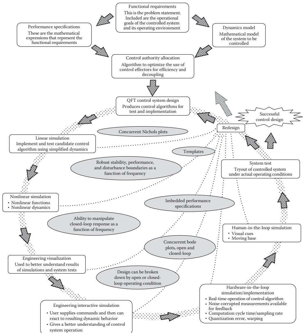
FIGURE 2.2 The QFT control system design process: bridging the gap .
