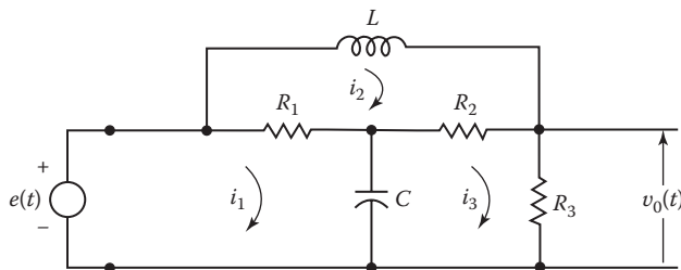
FIGURE 5.3 Multiloop network.
