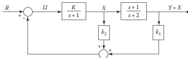
FIGURE 16.5 An uncontrollable state-feedback system.
