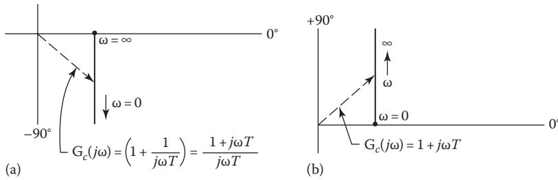
FIGURE 14.3 (a) Ideal integral plus proportional compensator. (b) Ideal derivative plus proportional compensator.
