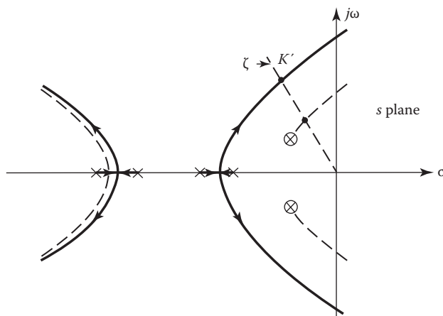
FIGURE 13.25 Root locus of G_c(s)G_x(s) = K'_0/((1 + T_1s)(1 + T_2s)(1 + T_3s)(1 + T_4s)) .
