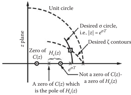
FIGURE 19.23 A plot of the poles and zeros of Equation 19.94.
