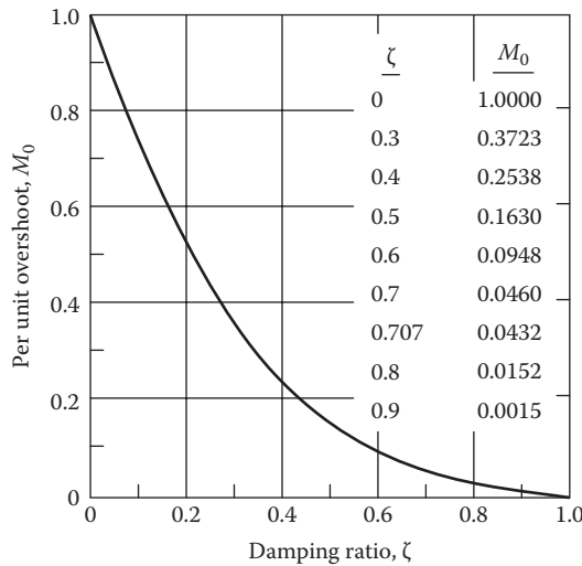
FIGURE 6.7 Peak overshoot versus damping ratios for a simple second-order equation D^2c/\omega_n^2 + (2\zeta/\omega_n)Dc + c = r(t) .
