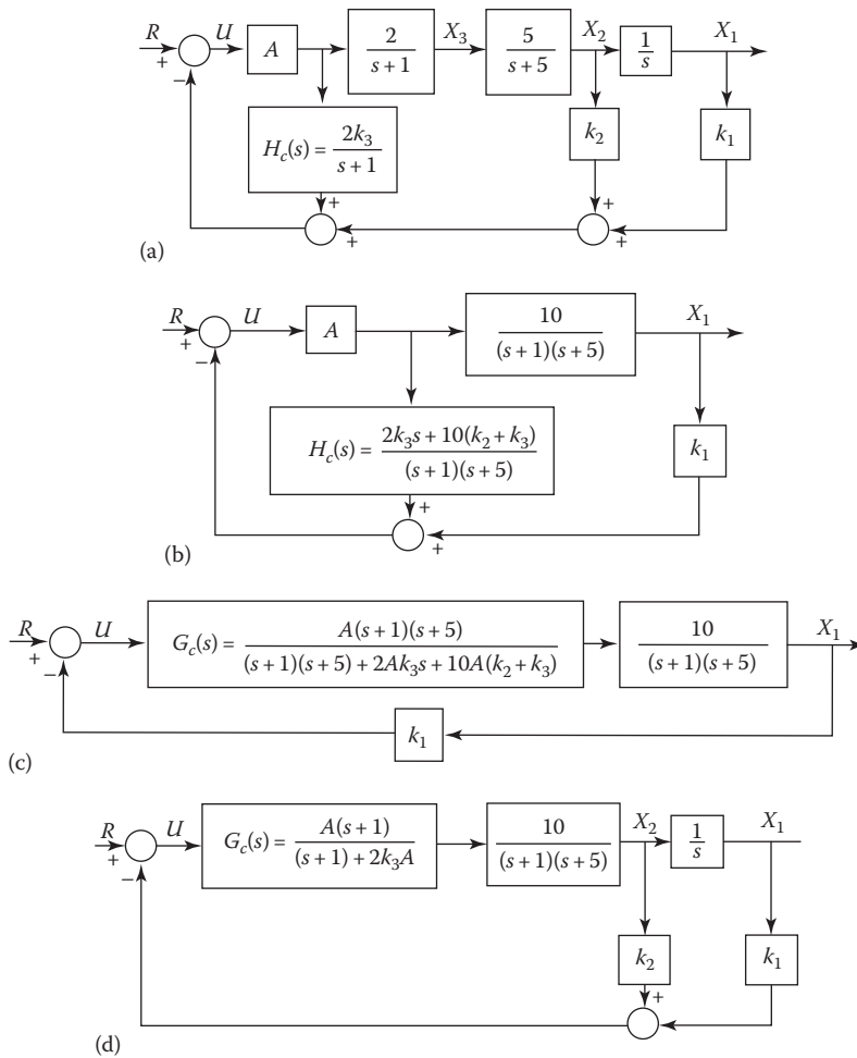
FIGURE 17.8 Manipulation of state feedback to the left for (a) the feedback coefficient k_3 of the control system of Figure 17.5b. (b) The feedback coefficient k_2 of Figure 17.8a. (c) The function H_c(s) of Figure 17.8b. (d) The manipulation to the right of the feedback function H_c(s) of Figure 17.8a.
