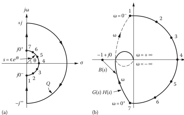
FIGURE 11.26 (a) The contour Q that encircles the RH s plane and (b) complete plot for Equation 11.57.
