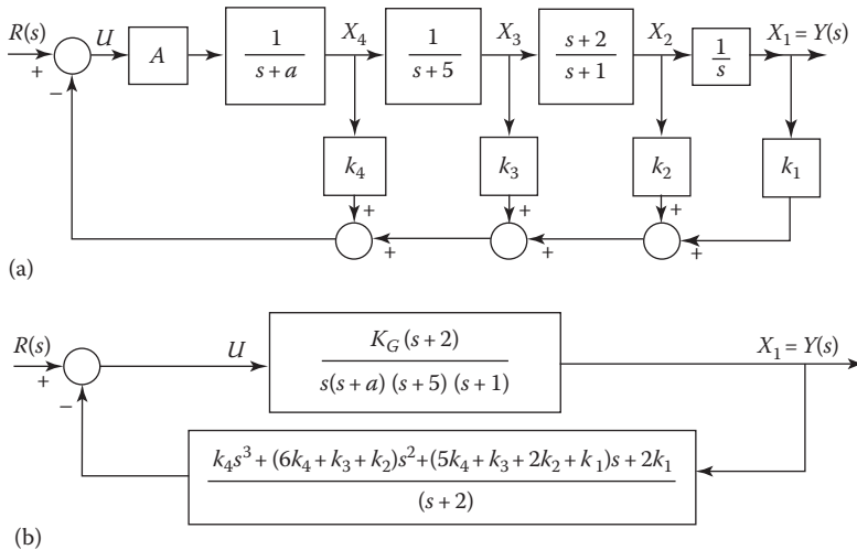
FIGURE 16.17 Closed-loop zero cancellation by state-variable feedback: (a) detailed block diagram and (b) H -equivalent reduction (where K_G = A ).
