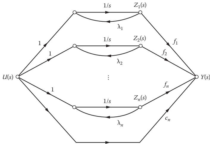
FIGURE 8.31 Simulation of Equation 8.67 by parallel decomposition for w = n . (Jordan diagram for distinct roots.)
