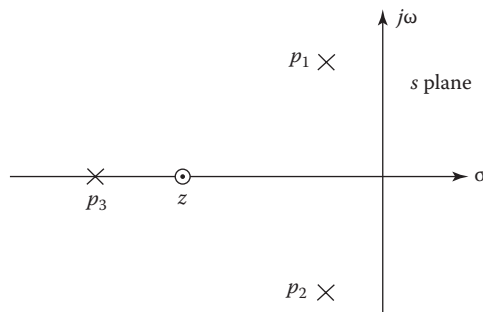
FIGURE 13.5 Pole–zero diagram of C(s)/R(s) for Equation 13.18.
