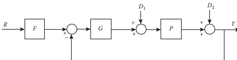
FIGURE 15.14 A MISO system.
