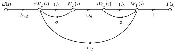
FIGURE 8.34 Simulation diagram for Equations 8.134 and 8.135.
