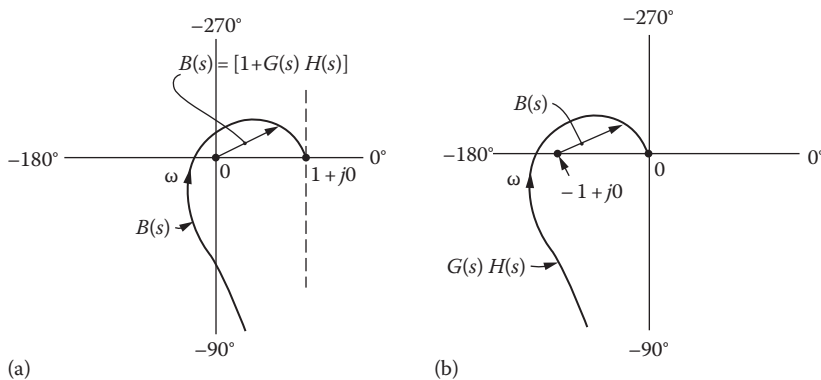
FIGURE 11.24 A change of reference for B(s) . The directed line segment B(s) (a) rotating about the origin and (b) rotating about the -1 + j0 point.
