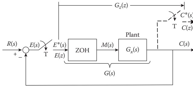
FIGURE 19.8 The uncompensated sampled-data control system.
