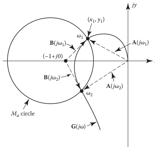
FIGURE 12.8 A plot of the transfer function \mathbf{G}(j\omega) and the M_a circle.
