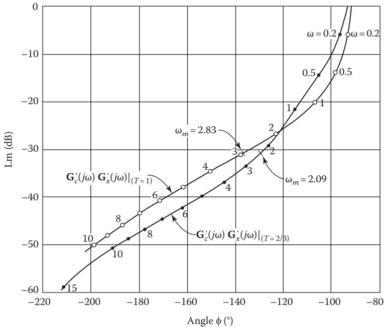
FIGURE 14.14 Lm-angle diagrams with lead compensators from Figure 14.13a and b.
