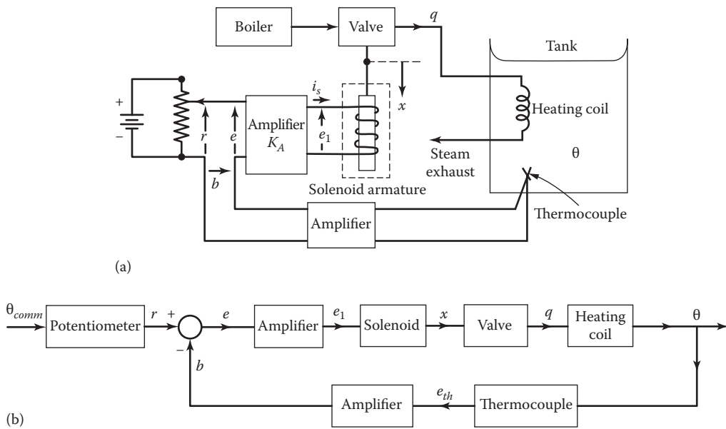
FIGURE 8.1 An industrial process temperature control system. (a) An industrial process system. (b) The block diagram representation of (a).
