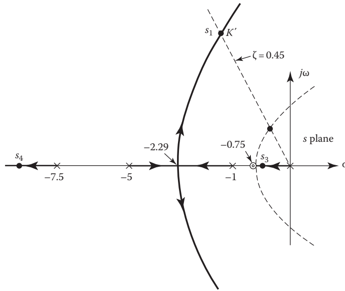
FIGURE 13.17 Root locus of G(s) = AK(s + 0.75)/(s(s + 1)(s + 5)(s + 7.5)) .
