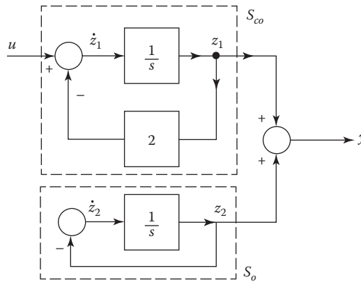
FIGURE 16.3 Simulation diagram for the system of Equations 16.17 and 16.18.
