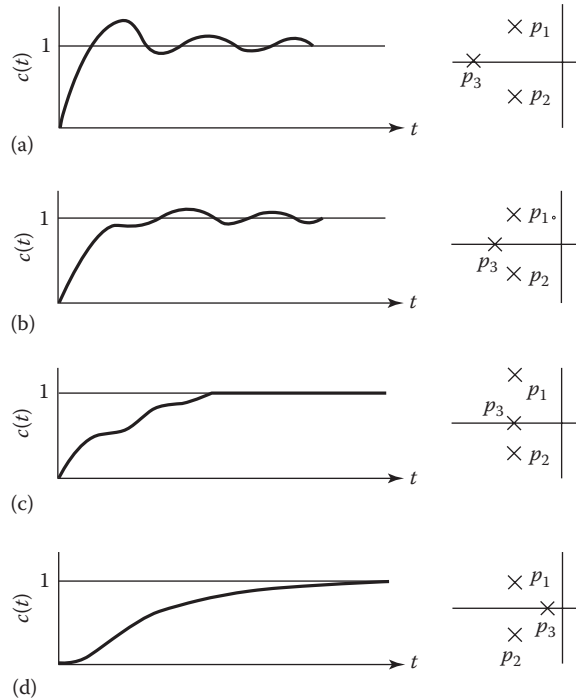
FIGURE 13.4 Typical time responses as a function of the real pole location (a–d).
