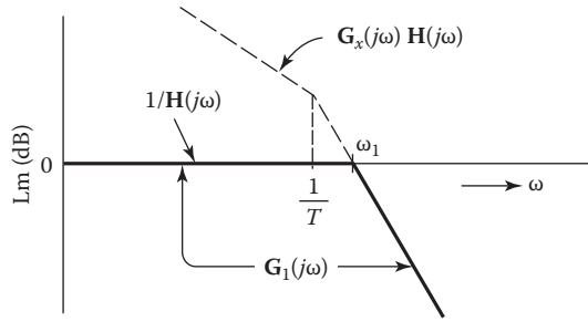
FIGURE 14.21 Lm curves for \mathbf{G}_x(j\omega)\mathbf{H}(j\omega) = K_1/j\omega(1 + j\omega T) and the approximate forward transfer function \mathbf{G}_1(j\omega) for \mathbf{H}(j\omega) = 1 .
