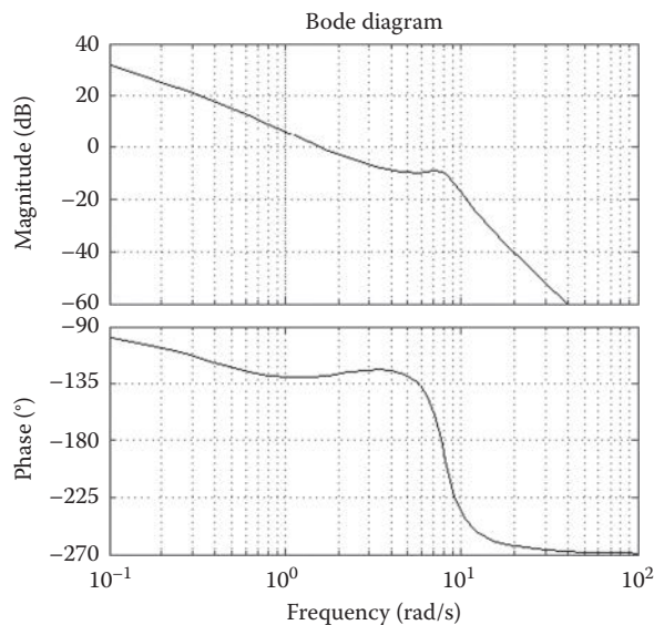
FIGURE 11.8 MATLAB® Bode plots corresponding to Figures 11.6 and 11.7.
