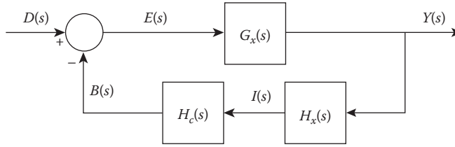
FIGURE 15.8 A control system with a disturbance input.
