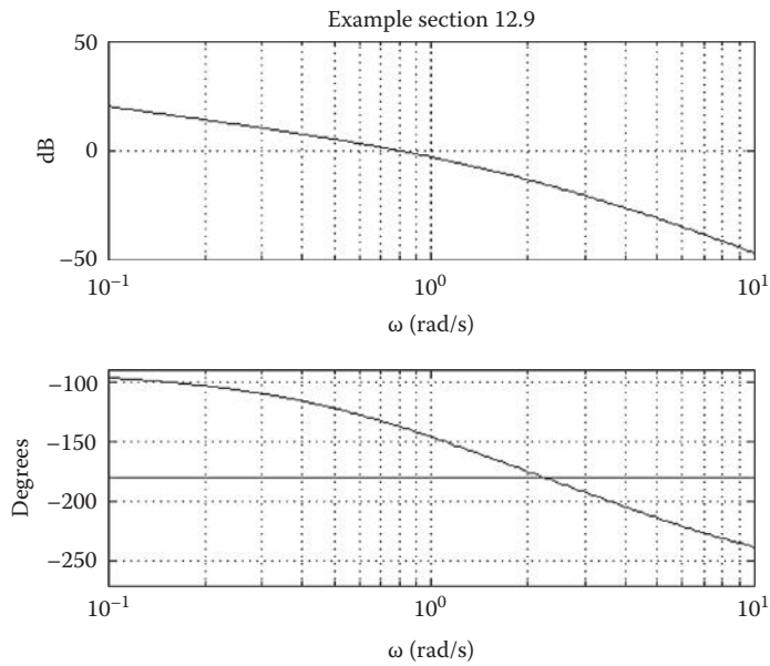
FIGURE 12.21 MATLAB® Bode plots for K = 5 .
