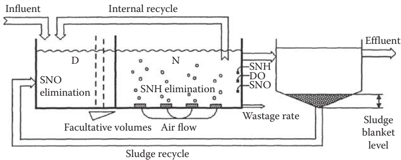
FIGURE 1.7 Wastewater treatment plant.
