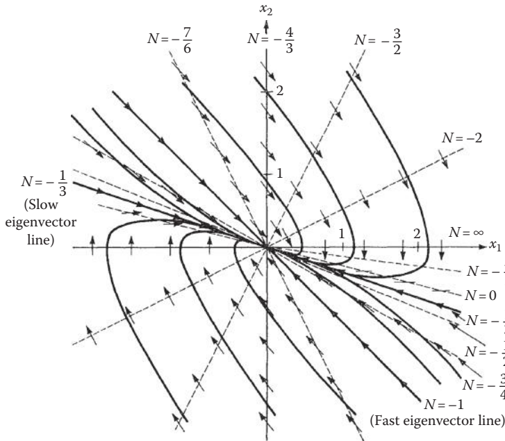
FIGURE 17.10 Phase-plane portrait for Equation 17.30.
