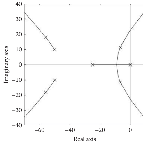
FIGURE 10.18 Root locus for G(s)H(s) = G(s)H(s) = \frac{65,000K_1}{s(s+25)(s^2+100s+2600)} .
