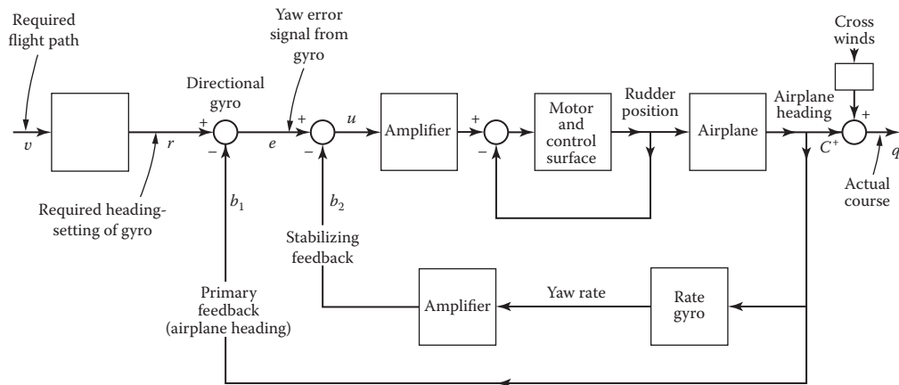
FIGURE 8.5 Airplane directional control system.
