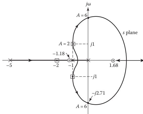
FIGURE 16.16 Root locus for Equation 16.120.
