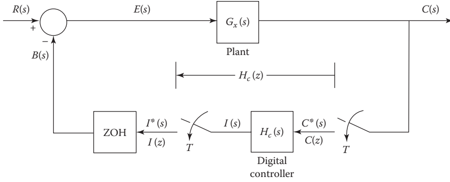
FIGURE 19.22 A feedback-compensated digital control system.
