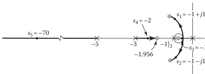
FIGURE 16.20 Root locus for Equation 16.133. (Drawing is not to scale.)
