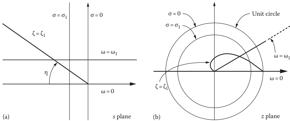
FIGURE 18.7 (a) s -plane representation of the desired values of \zeta_1 , \sigma_1 , \omega_1 , \omega = 0 , and \eta . (b) The transformation of these s plane values into the z plane.
