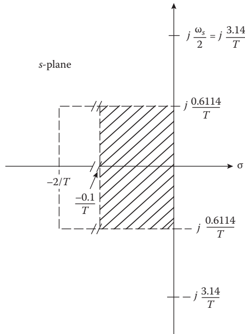
FIGURE 19.5 Allowable location (crosshatched area) of dominant poles and zeros in s -plane for a good Tustin approximation.
