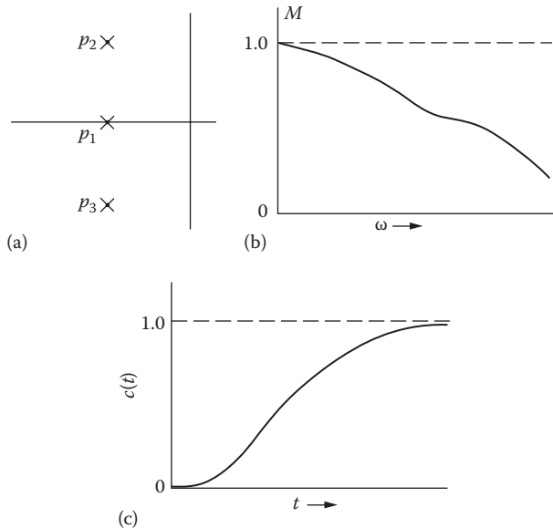
FIGURE 12.26 Form of the frequency and time responses for a particular pole pattern of Equation 12.53. (a) A particular pole pattern in the complex plane. (b) The frequency response corresponding to this pole pattern. (c) The unit step response for this particular pole pattern.
