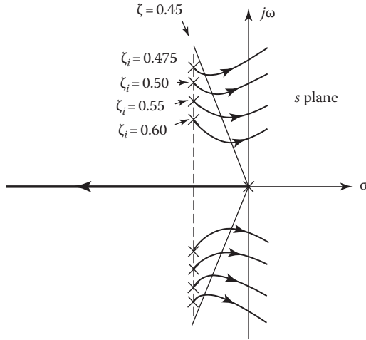
FIGURE 13.34 Root locus of complete system for several values of \zeta_i .
