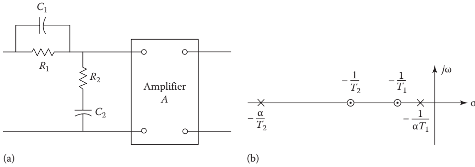
FIGURE 13.22 (a) Lag–lead compensator, (b) pole and zero locations.
