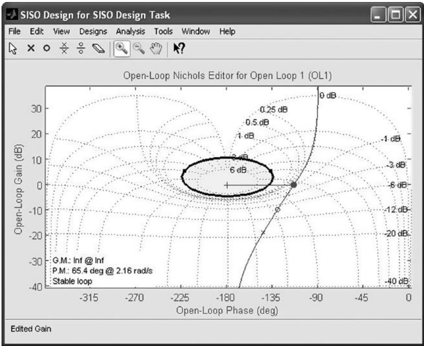
FIGURE C.9 Nichols chart diagram SISOTOOL window with grid and bounds.
