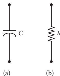
FIGURE 5.19 Network elements representing thermal systems.
