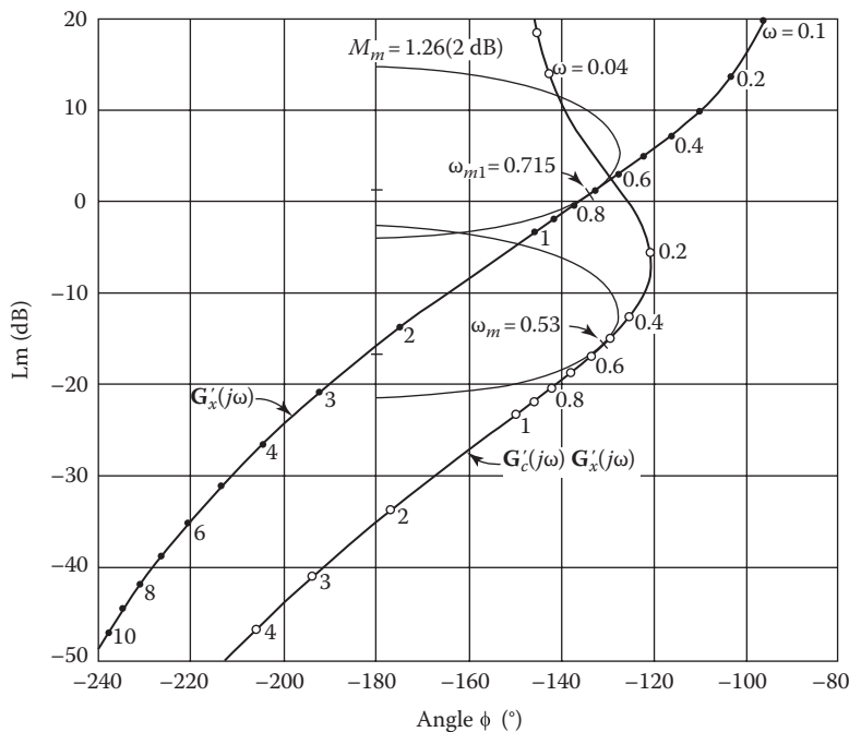
FIGURE 14.8 Lm-angle diagram: original and lag-compensated systems.
