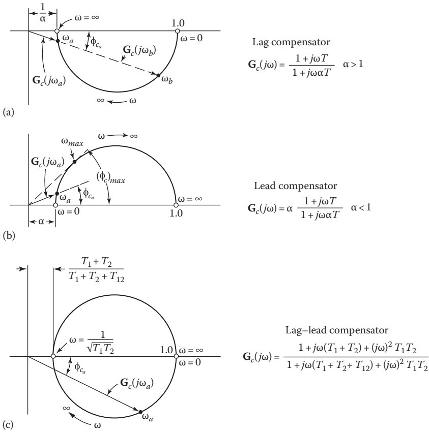
FIGURE 14.2 Polar plots: (a) lag compensator, (b) lead compensator, and (c) lag-lead compensator.
