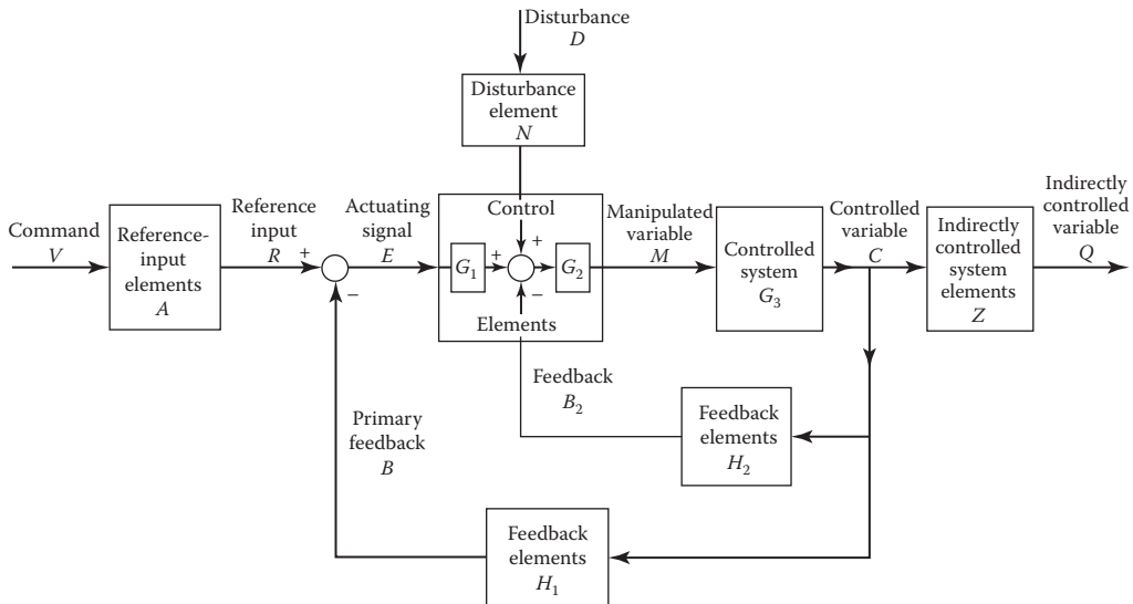
FIGURE 8.8 Block diagram of representative feedback control system showing multiple feedback loops. (All uppercase letters denote transformation.)
