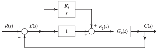
FIGURE 13.7 Ideal proportional PI control.
