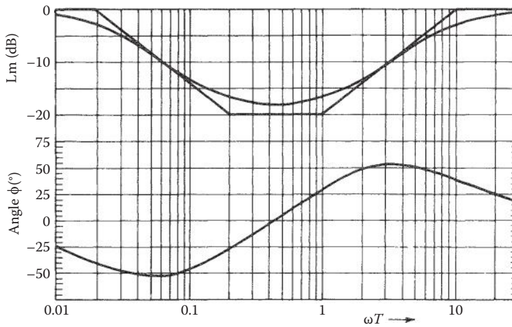
FIGURE 14.16 Lm and phase-angle diagram for lag-lead compensator \mathbf{G}'_c(j\omega) = \frac{(1 + j5\omega T_2)(1 + j\omega T_2)}{(1 + j50\omega T_2)(1 + j0.1\omega T_2)} .
