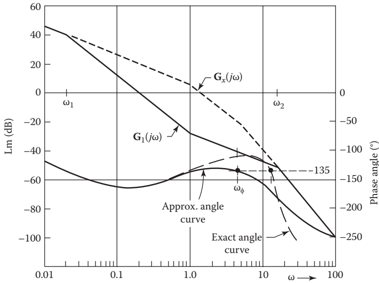
FIGURE 14.25 Lm and phase-angle diagrams of \mathbf{G}_1(j\omega) = \frac{2(1+j\omega)}{j\omega(1+j47.5\omega)(1+j0.0625\omega)^2} .
