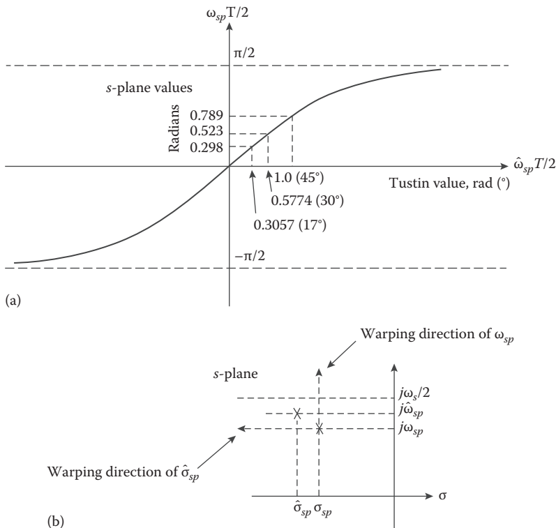
FIGURE 19.4 Map of \hat{\omega} = 2(\tan \omega_{sp}T/2)/T . (a) Plot of Equation 19.13 and (b) warping effect.
