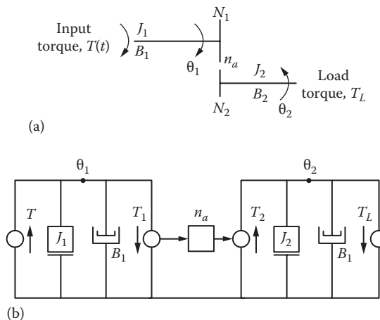
FIGURE 5.18 (a) Representation of a gear train; (b) corresponding mechanical network.
