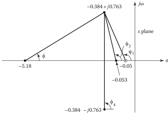
FIGURE 13.12 Angles used to evaluate T_p .
