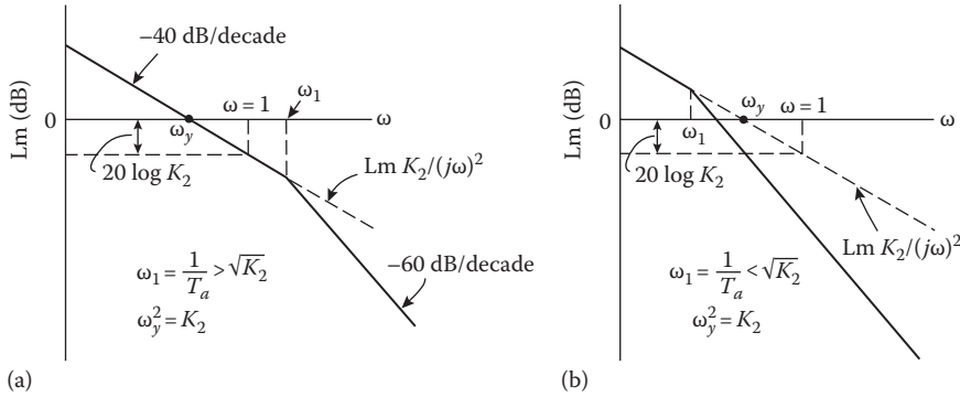
FIGURE 11.11 Lm plot for G(j\omega) = K_2/(j\omega)^2(1 + j\omega T_a) . The Lm plot when (a) \omega_1 > \sqrt{K_2} and (b) \omega_1 < \sqrt{K_2} .
