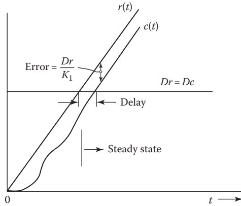
FIGURE 9.6 Steady-state response of a Type 1 system with a ramp input.
