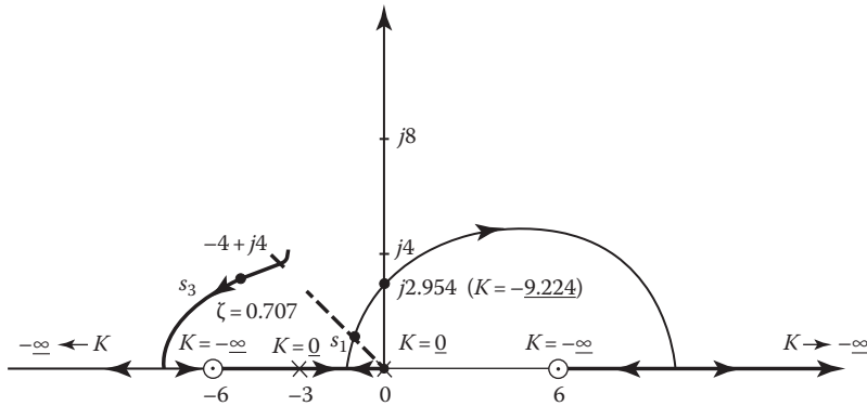
FIGURE 10.21 Root locus for Equation 10.73 for negative values of K .
