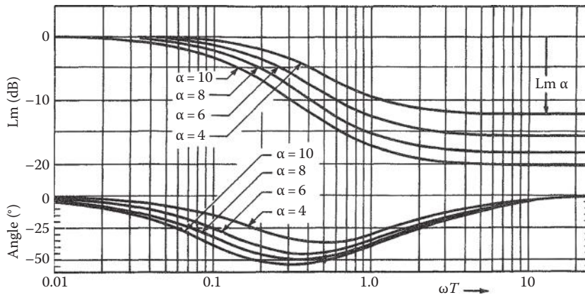
FIGURE 14.4 Lm and phase-angle diagram for lag compensator \mathbf{G}'_c(j\omega) = \frac{1 + j\omega T}{1 + j\omega\alpha T} .
