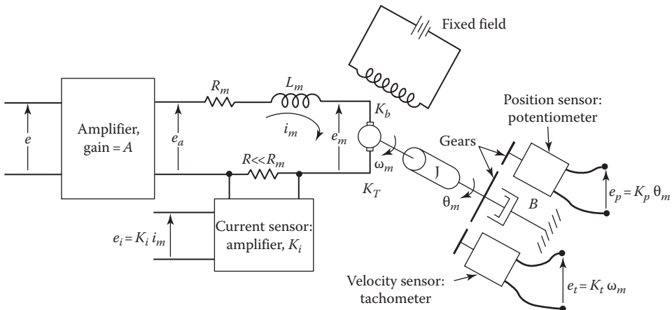
FIGURE 16.6 Open-loop position-control system and measurement of states.
