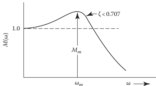
FIGURE 12.5 A closed-loop frequency-response curve indicating M_m and \omega_m .
