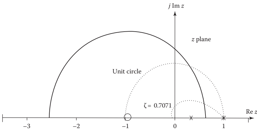
FIGURE 19.16 Lead compensation: root locus for Equation 19.59.
