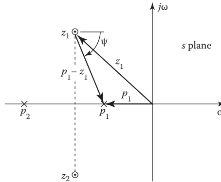
FIGURE 7.6 Directed line segments drawn on a pole–zero diagram of a function F(s) .
