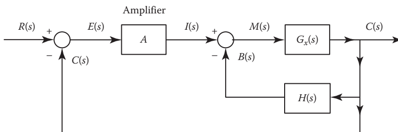
FIGURE 13.29 Block diagram for feedback compensation.
