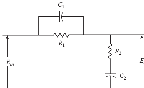
FIGURE 11.12 An RC circuit used as a lag-lead compensator.
