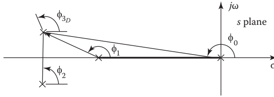
FIGURE 10.16 Location of the breakaway point.
