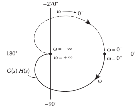
FIGURE 11.27 Plot of a typical Type 0 transfer function G(s)H(s) for -\infty < \omega < \infty .
