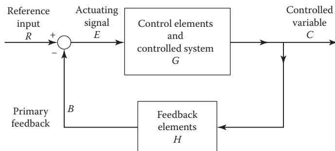
FIGURE 8.6 Block diagram of a feedback system.
