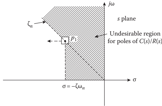
FIGURE 15.2 Location of the desired dominant pole.
