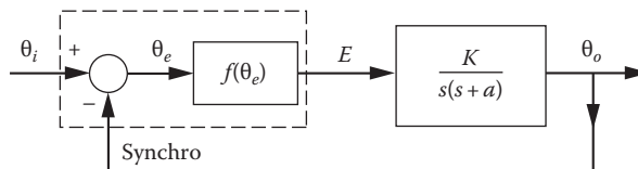
FIGURE 17.11 A nonlinear feedback control system.
