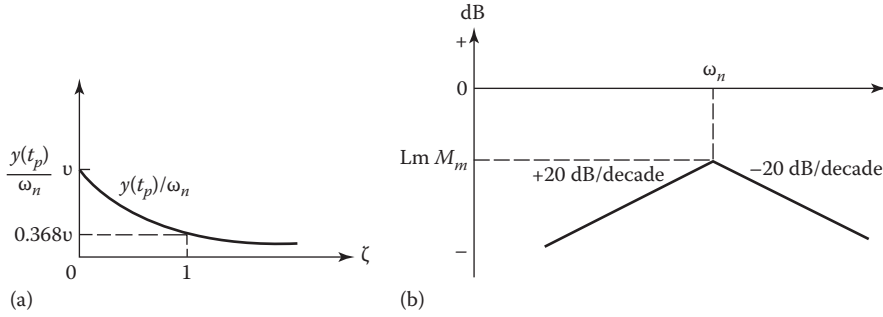
FIGURE 15.7 (a) Peak value of Equation 15.14, using Equation 15.17. (b) Bode plot characteristics of Equation 15.18.
