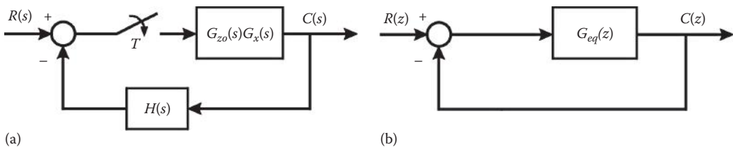
FIGURE 18.16 (a) A stable nonunity-feedback S-D system; (b) the equivalent z domain-stable unity-feedback system of Figure 18.16a.
