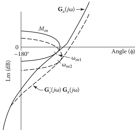
FIGURE 14.12 Original and lead-compensated Lm–angle curves.
