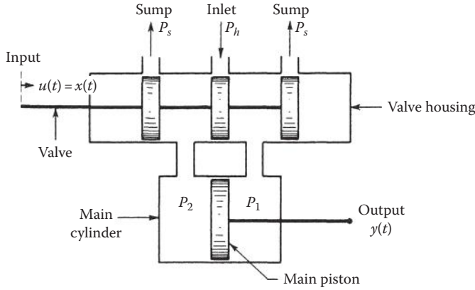
FIGURE 5.21 Hydraulic actuator.
