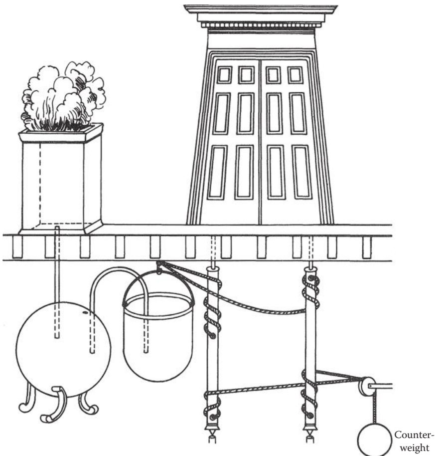
FIGURE 1.9 Hero's device for opening temple doors.
