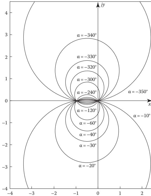
FIGURE 12.12 Constant \alpha contours.
