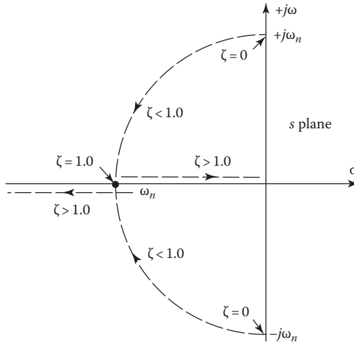
FIGURE 10.25 Variation of roots of a simple second-order system for a constant \omega_n .
