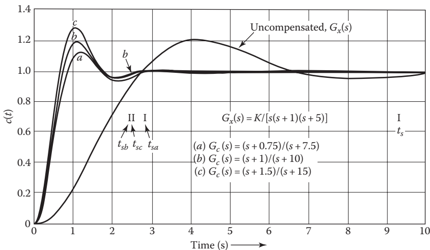
FIGURE 13.20 Time response with a step input for the uncompensated and the lead-compensated cases of Table 13.1.
