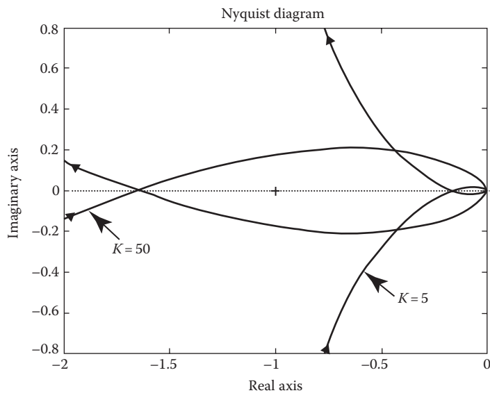
FIGURE 12.22 MATLAB® Nyquist plots.
