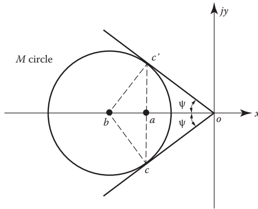
FIGURE 12.13 Determination of \sin \psi .
