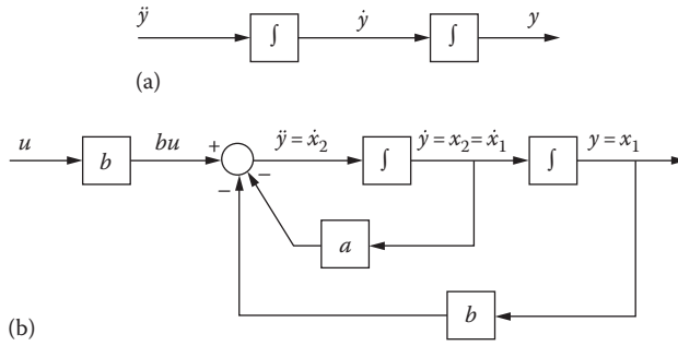
FIGURE 8.17 Simulation diagram for Equation 8.32. (a) Representation of integration. (b) The completed simulation diagram.
