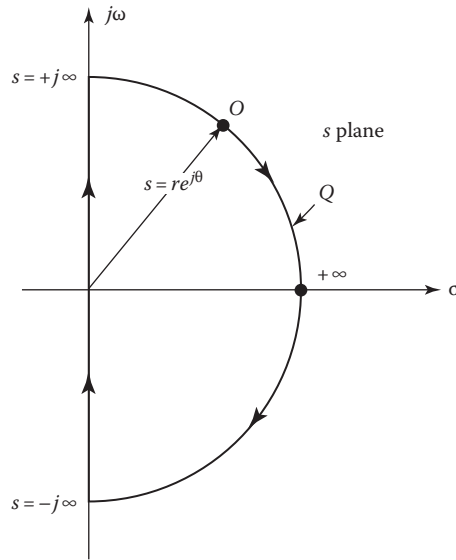
FIGURE 11.23 The contour that encloses the entire RH s plane.
