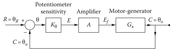
FIGURE 8.15 Equivalent representation of Figure 8.9.
