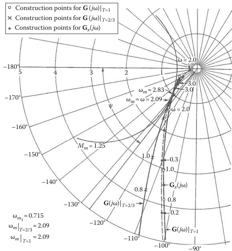
FIGURE 14.15 Polar plots of Type 1 control system with and without lead compensation:
