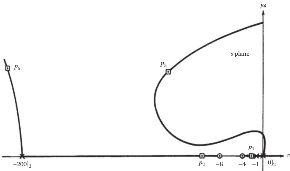
FIGURE 19.28 A possible root locus for Equation 19.115 (not to scale).
