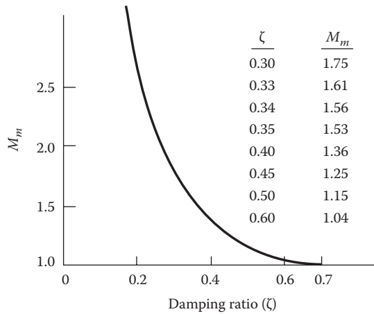
FIGURE 12.6 A plot of M_m versus \zeta for a simple second-order system.
