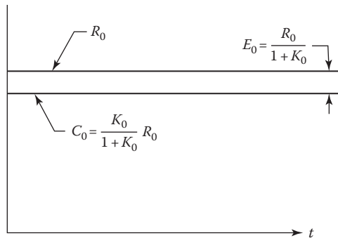
FIGURE 9.5 Steady-state response of a Type 0 system with a step input.
