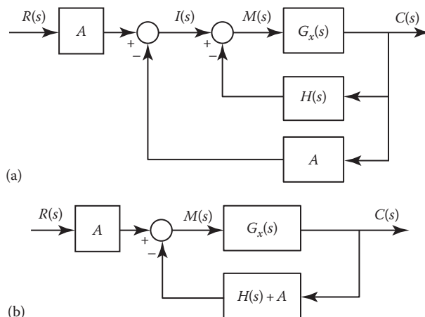
FIGURE 13.32 (a) A detailed block diagram and (b) its equivalent block diagram.
