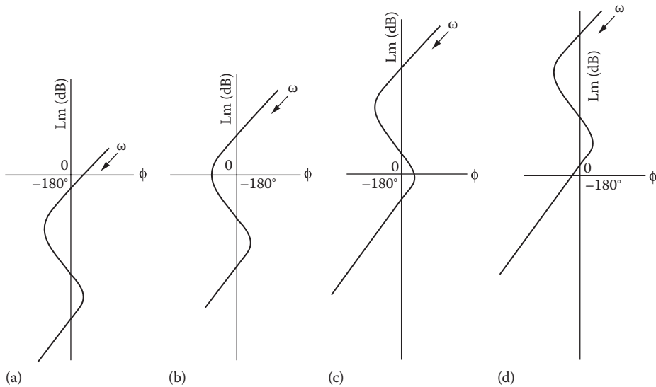
FIGURE 11.37 Lm-angle diagram for a conditionally stable system: (a), (c) stable; (b), (d) unstable.
