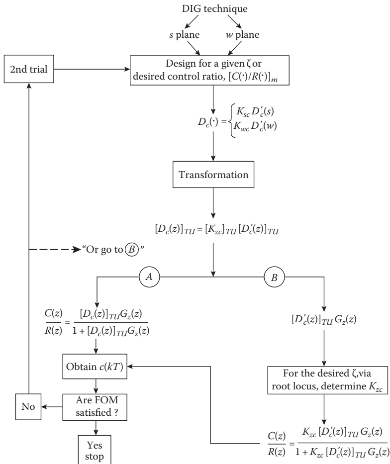
FIGURE 19.7 DIG design philosophy for Figure 19.1.
