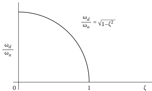
FIGURE 6.8 Frequency of oscillation versus damping ratio.
