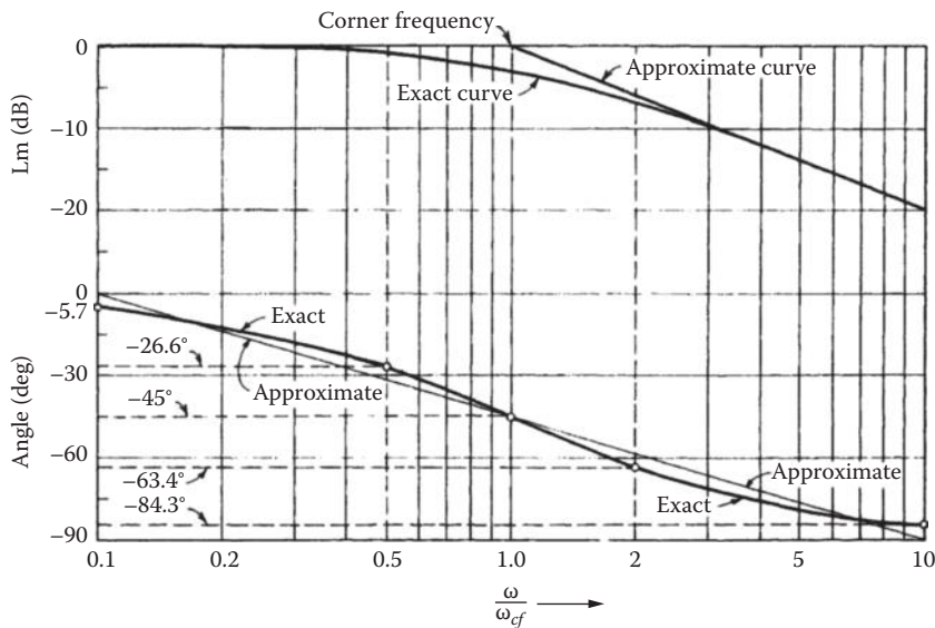
FIGURE 11.2 \text{Lm} and phase diagram for (1 + j\omega T)^{-1} = [1 + j(\omega/\omega_{cf})]^{-1} .
