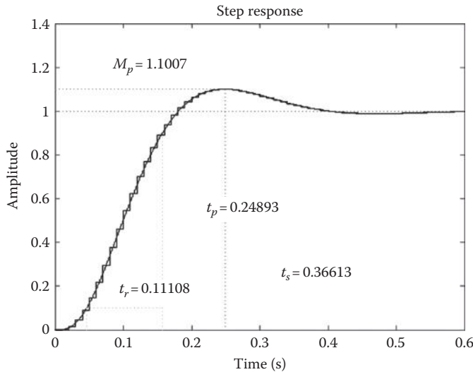
FIGURE 19.21 MATLAB® step response for T = 0.1 s and FOM for Equations 19.78 and 19.80.
