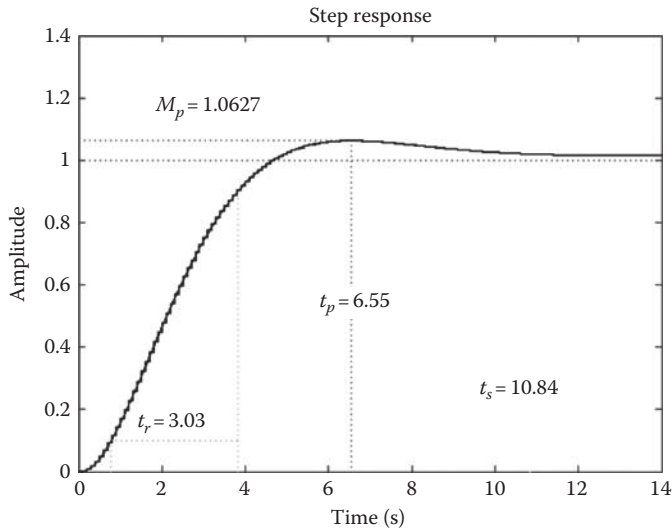
FIGURE 19.19 MATLAB® step response for T = 0.1 s, FOM for Equation 19.64 (DIG), and the DIR control ratio given in the m-file.
