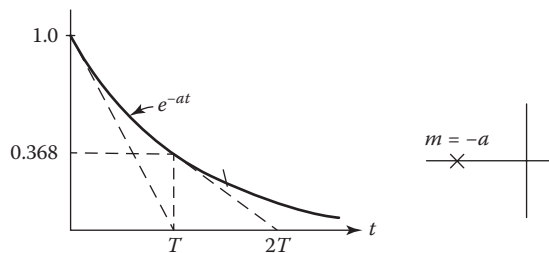
FIGURE 6.3 Plot of the exponential e^{-at} and the root location.
