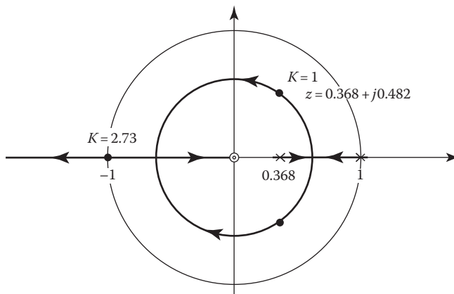
FIGURE 18.11 Root locus for Equations 18.44 and 18.45.
