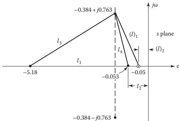
FIGURE 13.13 Lengths used to evaluate M_0 .
