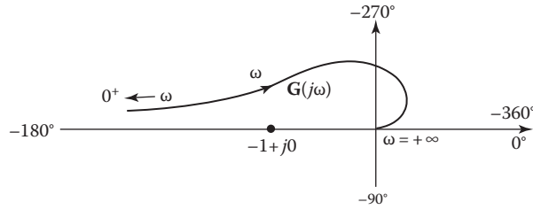
FIGURE 11.17 Polar plot of Equation 11.43, a typical Type 2 transfer function resulting in an unstable feed-back control system.
