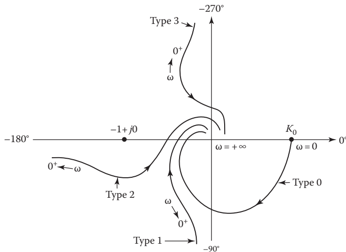
FIGURE 11.20 A summary of direct polar plots of different types of system.
