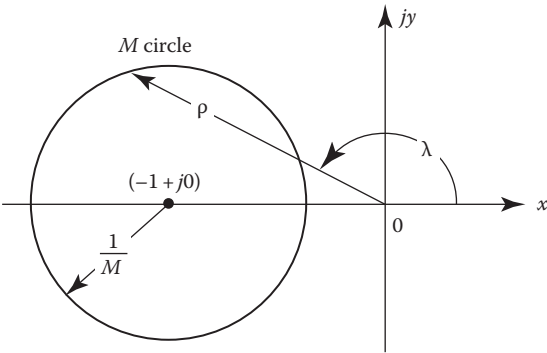
FIGURE 12.19 Constant M circle on the inverse polar plot.
