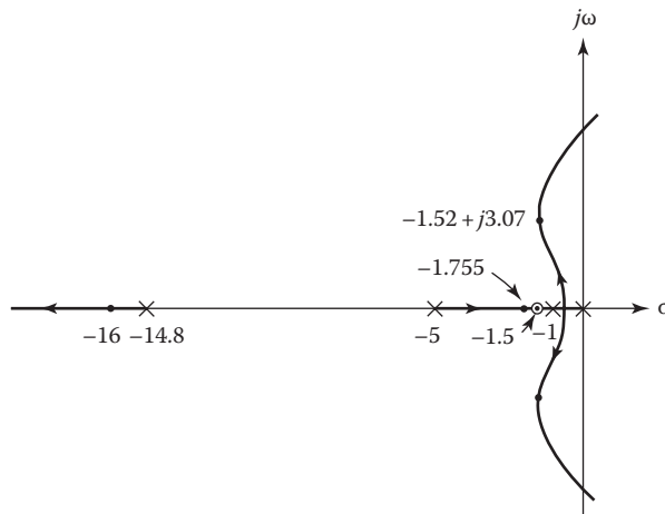
FIGURE 15.5 Root-locus plot for Example 15.1.
