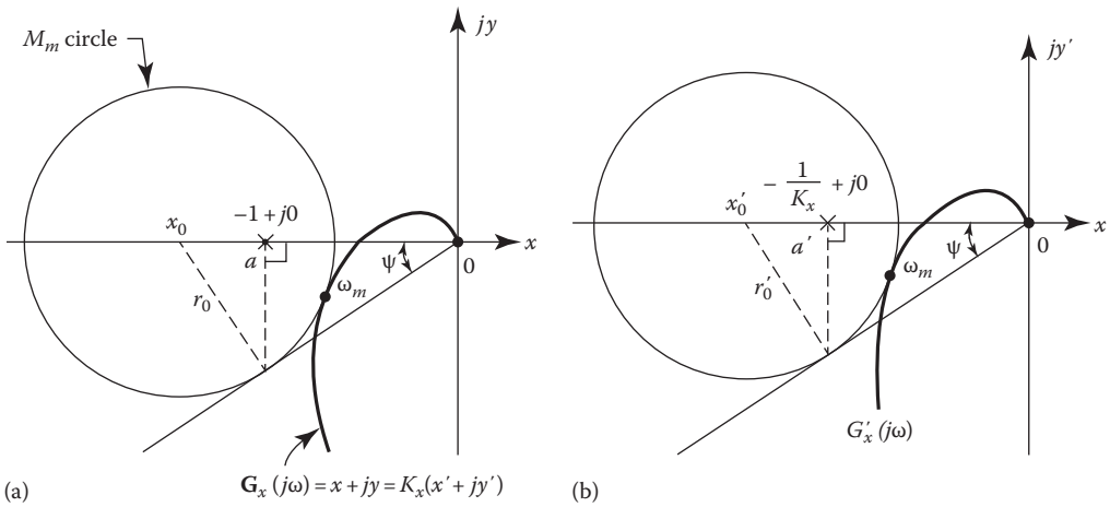
FIGURE 12.17 (a) Plot of \mathbf{G}_x(j\omega) with the respective M_m circle. (b) Circle drawn tangent both to the plot of \mathbf{G}'_x(j\omega) and to the line representing the angle \psi = \sin^{-1}(1/M_m) .
