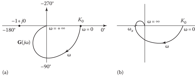
FIGURE 11.14 Polar plot for typical Type 0 transfer functions: (a) Equation 11.33 and (b) Equation 11.34.
