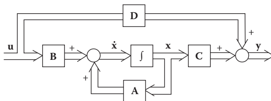
FIGURE 8.19 General matrix block diagram representing the state and output equations.
