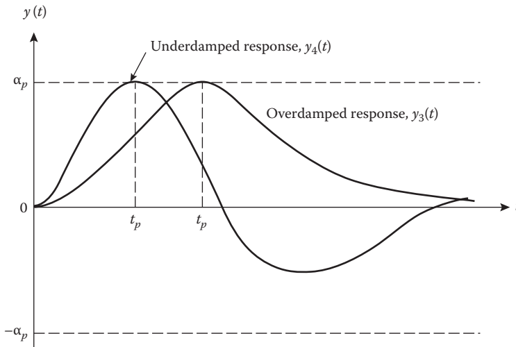
FIGURE 15.16 Disturbance-rejection time response for Figure 15.14 with r(t) = d_2(t) = 0 and d_1(t) = D_0 u_{-1}(t) .
