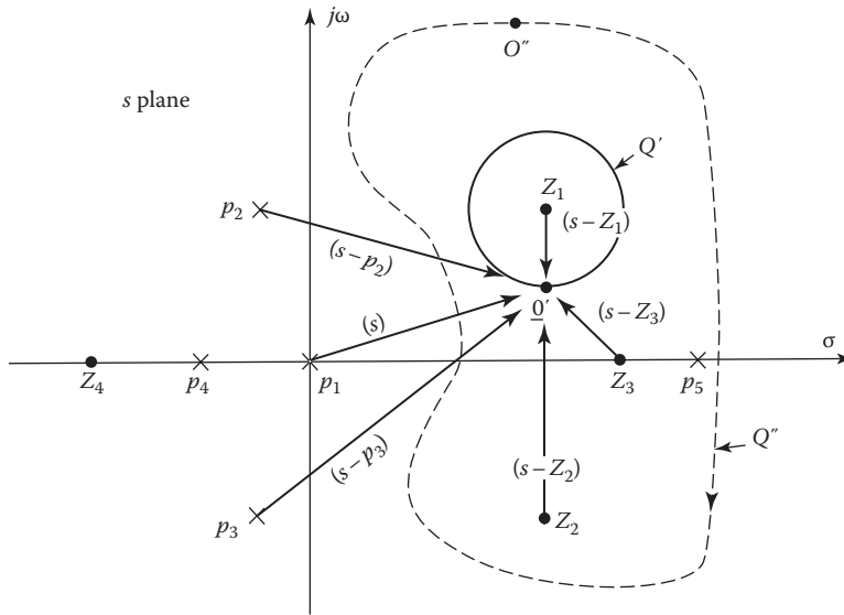
FIGURE 11.22 A plot of some poles and zeros of Equation 11.54.
