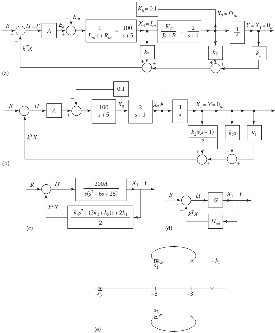
FIGURE 16.7 A position-control system with feedback, its H_{eq} representation, and the corresponding root locus. (a) A position-control system with feedback. (b) A simplified block diagram of (a). (c) A further block diagram reduction. (d) The H_{eq} block diagram. (e) A possible desired pole–zero location in the s -plane.
