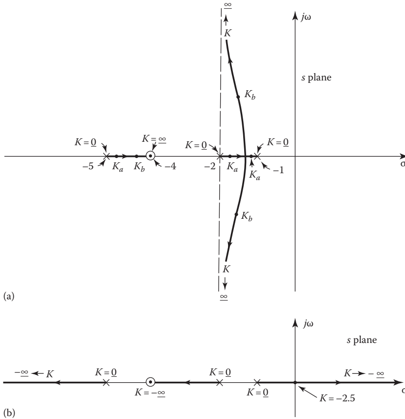
FIGURE 10.8 The complete root locus of Equation 10.36: (a) for K > 0 ; (b) for K < 0 .
