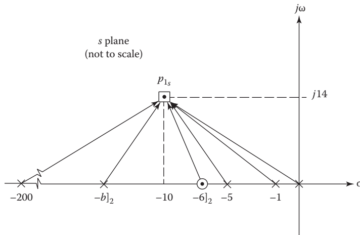
FIGURE 19.29 The plot of the poles and zeros of Equation 19.122: first trial.
