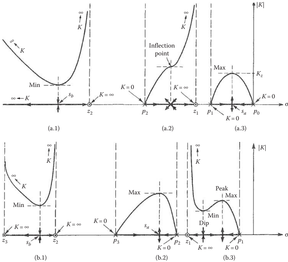
FIGURE 10.11 Six various root-locus plots as K goes from a value 0 to a value of infinity. (a) Plots corresponding to Figure 10.5a. (b) Plots corresponding to Figure 10.5b.
