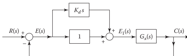
FIGURE 13.14 Ideal proportional PD control.
