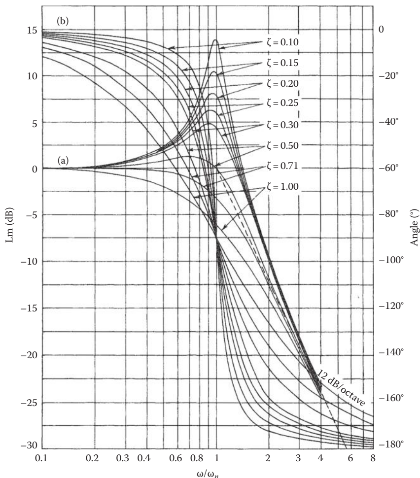
FIGURE 11.4 Lm and phase diagram for [1 + j2\zeta\omega/\omega_n + (j\omega/\omega_n)^2]^{-1} .
