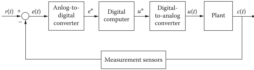
FIGURE 18.1 Control system incorporating a digital computer.
