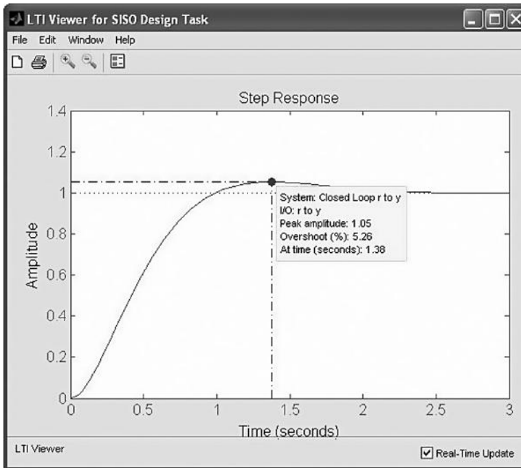
FIGURE C.5 Step response.
