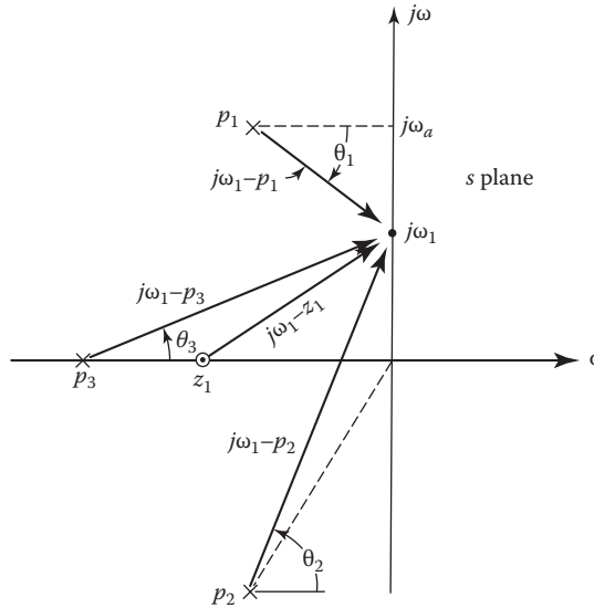
FIGURE 7.8 Pole-zero diagram of Equation 7.76 showing the directed line segments for evaluating the frequency response M < \alpha .
