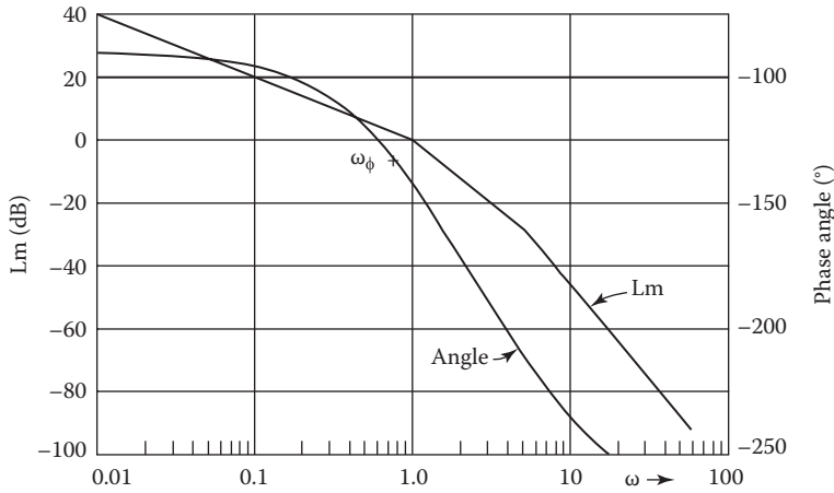
FIGURE 14.22 Lm and phase-angle diagram of \mathbf{G}'_x(j\omega) = \frac{1}{j\omega(1 + j\omega)(1 + j0.2\omega)} .
