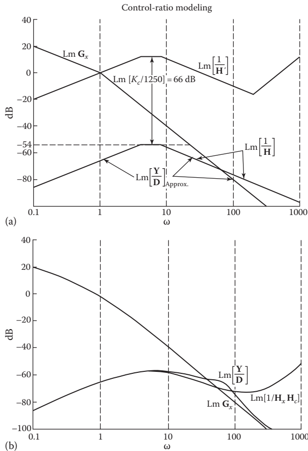
FIGURE 15.12 Bode plot for Example 15.4: (a) straight-line approximations; (b) exact poles.
