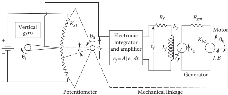
FIGURE 9.8 Position control of a space-vehicle camera (Type 2 system).
