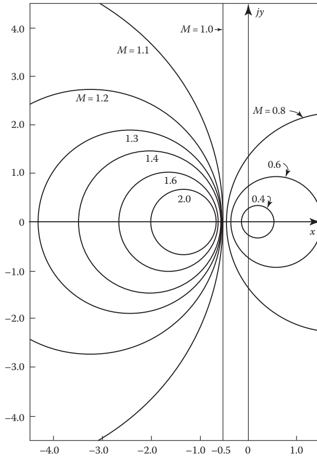
FIGURE 12.10 Constant M contours.
