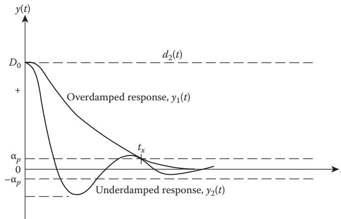
FIGURE 15.15 Disturbance-rejection time response for Figure 15.14 with r(t) = d_1(t) = 0 and d_2(t) = D_0 u_{-1}(t) .
