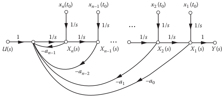
FIGURE 8.28 State diagram for Equation 8.60a.
