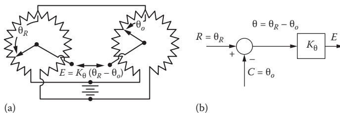
FIGURE 8.10 (a) Rotational position comparison; (b) its block-diagram representation.
