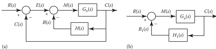
FIGURE 13.30 (a) Minor-loop compensation, (b) simplified block diagram, H_1(s) = 1 + H(s) .
