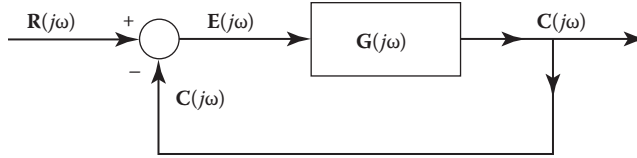
FIGURE 12.1 Block diagram of a simple control system.
