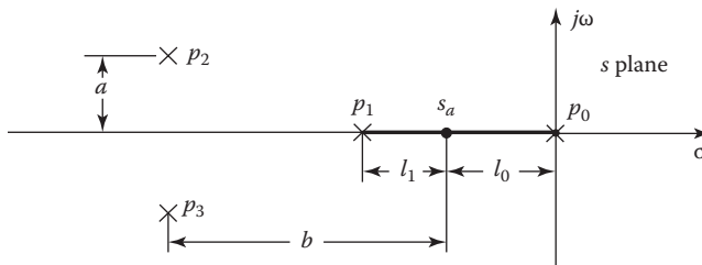
FIGURE 10.15 Nonunity-feedback control system.
