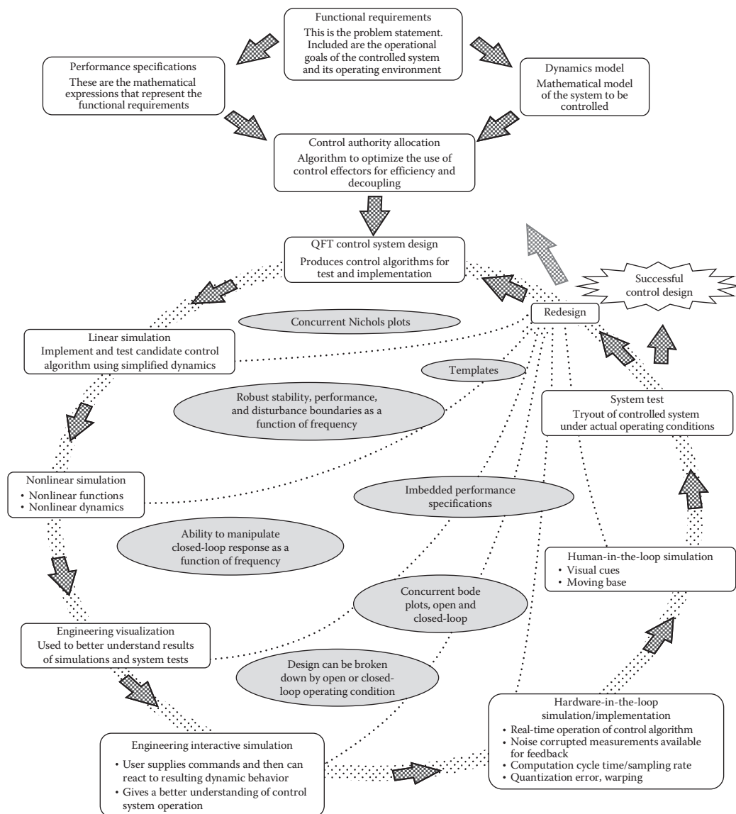
FIGURE 4.3 The QFT control system design process: bridging the gap .
