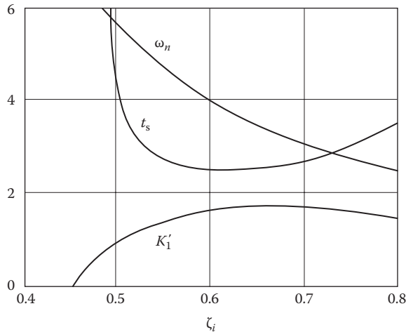
FIGURE 13.35 Variation of K'_1 , t_s , and \omega_n with \zeta_i .
