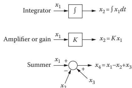
FIGURE 8.16 Elements used in a simulation diagram.
