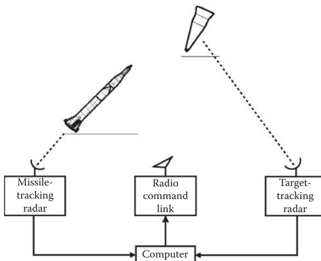
FIGURE 8.2 Command guidance interceptor system.
