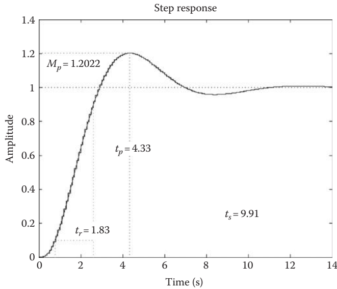
FIGURE 19.10 MATLAB® step response of DIG (PCT) versus DIR technique for T = 0.1 s.
