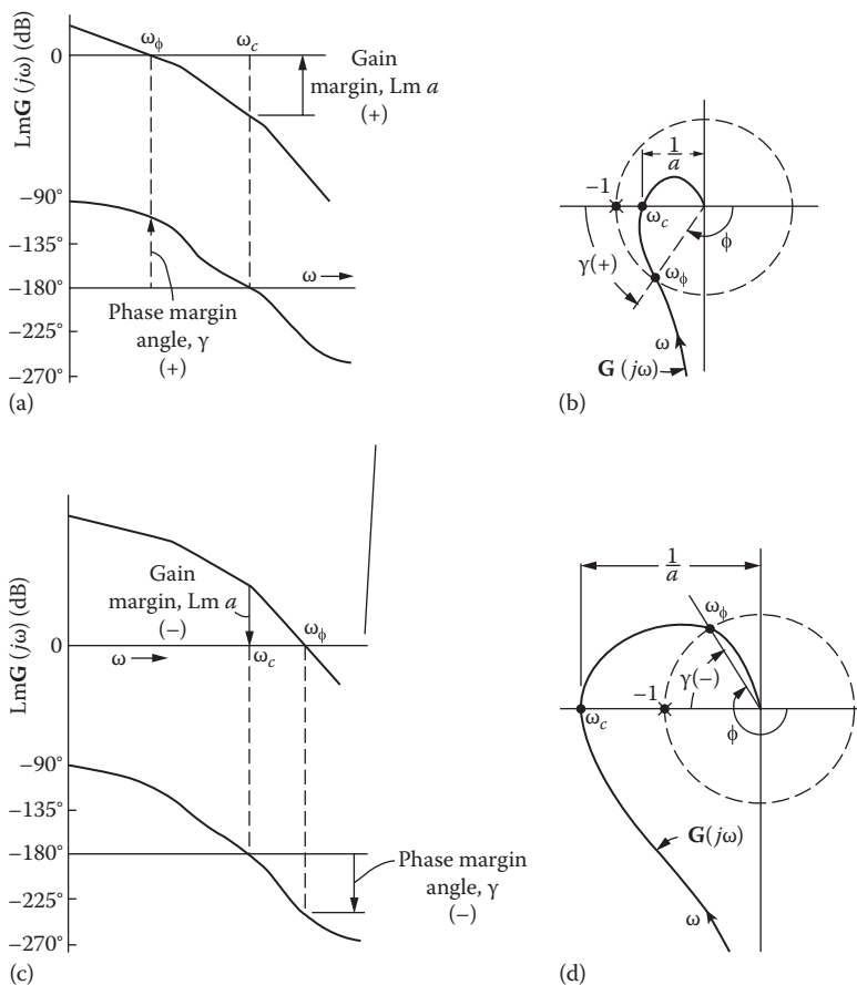
FIGURE 11.34 Lm and phase diagram and polar plots of G(j\omega) , showing gain-margin and phase-margin angle: (a) and (b) stable; (c) and (d) unstable.
