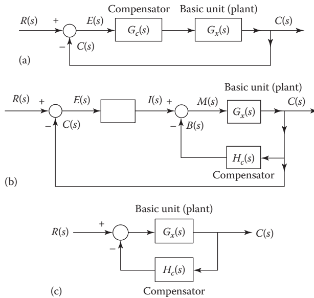
FIGURE 13.1 Block diagram showing the location of compensators: (a) cascade, (b) minor-loop feedback, and (c) output feedback.
