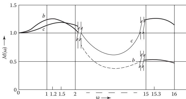
FIGURE 14.27 Closed-loop frequency response.
