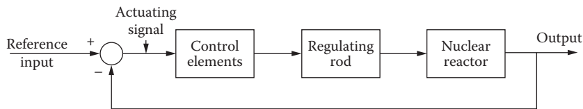
FIGURE 1.11 A feedback system for controlling the power level of a nuclear reactor.
