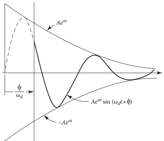
FIGURE 6.2 Sketch of an exponentially damped sinusoid.
