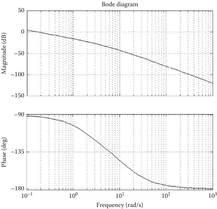
FIGURE C.7 Bode diagram of an example transfer function.
