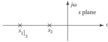
FIGURE 7.2 Location of real poles in the s plane.
