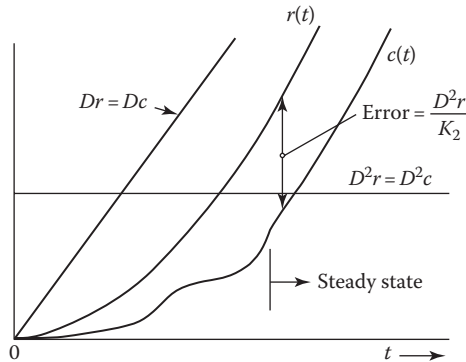
FIGURE 9.7 Steady-state response of a Type 2 system with a parabolic input.
