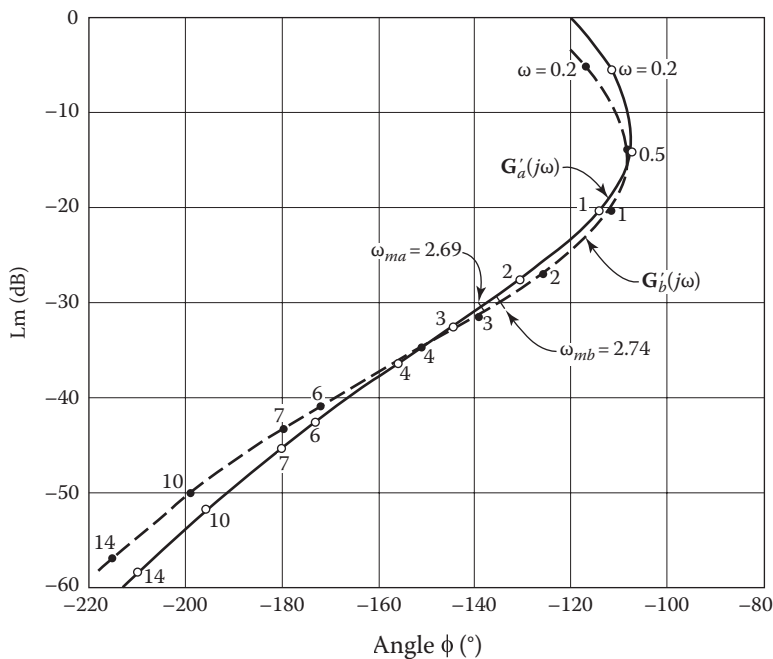
FIGURE 14.19 Lm–angle diagram of \mathbf{G}'(j\omega) from Equation 14.19 -\mathbf{G}'_a with T_1 = 14 and \mathbf{G}'_b with T_1 = 20 .
