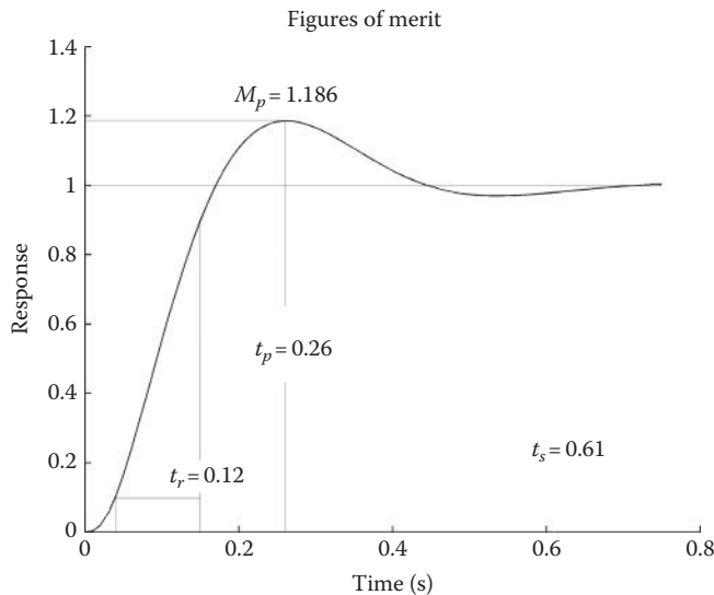
FIGURE 10.19 MATLAB® time response plot corresponding to Equation 10.72 and Figure 10.26.
