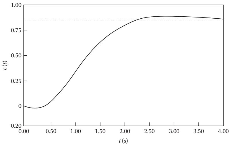
FIGURE 10.22 Step response for the closed-loop system given in Equation 10.75.
