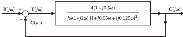
FIGURE 11.5 Block diagram of a control system with unity feedback.
