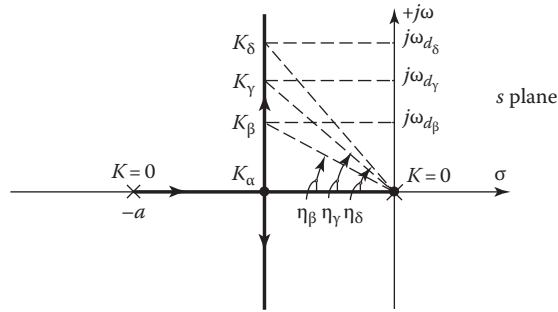
FIGURE 10.3 Root-locus plot of the position-control system of Figure 10.1. \eta = \cos^{-1}\zeta .
