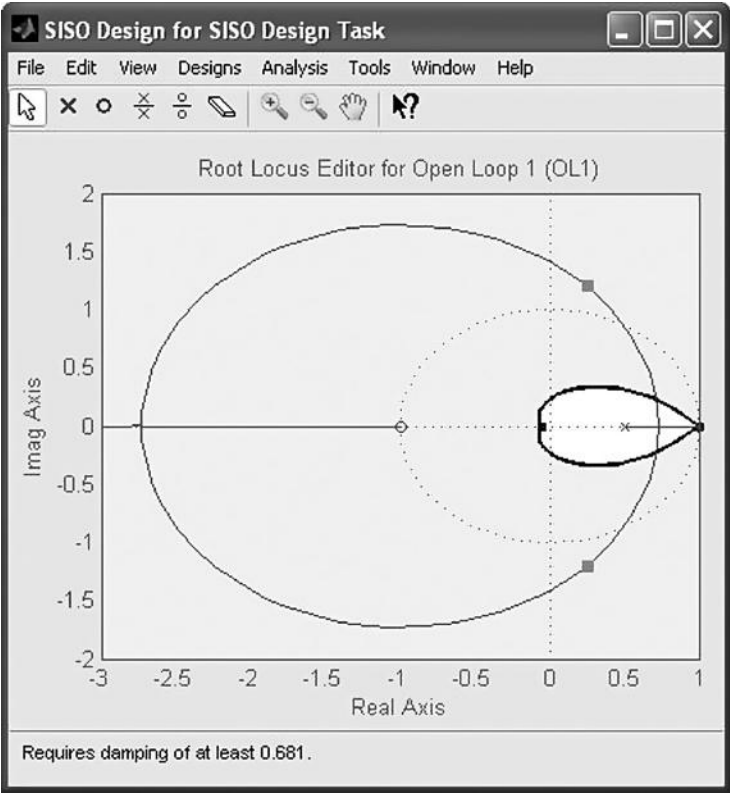
FIGURE C.6 Digital root locus SISOTOOL window.
