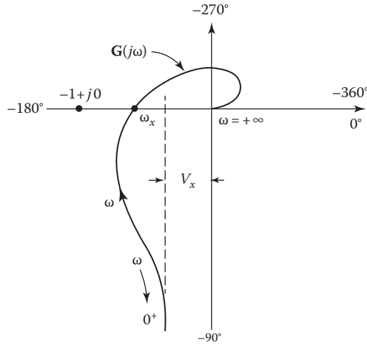
FIGURE 11.16 Polar plot for a typical Type 1 transfer function (Equation 11.36).
