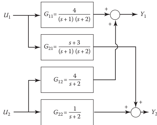
FIGURE 7.15 Block diagram for Equation 7.108.
