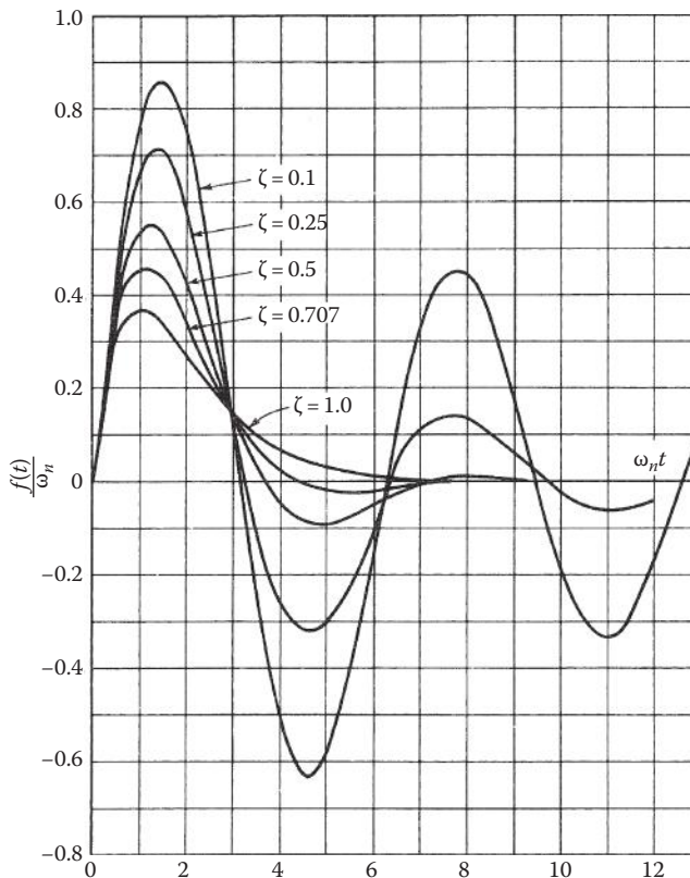
FIGURE 7.14 Response to an impulse for F(s) = \omega_n^2 / (s^2 + 2\zeta\omega_n s + \omega_n^2) .
