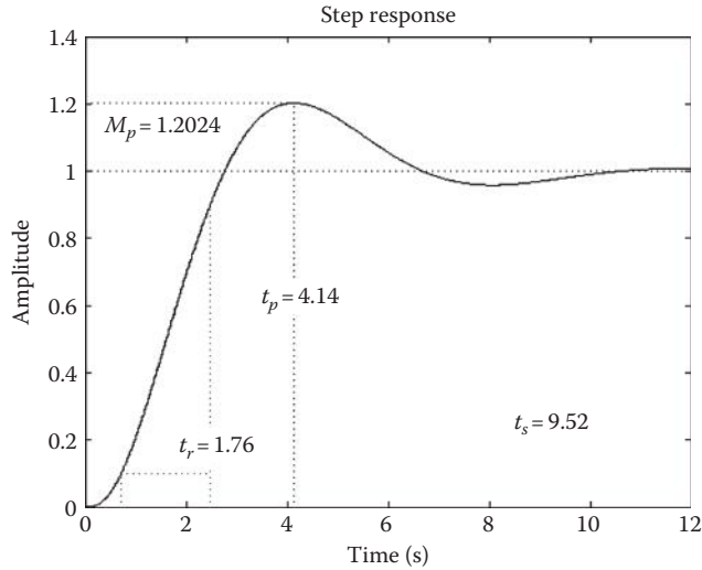
FIGURE 19.11 MATLAB® step response of DIG (PCT) versus DIR technique for T = 0.01 s.
