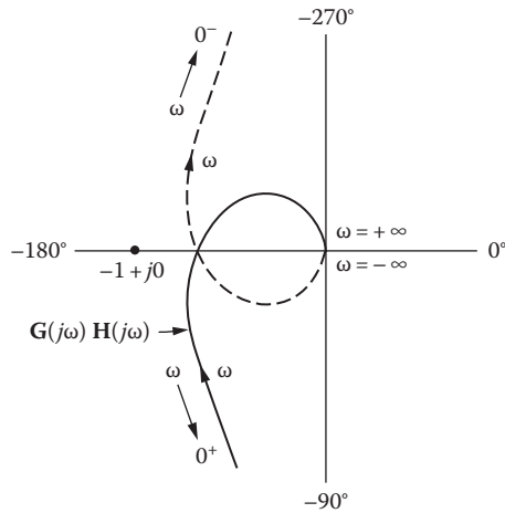
FIGURE 11.25 A plot of the transfer function G(j\omega)H(j\omega) for Equation 11.57.
