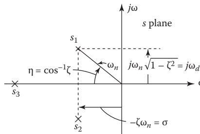
FIGURE 7.3 Location of complex-conjugate poles in the s plane.
