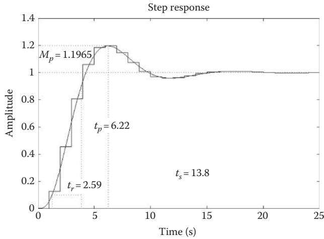
FIGURE 19.12 MATLAB® step response of DIG (PCT) versus DIR technique for T = 1.0 s.
