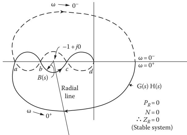
FIGURE 11.30 The complete polar plot of Equation 11.63.
