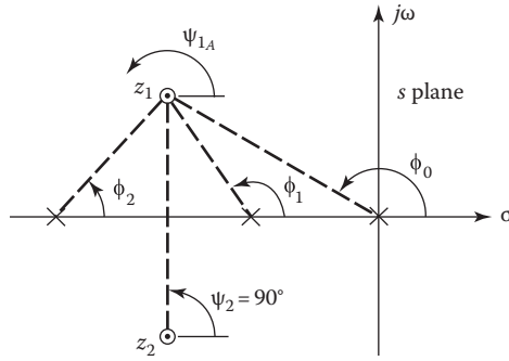
FIGURE 10.13 Angle condition in the vicinity of a complex zero.
