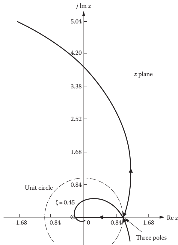
FIGURE 18.21 Root locus for G_z(z) = K_z(z + 0.26395)(z + 3.6767)/(z - 1)(z - 0.99005)(z - 0.95123) , where T = 0.001 s. (From Houpis, C.H. and Lamont, G.B., Digital Control Systems, Theory, Hardware, Software , 2nd edn., McGraw-Hill, New York, 1992. With permission.)
