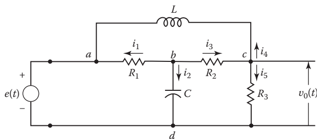
FIGURE 5.4 Multi-node network.
