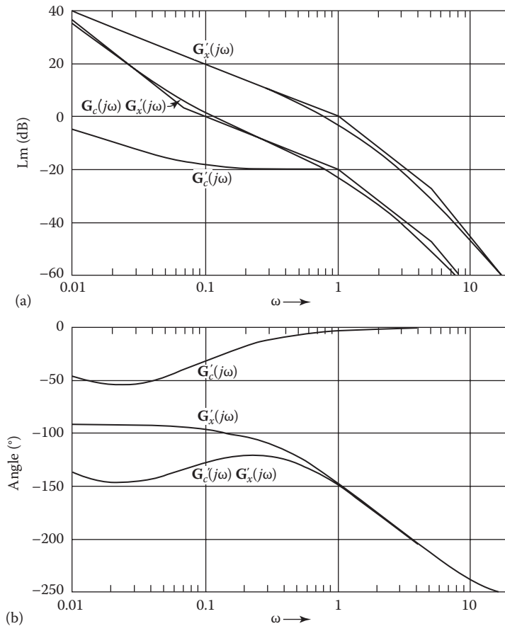
FIGURE 14.7 (a) Lm and (b) phase-angle diagrams for G'_x(j\omega) = \frac{1}{j\omega(1+j\omega)(1+j0.2\omega)} and G'_c(j\omega)G'_x(j\omega) = \frac{1+j14\omega}{j\omega(1+j\omega)(1+j0.2\omega)(1+j140\omega)} .
