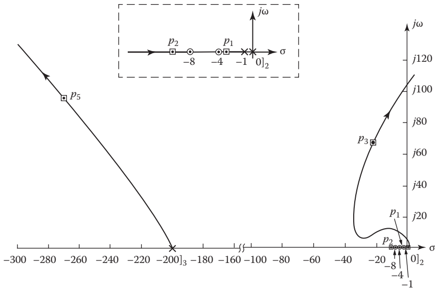
FIGURE 15.13 Sketch of root locus for Equation 15.34. Not to scale.
