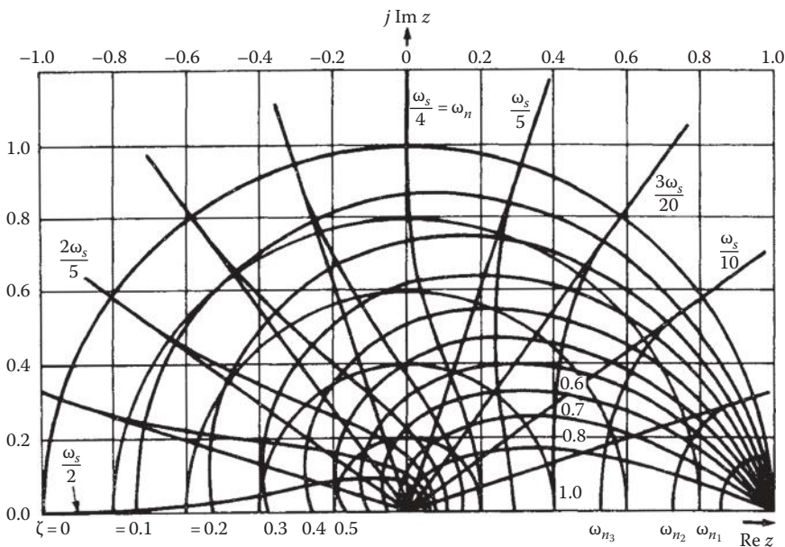
FIGURE 18.8 Plots of loci of constant \zeta and loci of constant \omega_n . (From Houpis, C.H. and Lamont, G.B., Digital Control Systems, Theory, Hardware, Software , 2nd edn., McGraw-Hill, New York, 1992. With permission.)
