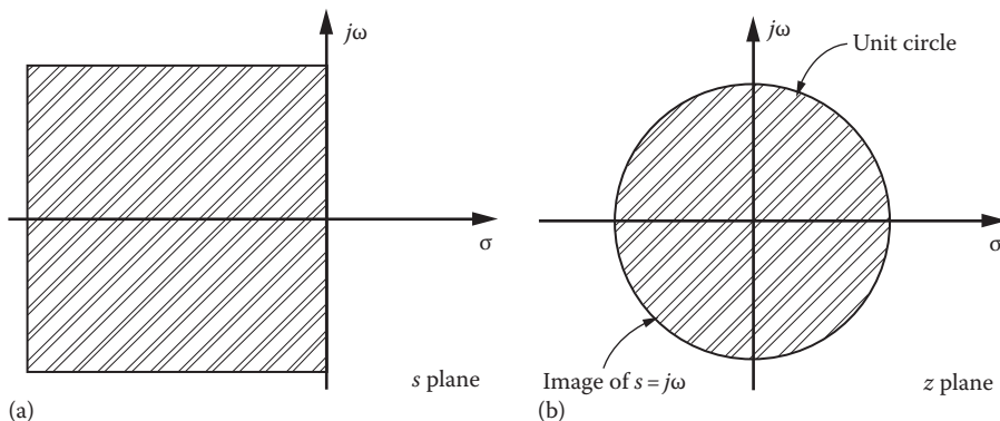
FIGURE 18.10 The mapping of the s plane into the z plane by means of z = e^{Ts} . (From Houpsis, C.H. and Lamont, G.B., Digital Control Systems, Theory, Hardware, Software , 2nd edn., McGraw-Hill, New York, 1992. With permission.)
