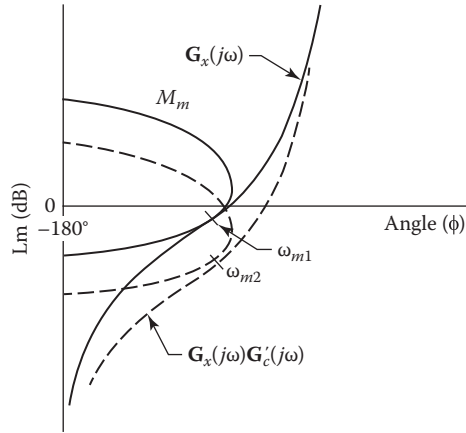
FIGURE 14.6 Original and lag-compensated Nichols plots.
