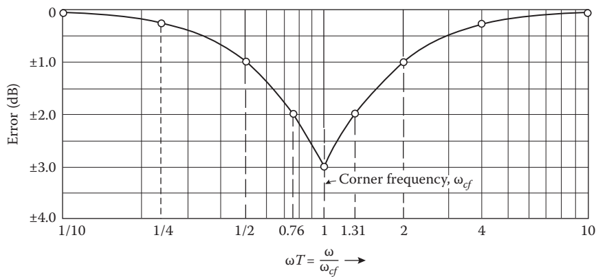
FIGURE 11.3 \text{Lm} correction for (1 + j\omega T)^{\pm 1} .
