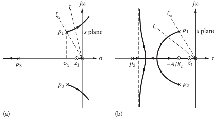
FIGURE 13.38 Root locus for the longitudinal motion of an aircraft: (a) uncompensated and (b) compensated (rate feedback).
