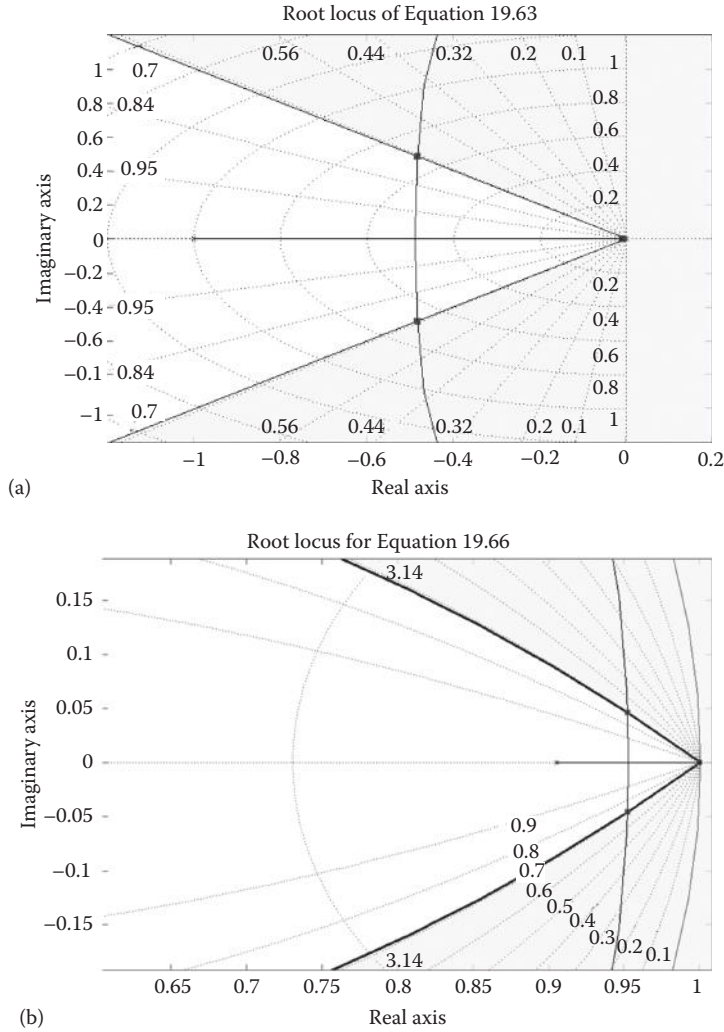
FIGURE 19.18 Root locus of (a) Equation 19.63 and (b) Equation 19.66.
