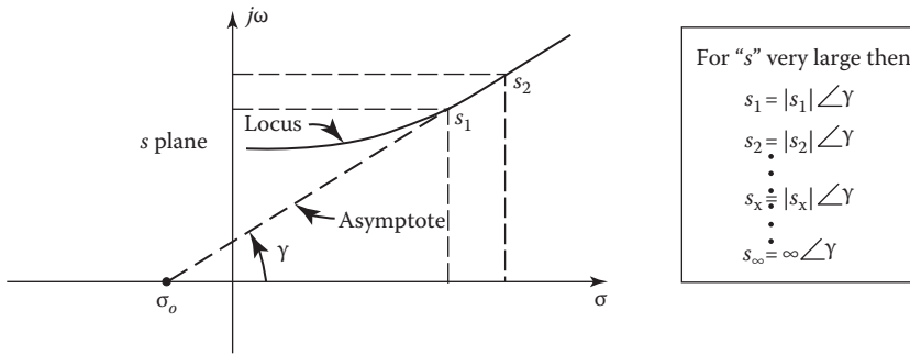
FIGURE 10.10 Asymptotic condition for large values of s .
