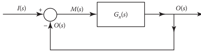
FIGURE 13.28 Transforming non-Type 0 control element to Type 0.
