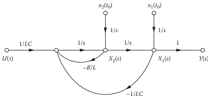
FIGURE 8.29 State diagram for Example 8.6.
