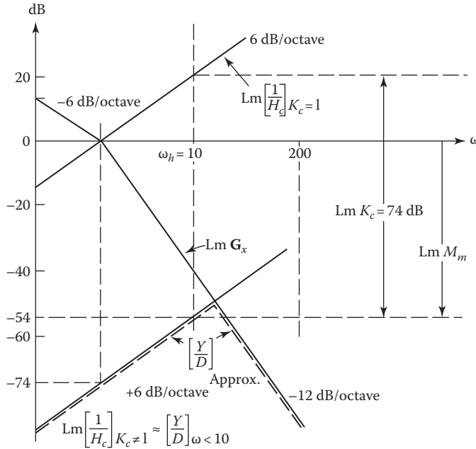
FIGURE 15.9 Lm plots of Example 15.2.
