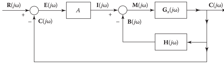
FIGURE 14.20 Block diagram for feedback compensation.
