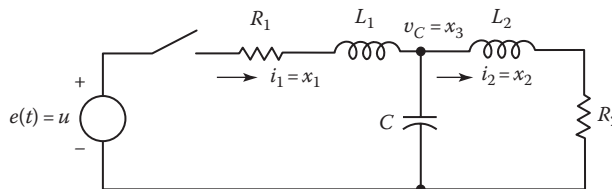
FIGURE 5.6 An electric circuit.
