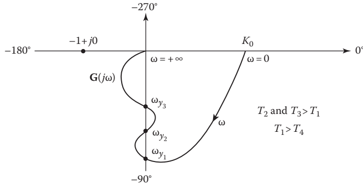
FIGURE 11.15 Polar plot for a more complex Type 0 transfer function (Equation 11.35).
