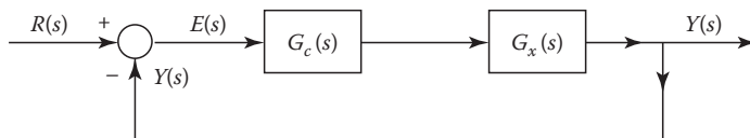
FIGURE 15.4 A cascade-compensated control system.
