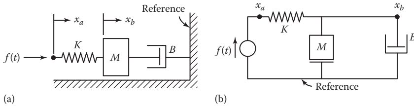
FIGURE 5.11 (a) Simple mass–spring–damper mechanical system; (b) corresponding mechanical network.
