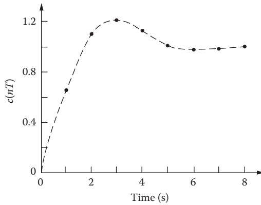
FIGURE 18.12 Plot of c(nT) for Equation 18.50.
