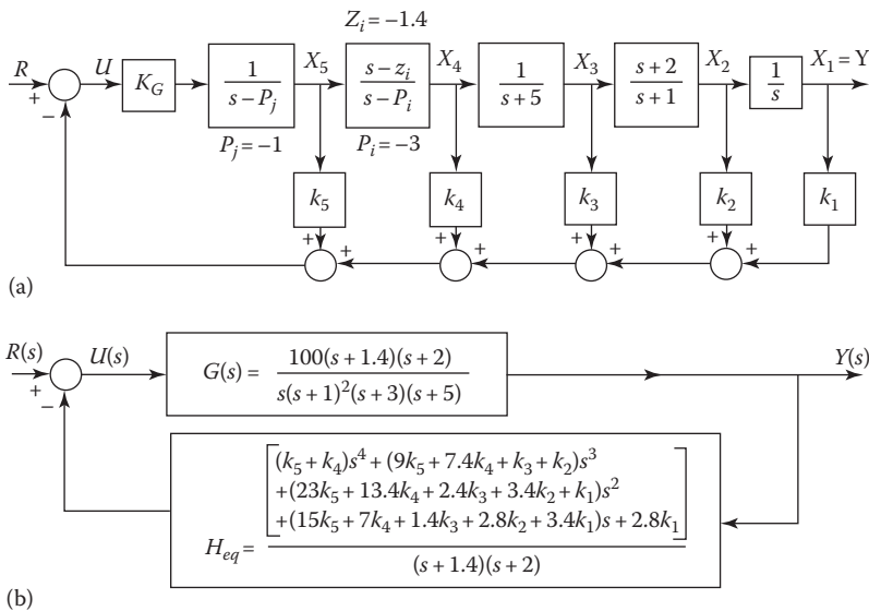
FIGURE 16.19 State-feedback diagram for Design Example 3.
