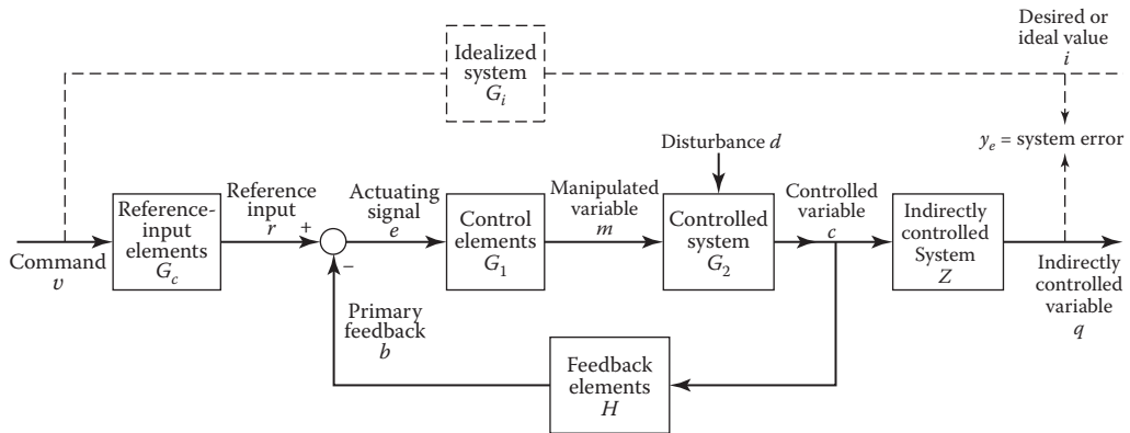
FIGURE 8.7 Block diagram of feedback control system containing all basic elements.
