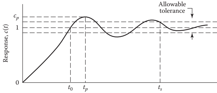
FIGURE 6.9 Typical underdamped response to a step input.
