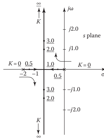
FIGURE 10.2 Plot of all roots of the characteristic equation s^2 + 2s + K = 0 for 0 \leq K < \infty . Values of K are underlined.
