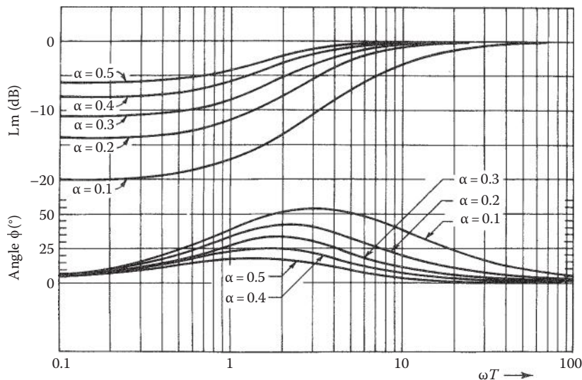
FIGURE 14.10 Lm and phase-angle diagram for lead compensator G'_c(j\omega) = \alpha \frac{1 + j\omega T}{1 + j\omega\alpha T} .
