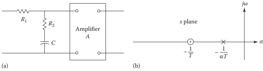
FIGURE 13.9 (a) Integral or lag compensator; (b) pole and zero location.
