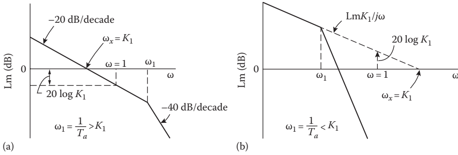
FIGURE 11.10 Lm plot for G(j\omega) = K_1/j\omega(1 + j\omega T_a) . The Lm plot when (a) \omega_1 > K_1 and (b) \omega_1 < K_1 .
