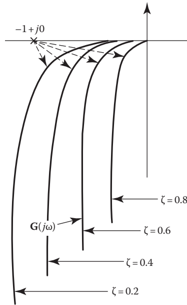
FIGURE 12.7 Polar plots of G(j\omega) for different damping ratios for the system shown in Figure 12.3.
