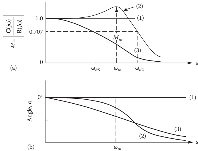
FIGURE 11.1 Frequency-response characteristics of C(j\omega)/R(j\omega) in rectangular coordinates. (a) Plot of 3 cases of the magnitude M and (b) plot of 3 cases of the phase angle \alpha .
