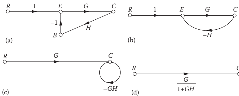
FIGURE 8.24 Successive reduction of the flow graph for the feedback system of Figure 8.6 (a–d).
