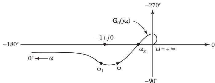
FIGURE 11.19 Polar plot for a typical Type 2 transfer function resulting in a stable system.
