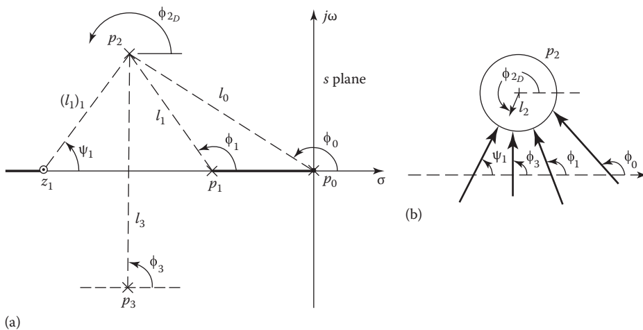
FIGURE 10.12 Angle condition in the vicinity of a complex pole. (a) Location of complex poles in the s -plane and (b) determination of the angle of departure.
