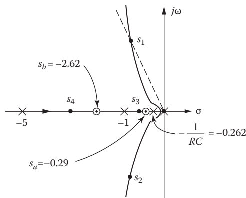
FIGURE 13.37 Root locus of Equation 13.68.
