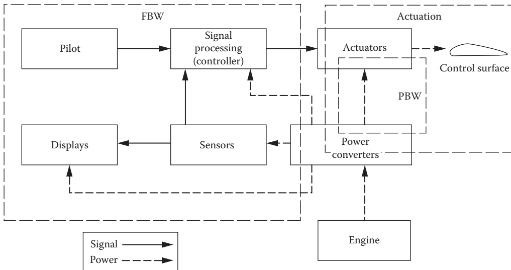
FIGURE 1.14 FBW and power-by-wire (PBW) control systems. (Courtesy of Control Systems Development Branch, Flight Dynamics Laboratory, Wright-Patterson AFB, OH.)
