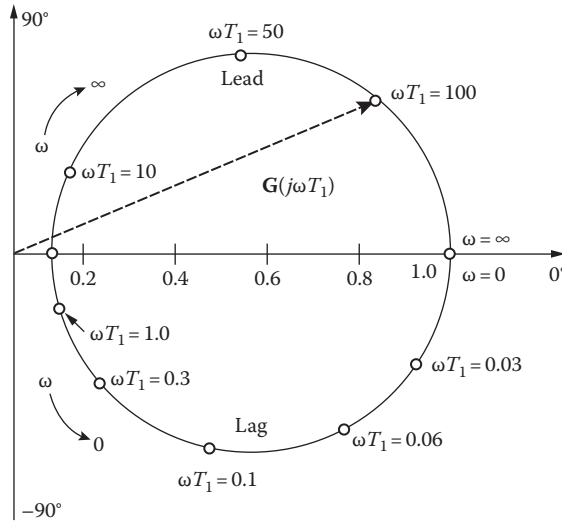
FIGURE 11.13 Polar plot of \mathbf{G}(j\omega T_1) = \frac{(1 + j\omega T_1)(1 + j0.2\omega T_1)}{(1 + j11.1\omega T_1)(1 + j0.0179\omega T_1)} ; T_2 = 0.2T_1, T_{12} = 10.0T_1 .
