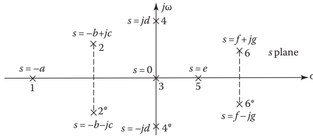
FIGURE 7.11 Location of poles in the s plane. (Numbers are used to identify the poles.)
