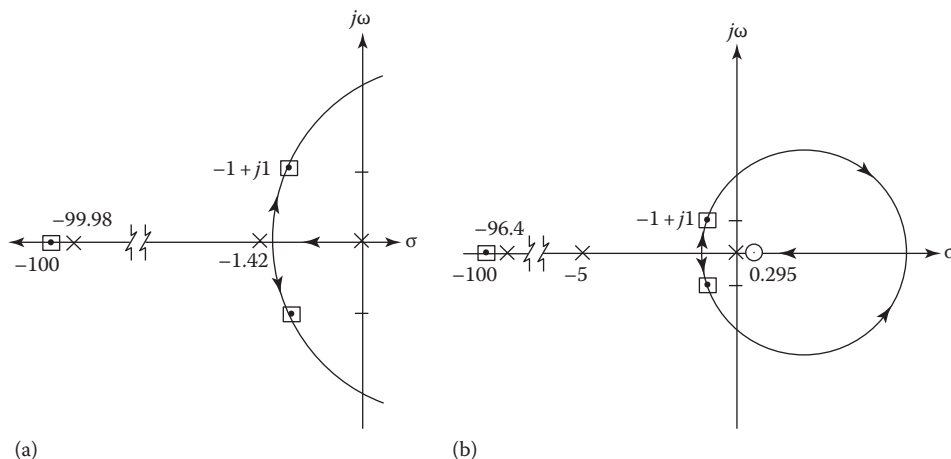
FIGURE 17.9 Root locus for (a) Figure 17.8c and (b) Figure 17.8d.
