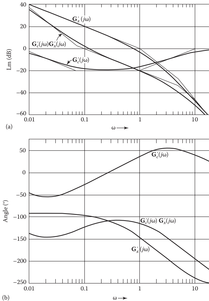
FIGURE 14.18 (a) Lm and (b) phase-angle diagrams of Equations 14.17 through 14.19 with T_1 = 14 .
