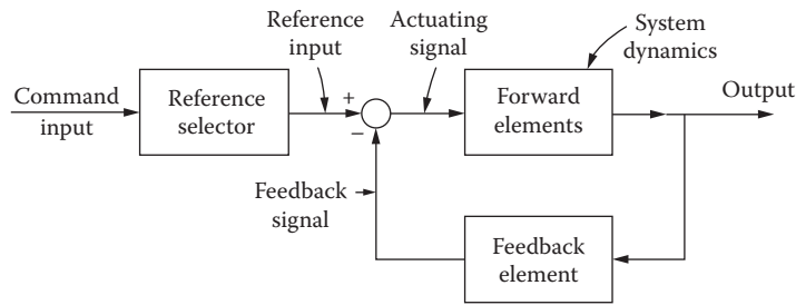
FIGURE 1.2 Functional block diagram of a closed-loop control system.
