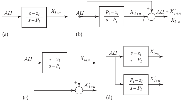
FIGURE 16.13 Cascade compensators: G_c(s) = (s - z_i)/(s - P_i) : (a) conventional, (b) feedforward form, (c) generating the state variable X'_{i+n} , and (d) mathematical model for (c).
