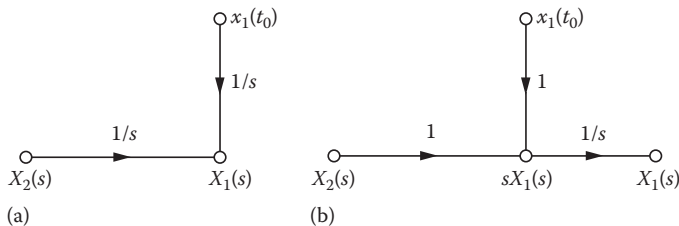
FIGURE 8.27 Two representations of the signal flow graph of Equation 8.59 are shown in (a) and (b).
