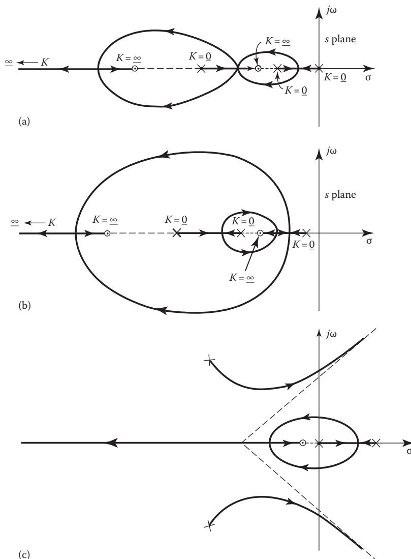
FIGURE 10.5 Various root-locus configurations:
