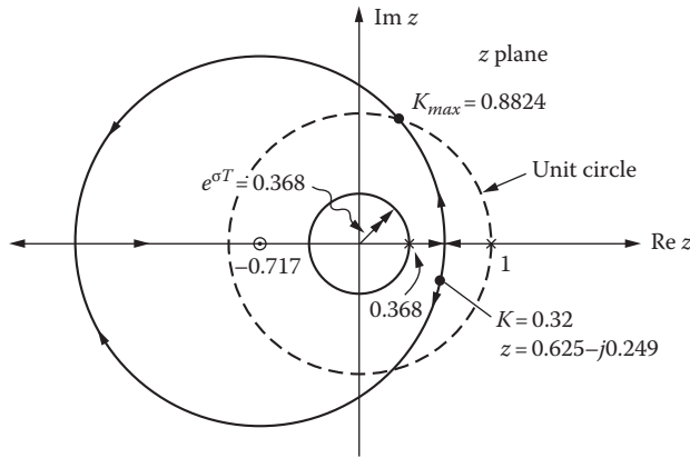
FIGURE 18.15 Root locus for the system of Figure 18.14.
