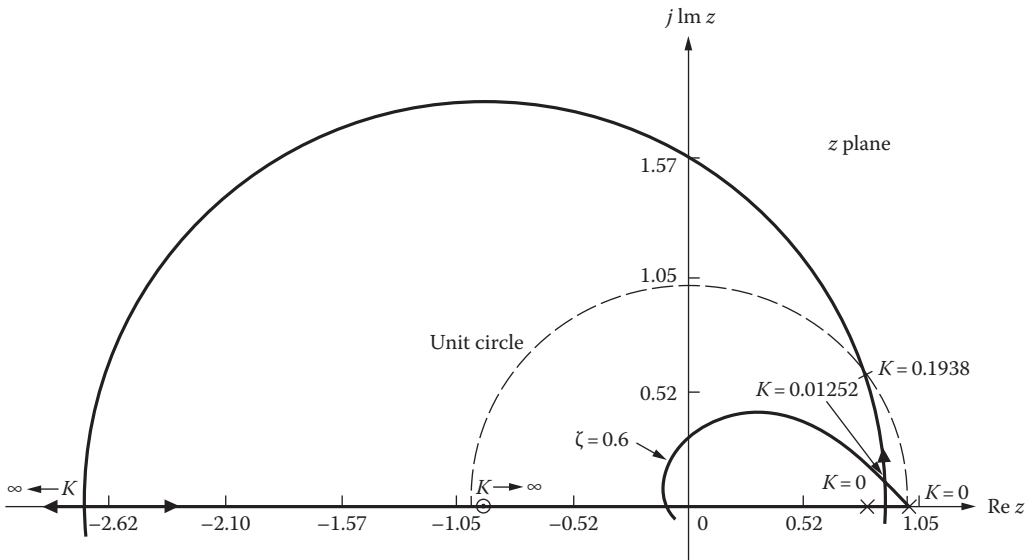
FIGURE 18.20 A root-locus sketch for Equation 18.106 where T = 0.1 s. (From Houppis, C.H. and Lamont, G.B., Digital Control Systems, Theory, Hardware, Software , 2nd edn., McGraw-Hill, New York, 1992. With permission.)
