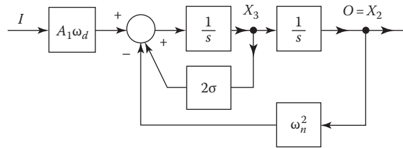
FIGURE 16.12 State-variable representation of O(s)/I(s) in Figure 16.11a.
