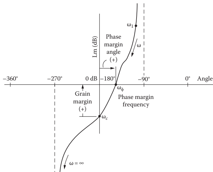
FIGURE 11.35 Example of a Lm-angle diagram for a m.p. open-loop transfer function.
