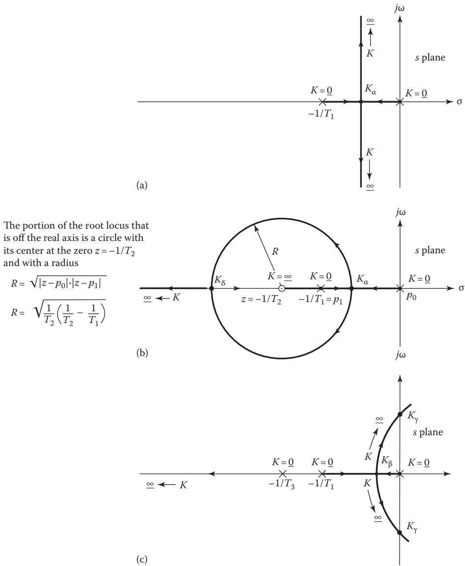
FIGURE 10.4 Various root-locus configurations for H(s) = 1 : (a) root locus of basic transfer function; (b) root locus with additional zero; (c) root locus with additional pole.
