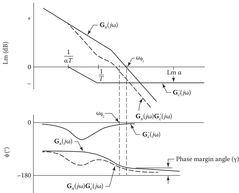
FIGURE 14.5 Original and lag-compensated Lm and phase-angle plots.
