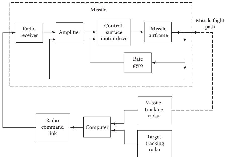
FIGURE 8.3 Block diagram of a generalized command guidance interceptor system.
