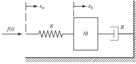
FIGURE 6.4 Simple mechanical system.
