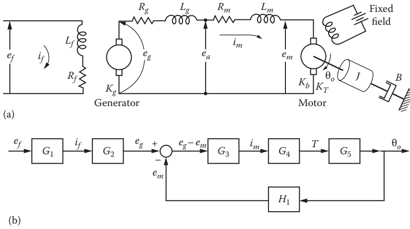
FIGURE 8.11 (a) Motor-generator control; (b) block diagram.
