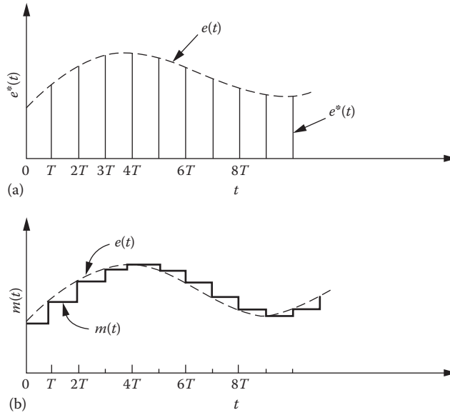
FIGURE 18.13 Input and output signals for a ZOH: (a) continuous input signal e(t) and the sampled signal e^*(t) ; (b) continuous signal e(t) and the piecewise-constant output m(t) of the ZOH.
