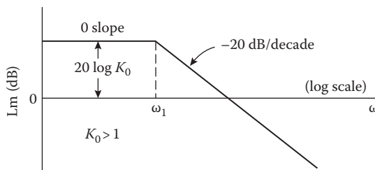
FIGURE 11.9 Lm plot for \mathbf{G}(j\omega) = K_0/(1 + j\omega T_a) .
