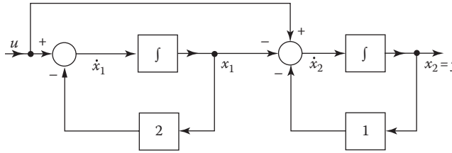
FIGURE 16.2 Simulation diagram for the system of Equation 16.17.
