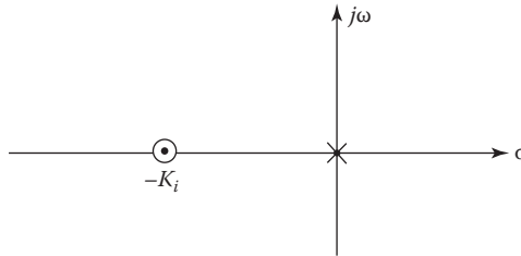
FIGURE 13.8 Location of the pole and zero of an ideal proportional PI compensator.
