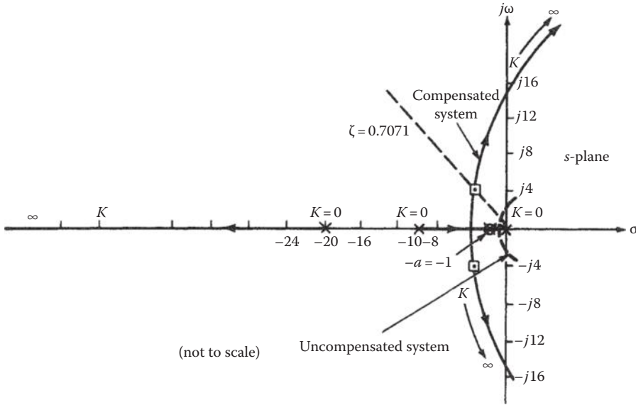
FIGURE 19.15 Root locus of a compensated system: D_c(s)G_{pc}(s) = -1 .
