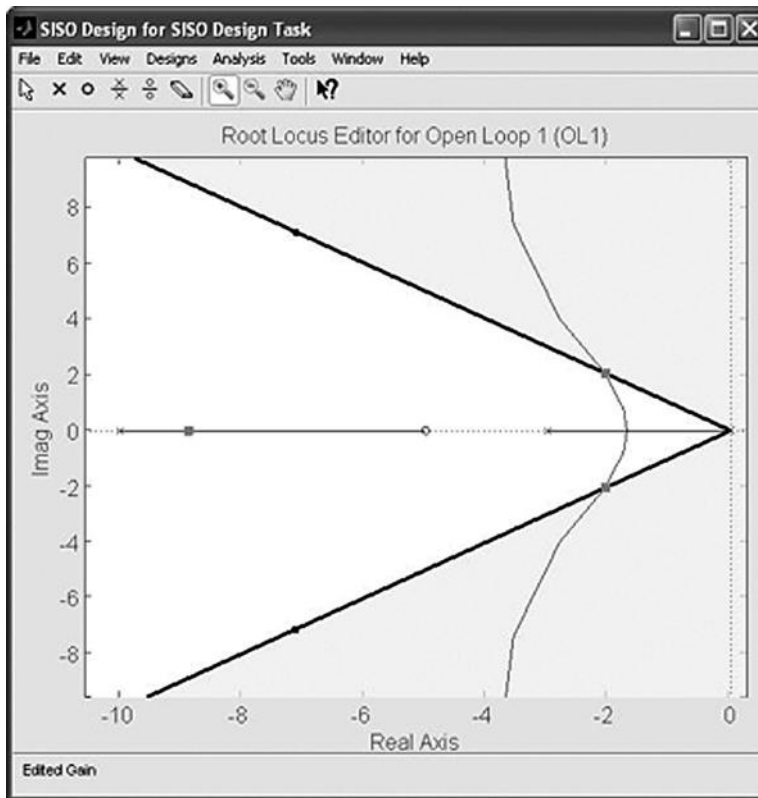
FIGURE C.4 Root locus SISOTOOL window.
