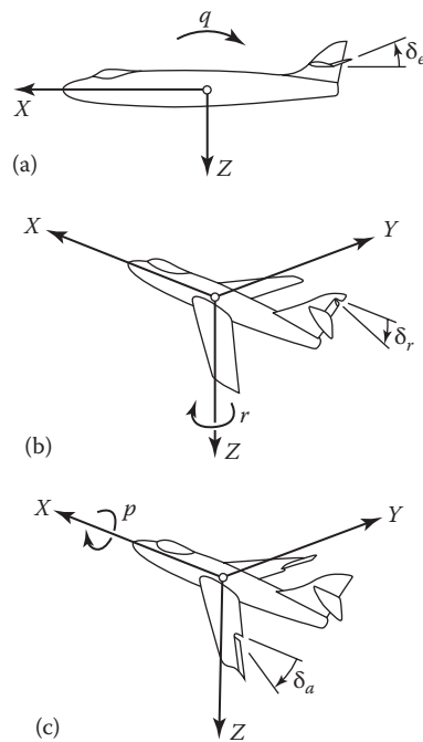
FIGURE 8.4 Airplane control surfaces: (a) elevator deflection produces pitching velocity q ; (b) rudder deflection produces yawing velocity r ; (c) aileron deflection produces rolling velocity p .
