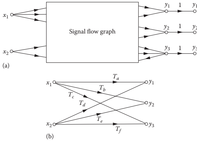
FIGURE 8.25 (a) An arbitrarily complex system and (b) its equivalent SFG.
