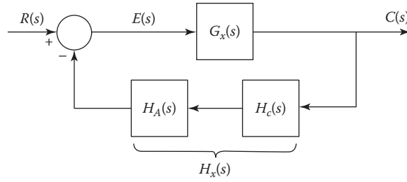
FIGURE 19.24 PCT system approximation of the sampled-data control system of Figure 19.22.
