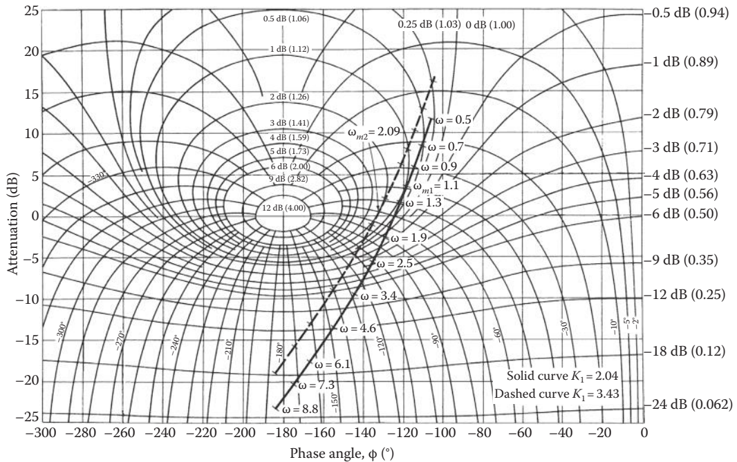
FIGURE 12.23 Log magnitude–angle diagram for Equation 12.49.
