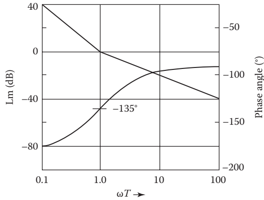
FIGURE 14.23 Lm and phase-angle diagram of \frac{1}{\mathbf{H}'(j\omega T)} = \frac{1+j\omega T}{(j\omega T)^2} .
