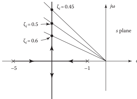
FIGURE 13.33 Poles of the inner loop for several values of \zeta_i .
