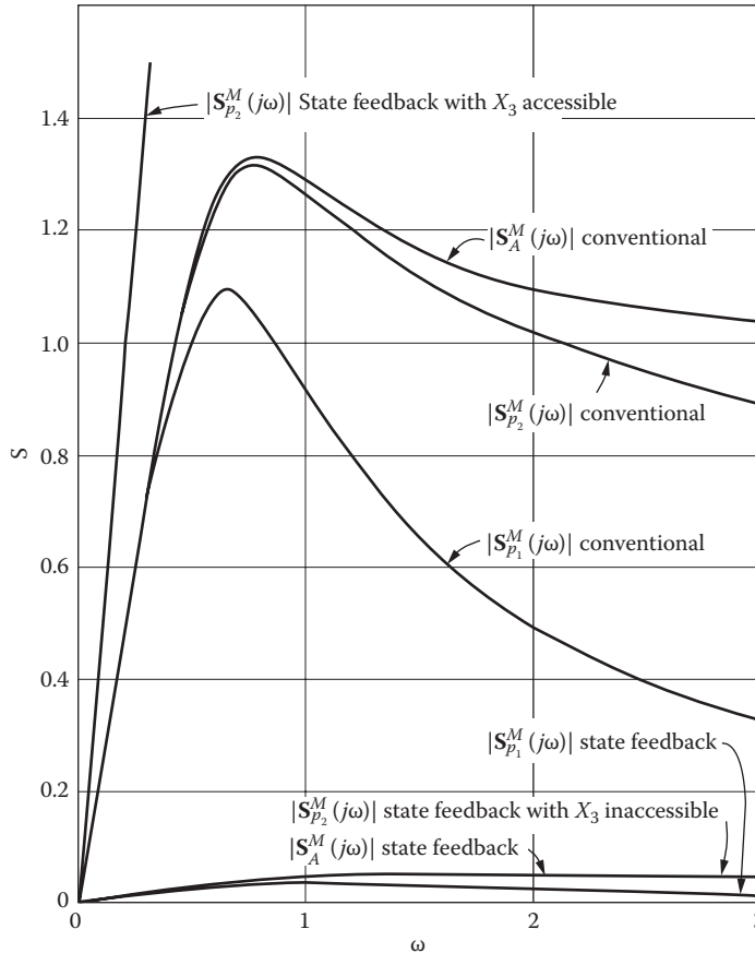
FIGURE 17.6 Sensitivity due to pole and gain variation.
