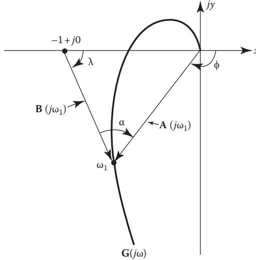
FIGURE 12.2 Polar plot of G(j\omega) for the control system of Figure 12.1.
