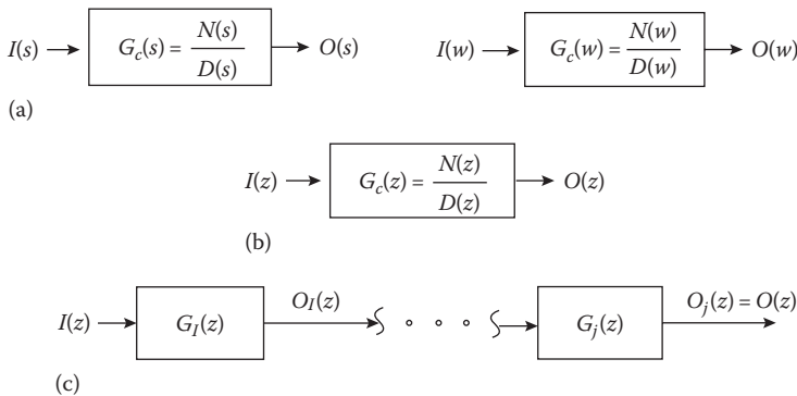
FIGURE 19.30 s - or w -domain to z -domain bilinear transformation: formulation for implementation of the G_c(z) controller. (a) The design compensators, (b) z domain compensator, (c) z domain j cascaded controllers.
