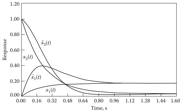
FIGURE 16.23 Plant and observer states, Equations 16.148 and 16.150.
