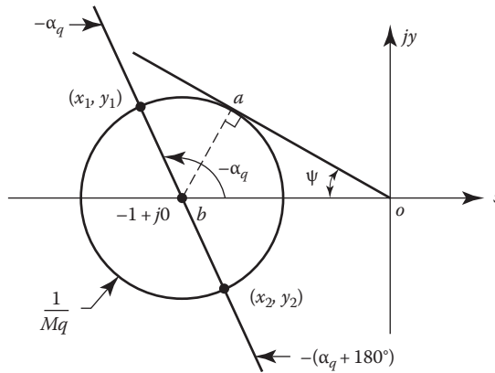
FIGURE 12.15 Contour for a particular magnitude \mathbf{R}(j\omega)/\mathbf{C}(j\omega) = 1/M_q .
