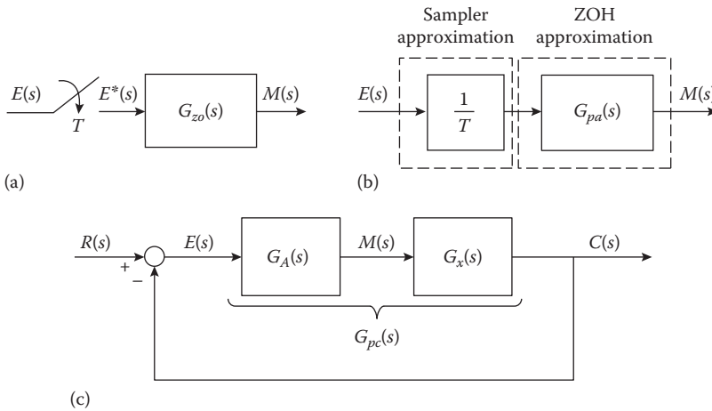
FIGURE 19.9 (a) Sampler and ZOH. (b) Approximations of the sampler and ZOH, (c) The approximate continuous-time control system equivalent of Figure 19.8.
