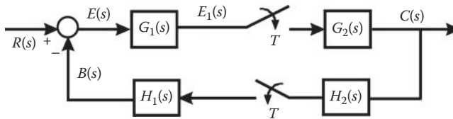
FIGURE 18.9 A nonunity-feedback S-D control system. (From Houpis, C.H. and Lamont, G.B., Digital Control Systems, Theory, Hardware, Software , 2nd edn., McGraw-Hill, New York, 1992. With permission.)
