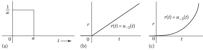
FIGURE 6.1 Singularity functions: (a) an impulse function as a approaches 0; (b) ramp function, u_{-2}(t) ; (c) parabolic function, u_{-3}(t) .
