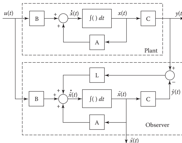
FIGURE 16.21 Plant with inaccessible states and an observer that generates estimates of the states.
