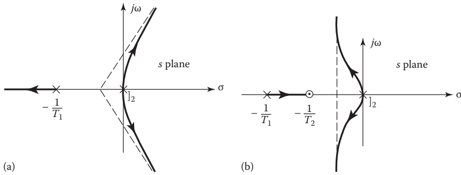
FIGURE 13.15 Root locus for (a) G_x(s) = K/s^2(s + 1/T_1) ; (b) G(s) = K(s + 1/T_2)/s^2(s + 1/T_1) .
