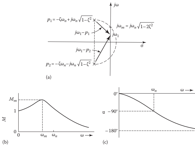
FIGURE 7.10 (a) Pole-zero diagram, \zeta < 0.707 ; (b) magnitude of frequency response; (c) angle of frequency response.
