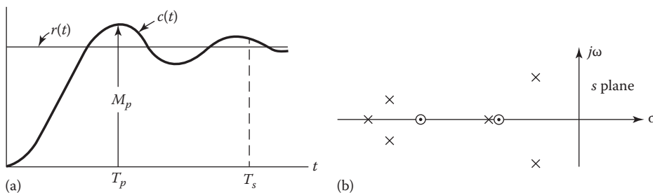
FIGURE 13.2 Transient response to a step input with dominant complex poles. (a) The time response plots due to a unit step input and (b) pole-zero pattern of C(s)/R(s) for the desired response.
