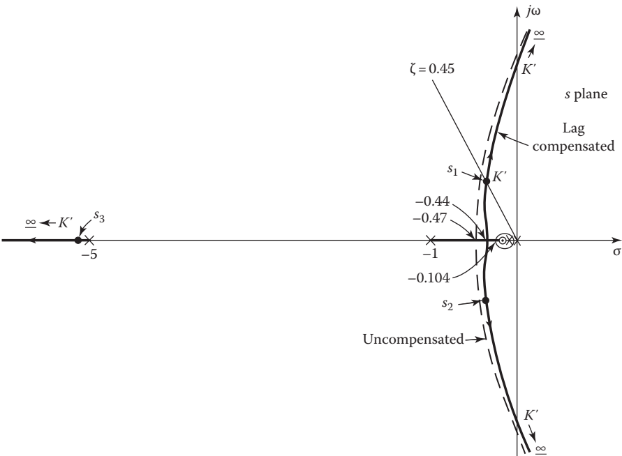
FIGURE 13.11 Root locus of G(s) = K'(s + 0.05)/s(s + 1)(s + 5)(s + 0.005) .
