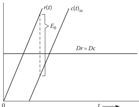
FIGURE 9.11 Steady-state response of a Type 1 system for Dr = \text{constant} .
