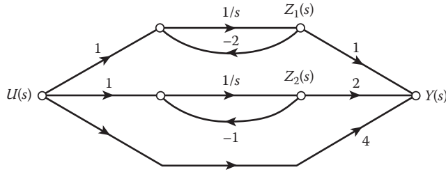
FIGURE 8.32 Simulation diagram for Example 8.8.
