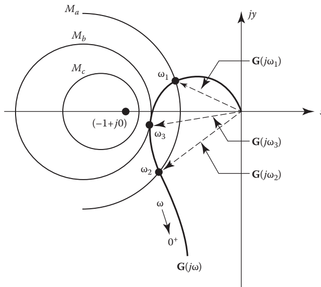
FIGURE 12.9 M contours and a \mathbf{G}(j\omega) plot.
