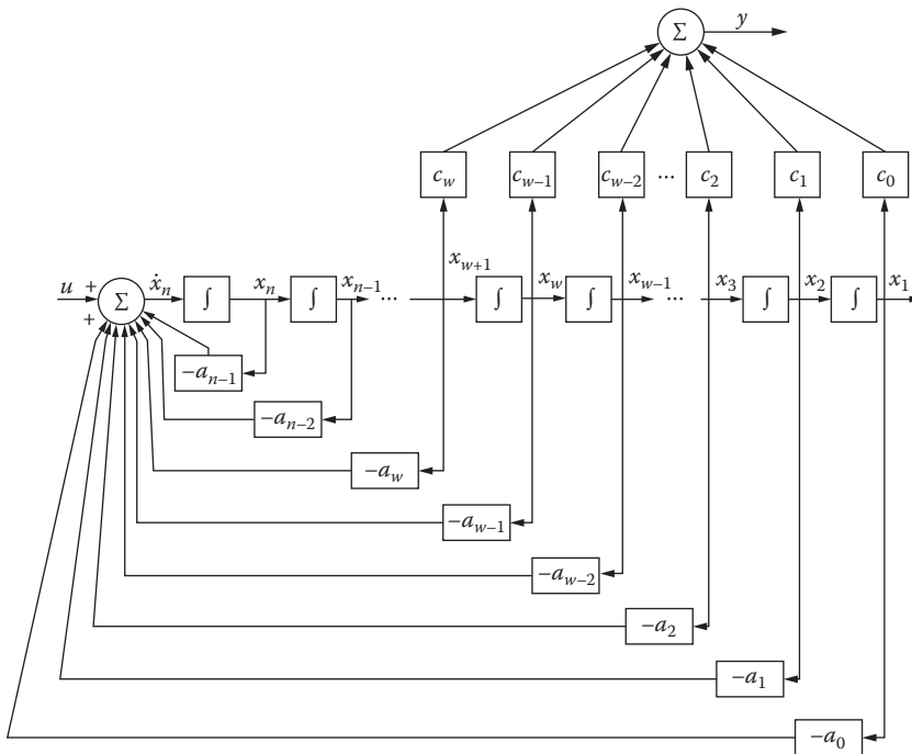
FIGURE 8.18 Simulation diagram representing the system of Equation 8.40 in terms of Equations 8.38 and 8.45.
