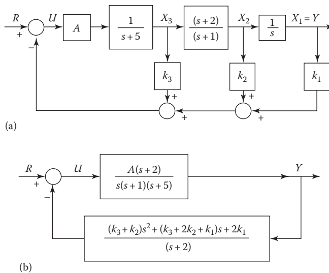
FIGURE 16.15 Closed-loop zero cancellation by state-variable feedback: (a) detailed block diagram and (b) H -equivalent reduction (where K_G = A ).
