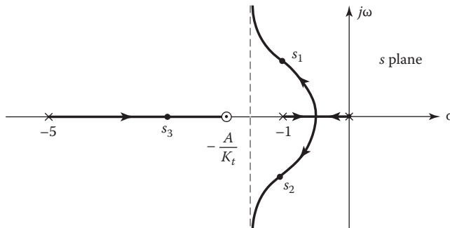
FIGURE 13.31 Root locus for Equation 13.60.
