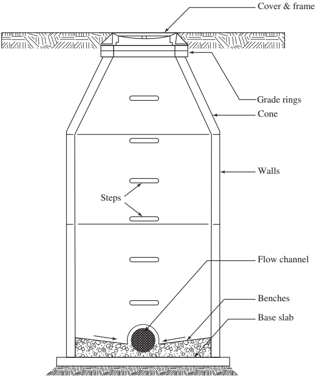
FIGURE 19-4 Manhole nomenclature.
