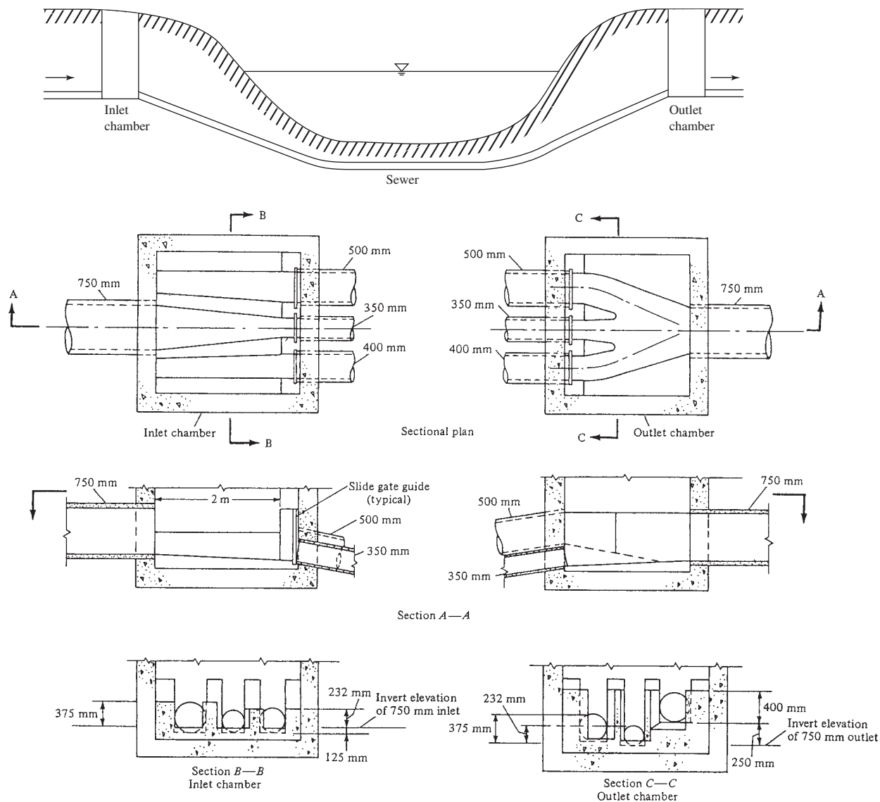
FIGURE 19-7 Inverted siphon with detailed views of inlet and outlet chambers. (Adapted from Metcalf & Eddy, 1981.)
