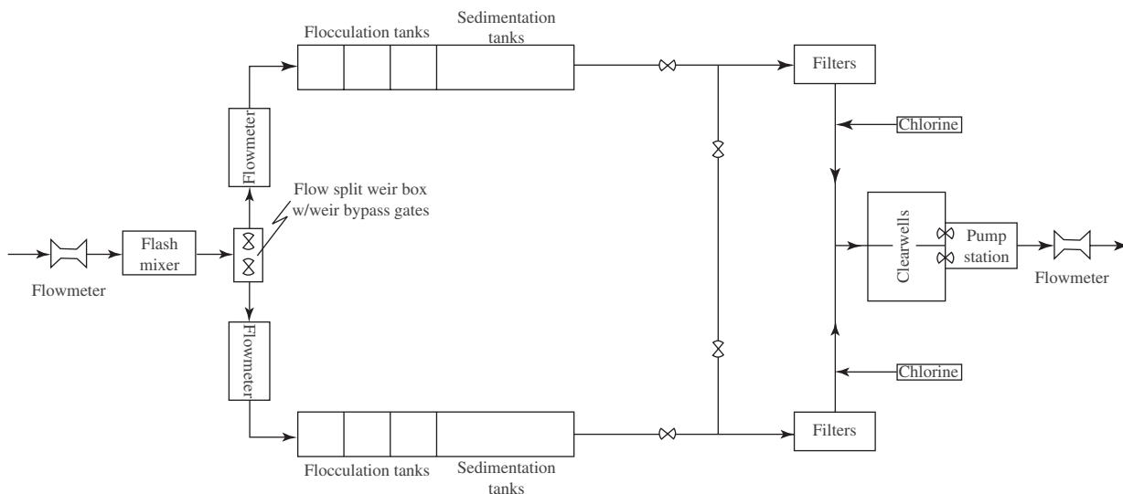
FIGURE 16-8 Process train scheme to improve treatment flexibility.
