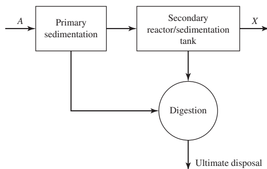
FIGURE P-27-7 Flowsheet for Doubtful WWTP.
